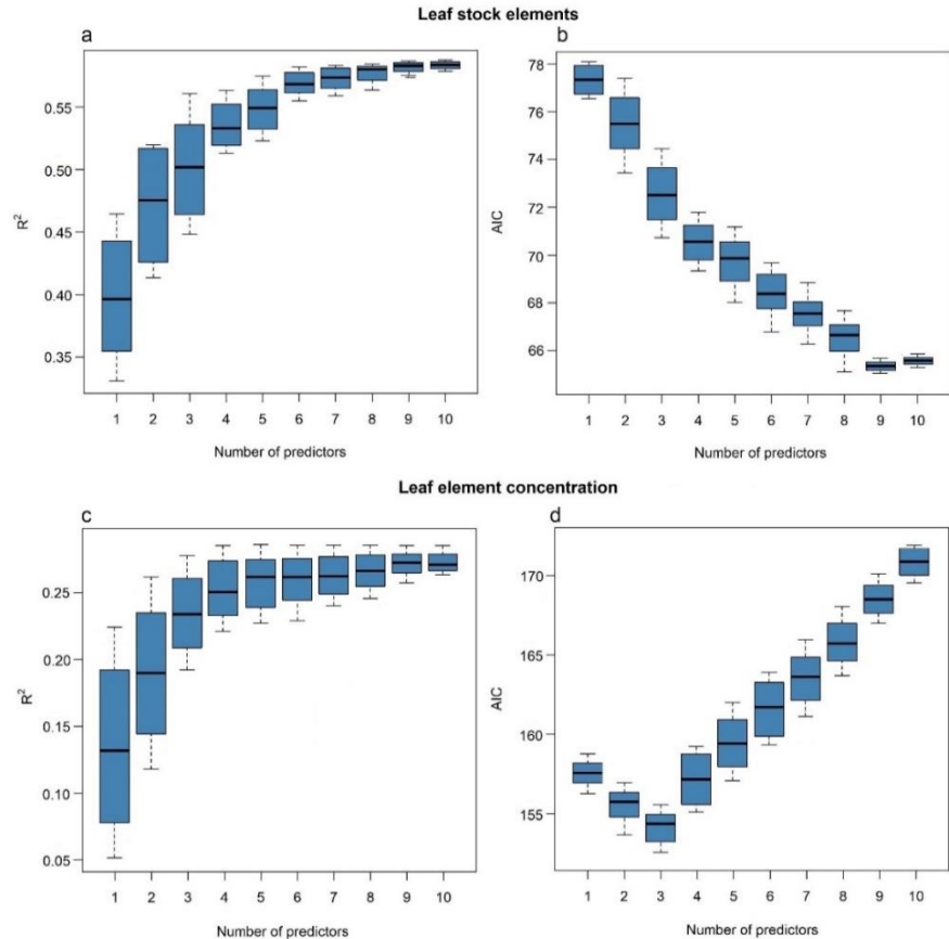
Figure 2: Forest biomass production (a, b) and productivity (c, d) predicted by leaf element stocks (a, b) and leaf element concentration (c, d). Results demonstrated by the performance (AIC and R^2 ) of the most robust subsets of models ( \Delta AIC < 4 ).
