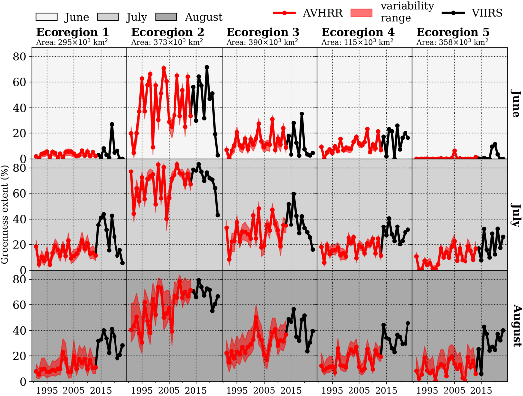
Figure 2. Development of green-vegetation greenness extent between 1991 and 2023 for June (upper row), July (middle row) and August (bottom row) across ecoregions based on AVHRR (red) and VIIRS (black). The AVHRR variability range is shaded in red, given the monthly minimum and maximum number of observations within VIIRS period ( 2014–2023 2014–2023 ).
