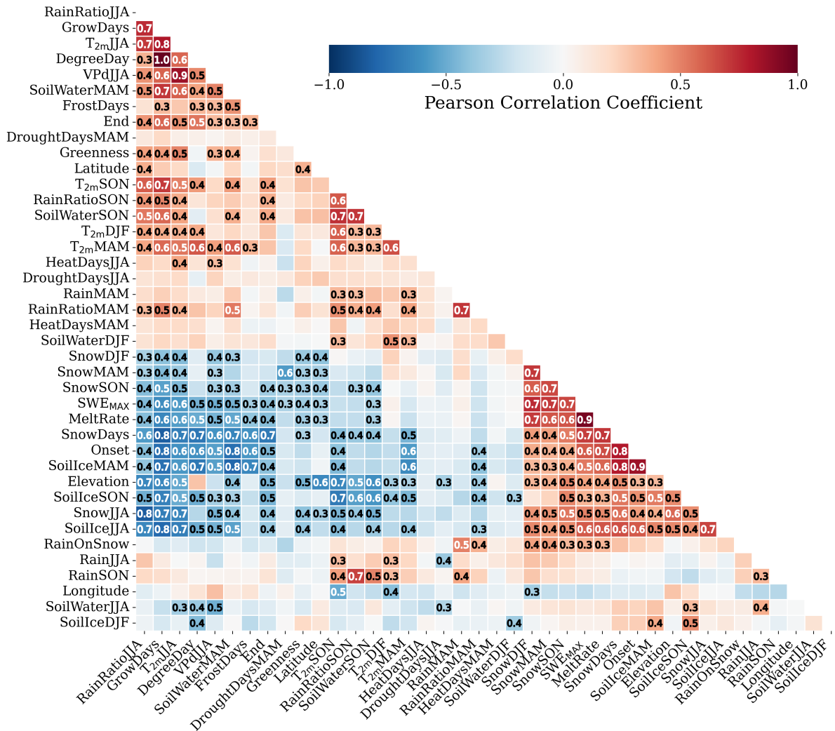
Figure 3. Correlation matrix for the bio-climatic indicators in ecoregion 2, including Elevation, Longitude and Latitude. The correlation coefficient is colour-coded and the absolute value noted for absolute correlation coefficients higher than 0.3. The abbreviations of the bio-climatic indicators are described in Section 3.2 and in Table 1.
