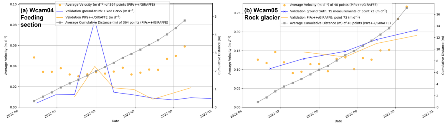
Figure 8: Graphs showing weekly velocities and cumulative distances of tracked points measured using the PIPs++/GIRAFFE workflow, including validation against ground truth data. a) Feeding section (Wcam04) and b) Rock glacier (Wcam05) during summer 2022, derived from time-lapse imagery. Note that the data from October 26 is excluded from a) due to foggy conditions and was interpolated by the model. Validation points, marked in a solid blue line, represent measurements from a permanent GNSS antenna installed on a large boulder in the upper feeding area (a) and one theodolite point on the rock glacier (b). The corresponding tracked points by PIPs++/GIRAFFE is displayed in a solid orange line.
