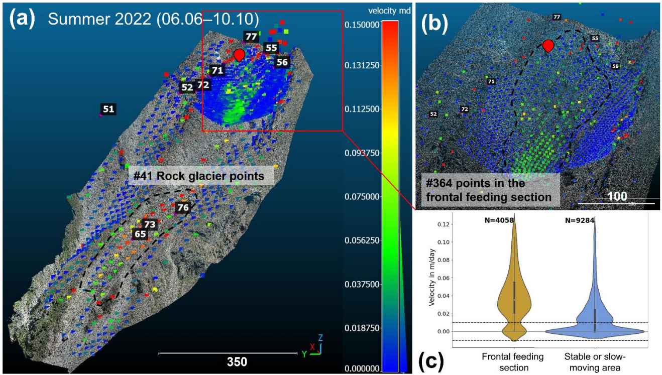
Figure 5: a) Velocity results (in m d -1 ) over the entire summer period (127 days) for both the frontal feeding section (upper area, observed by Wcam04) and the rock glacier (lower area, observed by Wcam05), displayed on UAV point cloud data, including total station-measured points (black and white labels) and the permanent GNSS installation (marked with a red location pin), b) close-up of the frontal feeding section (Wcam04), c) plot of the weekly velocity distribution for both the frontal feeding section and the surrounding stable or slow-moving areas (data from Wcam04), showing a clear noise level between \pm 0.007 m d -1 in both regions. Dotted lines indicate the moving areas in this study. Points in blue display areas moving less than about 0.02 m d -1 for the considered timeframe of 127 days.
