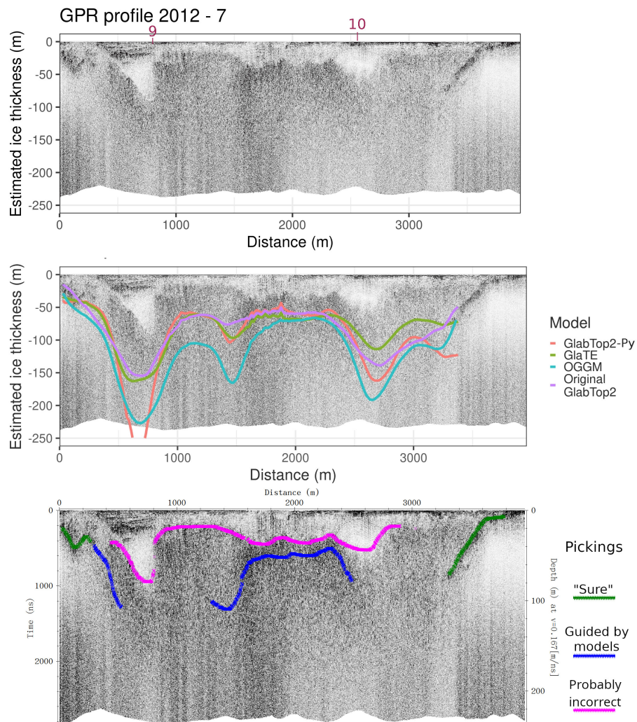
Figure 6. An example GPR section with the estimation from the four models overlaid: GlabTop2-Py in red, GlaTE in green, OGGM in blue, Original-GlabTop2 in purple. The manual selection of the ice-bedrock interface, which was possible by comparing the GPR profiles and the models, is displayed in different colours according to their reliability. Purple numbers indicate where this profile crosses other GPR profiles.
