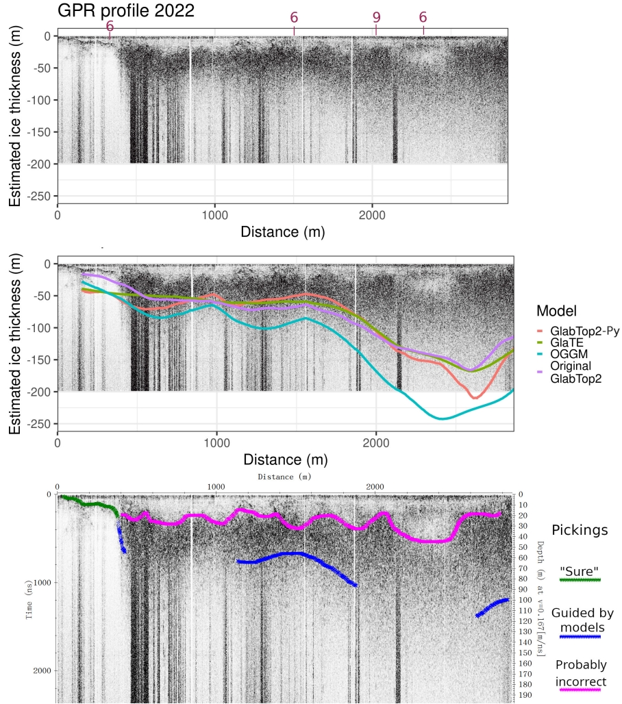
Figure A6. GPR section 2022. This GPR section was acquired with an antenna (40 MHz) different from that used for the previous sections shown. It also was ground-based and not helicopter-based. Notwithstanding the lower frequency and being ground-based, the GPR reflections were not particularly clearer, showing a physical limit of the technology in the presence of widespread englacial water or debris [Forte et al. , 2021]. The models did not perform well near the margin, with the exception of Original-Glabtop2, as observed also in the other GPR sections. However, probably the models offer a reasonable estimate of the bedrock interface in all the left-central part of the image. The right part seems more problematic because the GPR signal is completely lost, however, its greater depth is supported by the GPR signal texture: compare e.g. the image at 100 m depth at Distance = 1000 m and = 2500 m. At distance = 2500 m, the image shows a granular texture similar to where there is ice and englacial water, while at Distance = 1000 m the texture is transparent. Similar considerations were used to interpret the GPR sections by Forte et al. [2021].
