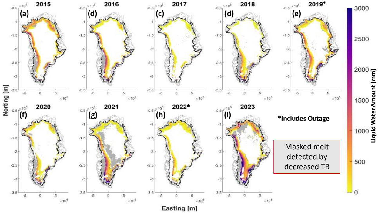
Figure 8: Total annual sum of SMAP daily LWA for 2015 - 2023. The black solid line represents GrIS edges, and the grey color masks inside the ice sheet indicate melt detections by decreased TB, which were not quantified.
