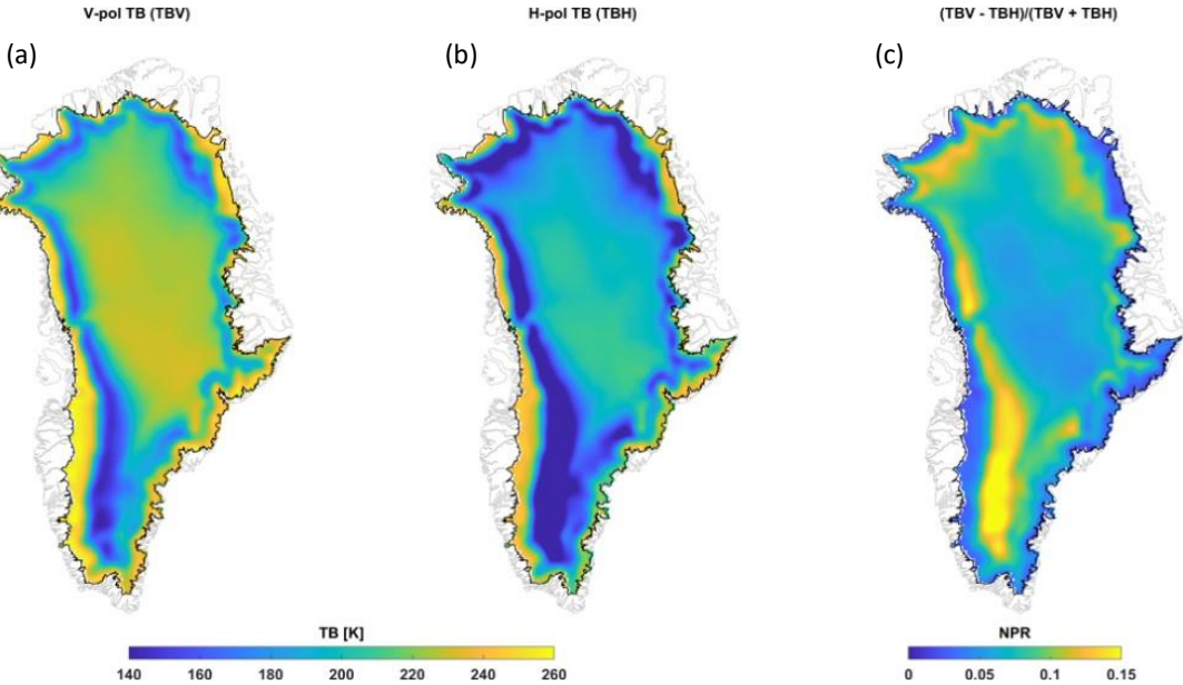
193 194 Figure 1: L-band radiometric response of GrIS during frozen season. Vertically polarized TB (a), horizontally polarized TB (b) 195 averaged over Jan 1 – Apr 7 th , 2015 – 2023, and their normalized polarization difference (c).
