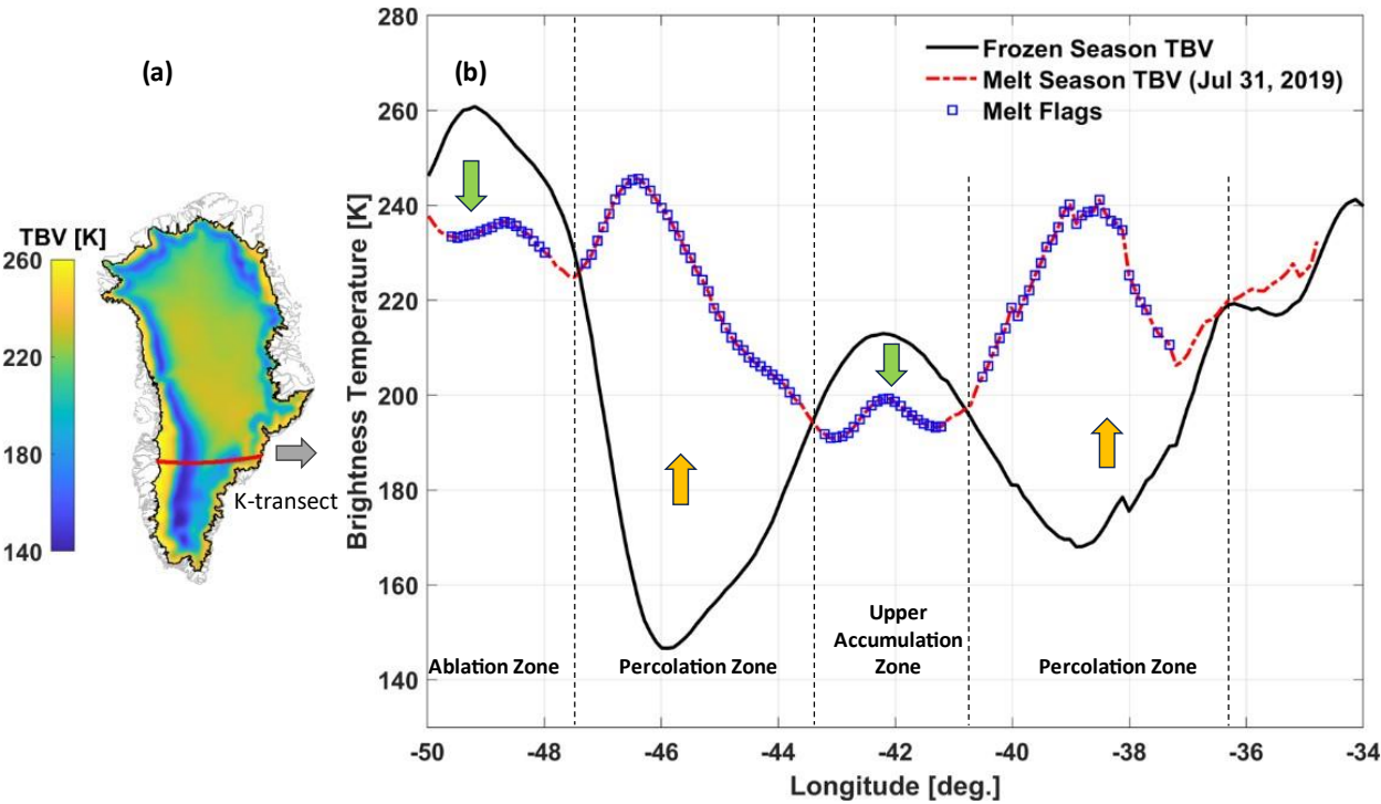
212 Figure 2: Radiometric response of L- band TB during frozen and melt season. The location of K-transect is highlighted by red line 213 over the mean frozen season TBV map (a). Corresponding TBs across the transect are shown in (b): the black line represents the 214 mean V-pol TB during the frozen season (Jan 1 – Apr 7th of the same year). The red dash-dotted line indicates TB responses on a 215 sample melt day (Jul 31, 2019). The blue square symbols on the red dashed-dotted line depict melt flags (melt detections). 216 Approximate location of ablation, percolation, and upper accumulation zones are depicted along the K-transect for reference.
