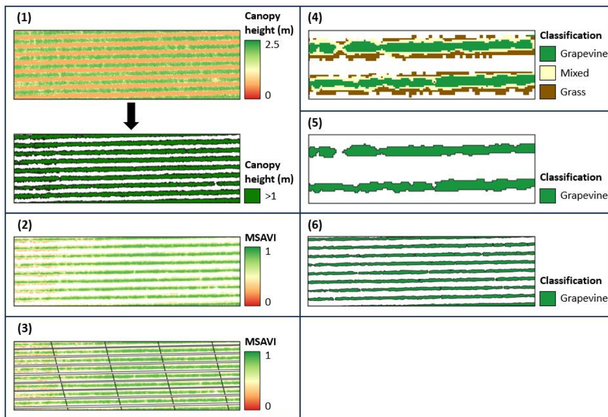
Figure 2 – Process of segmenting grapevine pixels from inter-row pixels to generate a pure grapevine mask. (1) First raw distinction between rows (>1 m) and inter-rows (<1 m) using the canopy height derived from the LiDAR data; (2) Application of the raw grapevine mask obtained in (1) on the Modified Soil Adjusted Vegetation Index (MSAVI) raster; (3) Subdivision of the new MSAVI raster obtained in (2) into smaller areas (rectangles of 10 m x 1.5 m); (4) Application of k-means algorithm in each rectangle. The number of clusters was set to three (pure grapevine, mixed, pure grass); (5) Selection of pure grapevine pixels, based on the clustering obtained with the k-means algorithm; (6) Creation of a unique mask to extract pure grapevine pixels from each raster of vegetation indices.
