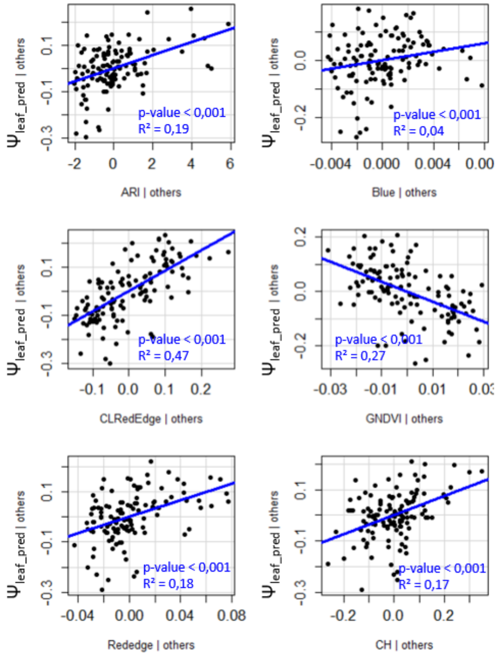
Figure S6 – Partial regression plots of each predictor variable on the prediction of \Psi_{\text{leaf}} , for the model 2 \Psi_{\text{leaf\_pred}} = -0.77 + 0.81 \cdot \text{CLRedEdge} + 6.78 \cdot \text{Blue} + 0.38 \cdot \text{CH} + 1.49 \cdot \text{RedEdge} + 0.02 \cdot \text{ARI} - 3.32 \cdot \text{GNDVI} (multispectral and LiDAR data). The p-value < 0.001 signifies that the slope of the linear regression (blue line) is significantly different from 0.
