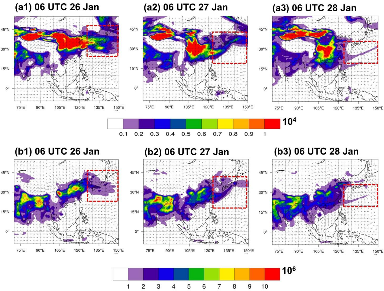
996 Figure S4: MERRA2 dust (a1-a3) and BC (b1-b3) mass column during 06 UTC (a1, b1) 26 January, (a2, 997 b2) 27 January and (a3, b3) 28 January 2023.
