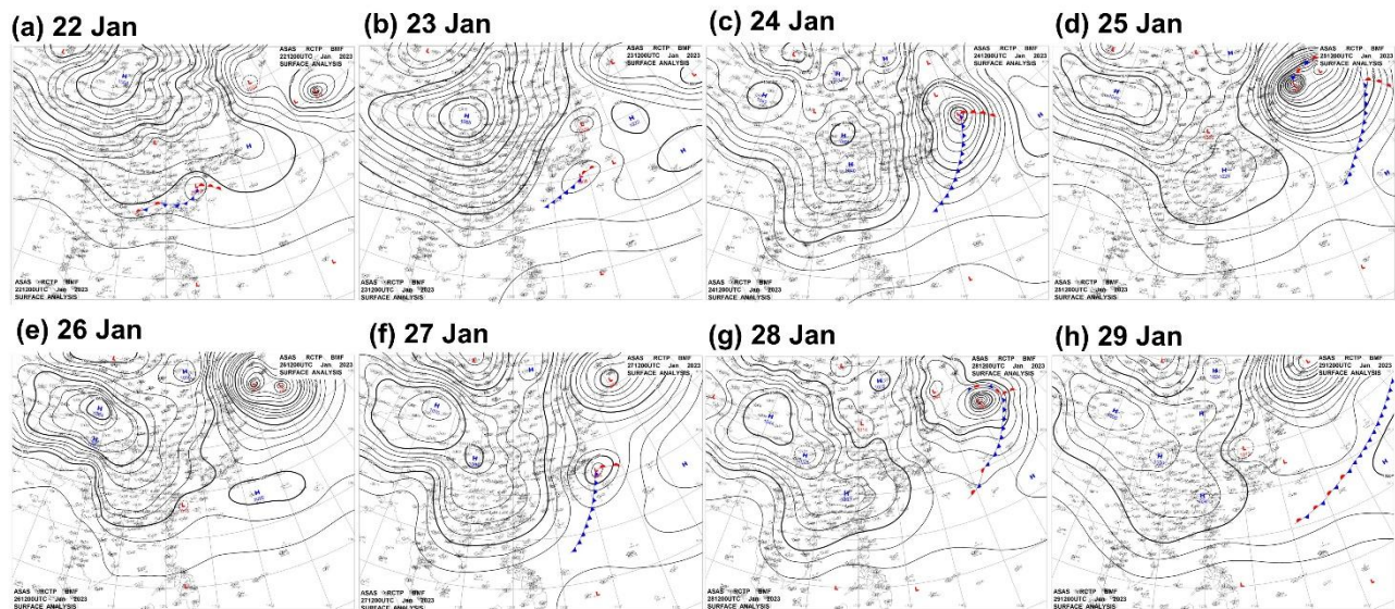
Figure S2: Surface weather maps for the weather pattern obtained by Taiwan Central Weather Bureau ( https://www.cwa.gov.tw/ ).
