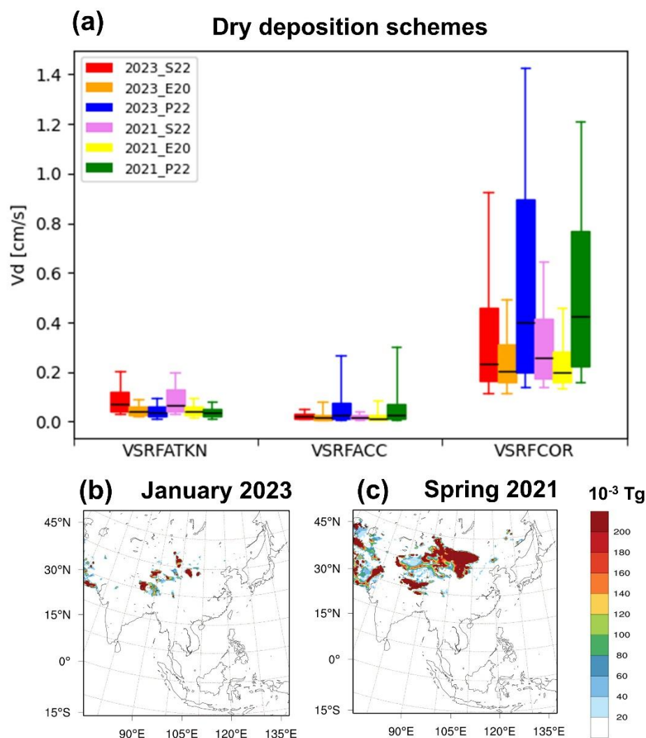
865 866 Figure 7: (a) 10-days (2023) and 40-days (2021) averaged dry V_d predicted by CMAQ for the Aitken, 867 accumulation, and coarse particle modes using the 2023_S22 (red), 2023_E20 (orange), 2023_P22 (blue), 868 2021_S22 (violet), 2021_E20 (yellow) and 2021_P22 (green) particle dry deposition schemes. The 869 variability illustrated by the boxes and whiskers corresponds to spatial variability in annually averaged 870 values throughout the CMAQ domain. The simulated total dust emission from CMAQ_Dust_E20 in (b) 871 January 2023 and (c) Spring 2021.
