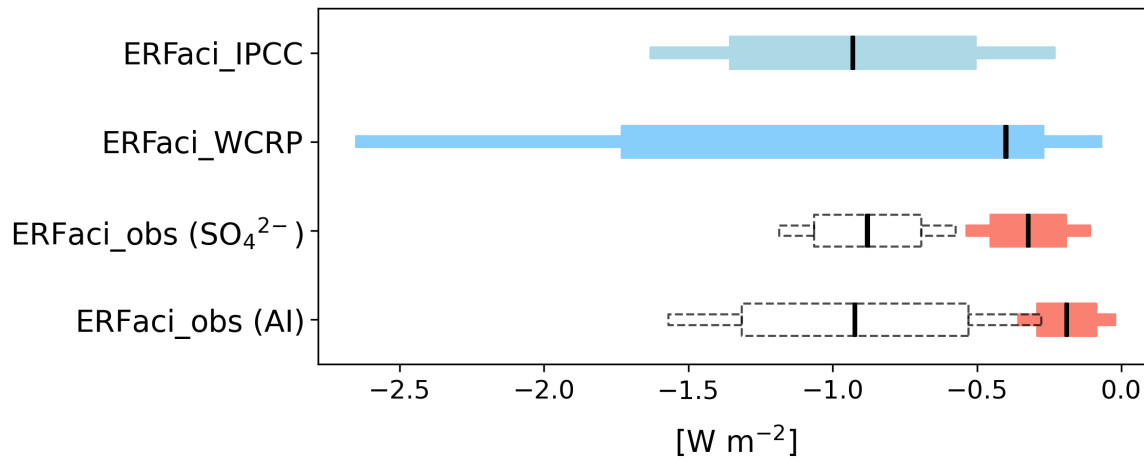
Figure 4. Estimates of globally averaged ERFaci values, including those from the IPCC Sixth Assessment Report, from the WCRP assessment, ERFaci_obs for SO 4 2- , and ERFaci_obs for Al. The ERFaci_obs estimates considering activation rate are shown in red, while those not considering activation rate are displayed in dashed grey. Thin and thick bars represent the 90% and 66% confidence intervals (CI), respectively, except for the WCRP estimate of ERFaci, which shows 68% CI for the thick bar. The black vertical lines indicate the best estimate of each ERFaci. The ERFaci estimate from the IPCC represents the assessment based on observational evidence alone.
