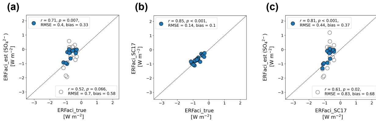
Figure 3. “Perfect-model” cross validation analysis of global-mean ERFaci estimates. (a) ERFaci_true versus ERFaci_est which is estimated by simplified version of Eq. (1) and Eq. (2) with \text{SO}_4^{2-} as the aerosol proxy (Appendix A4), (b) ERFaci_true versus ERFaci estimates obtained using the method proposed by Soden and Chung (2017; SC17), and (c) ERFaci_SC17 versus ERFaci_est. Filled blue circles represent estimates where the activation rate is considered, and open grey circles represent estimates without activation rate consideration. The correlation coefficient ( r ), associated p -value ( p ), Root Mean Square Error (RMSE), and bias are displayed in the upper left corner for the filled blue circles and in the lower right for the open grey circles in each panel. Bias is defined as the mean absolute difference from the 1:1 reference line, depicted by a dashed line. All panels have identical x and y axis ranges to highlight the variance among the estimation methods. Higher r values, lower RMSE, and minimal bias indicate consistency in ERFaci estimates across different estimation methods using CMIP6 models.
