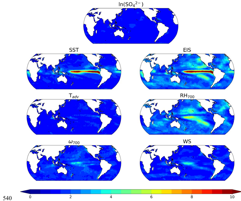
Figure A1. Variance inflation factors (VIF) for each environmental factor Y_i in CCF analysis, calculated as VIF_i = 1/(1 - R_i^2) , where R_i^2 represents the total variance in Y_i explained by the remaining environmental predictors. The environmental predictors include natural logarithmic sulfate mass concentration ( \ln(\text{SO}_4^{2-}) ), sea surface temperature (SST), estimated inversion strength (EIS), horizontal surface temperature advection ( T_{adv} ), relative humidity at 700 hPa ( \text{RH}_{700} ), vertical velocity at 700 hPa ( \omega_{700} ), and near-surface wind speed (WS).
