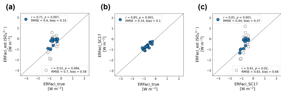
Figure 3. “Perfect-model” cross validation analysis of global-mean ERFaci estimates. (a) ERFaci_true versus ERFaci_est which is estimated by simplified version of Eq. (1) and Eq. (2) with \text{SO}_4^{2-} as the aerosol proxy (Appendix A4), (b) ERFaci_true versus ERFaci estimates obtained using the method proposed by Soden and Chung (2017; SC17), and (c) ERFaci_SC17 versus ERFaci_est. Filled blue circles represent estimates where the activation rate is considered, and open grey circles represent estimates without activation rate consideration. The correlation coefficient ( r ), associated p -value ( p ), Root Mean Square Error (RMSE), and bias are displayed in the upper left corner for the filled blue circles and in the lower right for the open grey circles in each panel. Bias is defined as the mean absolute difference from the 1:1 reference line, depicted by a dashed line. All panels have identical x and y axis ranges to highlight the variance among the estimation methods. Higher r values, lower RMSE, and minimal bias indicate consistency in ERFaci estimates across different estimation methods using CMIP6 models.
