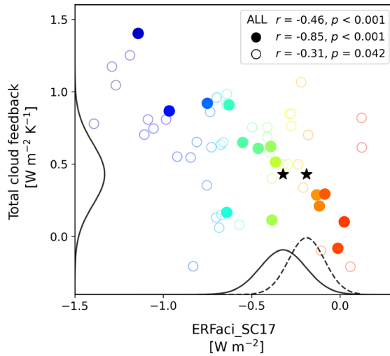
260 Figure 5. Correlation between global-mean ERFaci estimates obtained using the method proposed by Soden and Chung (2017; SC17), aimed at expanding the model availability, and the globally averaged total cloud feedback as determined by the corresponding models. Each dot represents a single model. The colors from red to blue indicate weak ERFaci models to strong negative ERFaci models. Filled circles represent the 15 “GOOD HIST” models that align more closely with historical observations of global-mean surface warming, whereas open circles denote the remaining models (Appendix A1.4). 265 Correlation coefficients ( r ) and their associated p -values ( p ) for the entire models, the “GOOD HIST” models, and remaining models are shown in the upper right corner. The probability density functions (PDFs), showing the 90% confidence intervals for observationally constrained ERFaci from sulfate mass concentration ( \text{SO}_4^{2-} ; solid line) and the aerosol index (AI; dashed line) when the activation rate is accounted for, are plotted along the x-axis, while the PDF for observationally constrained total cloud feedback (solid line), derived from Ceppi and Nowack (2021), is plotted on the y-axis (amplitudes scaled arbitrarily). 270 Stars denote the best estimates of the PDFs, signifying the most probable values within the distributions.
