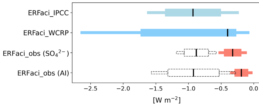
Figure 4. Estimates of globally averaged ERFaci values, including those from the IPCC Sixth Assessment Report, from the WCRP assessment, ERFaci_obs for SO 4 2- , and ERFaci_obs for AI. The ERFaci_obs estimates considering activation rate are shown in red, while those not considering activation rate are displayed in dashed grey. Thin and thick bars represent the 90% and 66% confidence intervals (CI), respectively, except for the WCRP estimate of ERFaci, which shows 68% CI for the thick bar. The black vertical lines indicate the best estimate of each ERFaci. The ERFaci estimate from the IPCC represents the assessment based on observational evidence alone.
