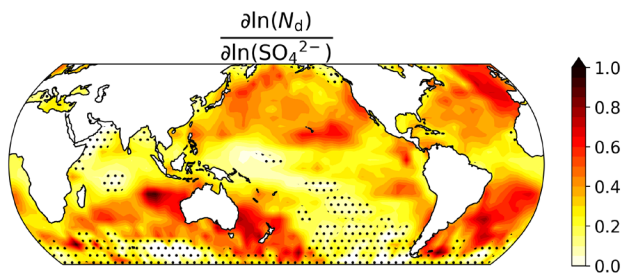
Figure 1. Regression coefficient map of the activation rate of cloud droplet number concentration ( N_d ) in response to variations in sulfate aerosol mass concentration ( SO_4^{2-} ) for the period January 2003 to December 2019, derived from cloud controlling factor (CCF) analysis (Appendix A3). The color scale indicates the magnitude of sensitivity, where an increase in SO_4^{2-} corresponds to an increase in N_d . Areas with stippling indicate where the changes are not statistically different from zero at the 95% confidence level using a Student's t-test.
