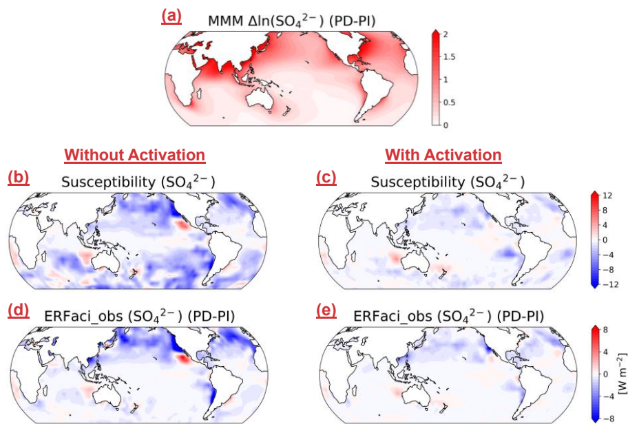
Figure 2. Spatial distribution of ERFaci_obs components and the estimated ERFaci_obs differentiated by the consideration of the activation rate. (a) Multi-model mean (MMM) of changes in \text{SO}_4\text{SO}_4^{2-} between pre-industrial (PI) and present-day (PD) periods. 13 models are used for this analysis (Table S1). (b,c) Susceptibility of low cloud radiative effect to \text{SO}_4\text{SO}_4^{2-} derived from CCF analysis using observational and reanalysis data (Appendix A3). (d,e) Observationally constrained ERFaci for \text{SO}_4\text{SO}_4^{2-} estimated by multiplying the susceptibility with the changes in \text{SO}_4\text{SO}_4^{2-} .
