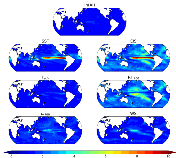
Figure A2. Same as Figure A1, but for AI instead of \text{SO}_4 .
