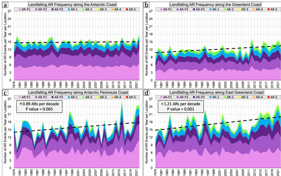
560 Figure 11. (a) The time series of averaged frequency of landfalling ARs along the Antarctic coastline according to the new polar AR scale in 1979–2022 based on ERA5. Different colors denote the ARs at different scales and the dashed black line is the linear trend for the frequency of all ARs. (b), (c), and (d) are the same as (a) but for the coastline of Greenland in the polar 565 region, Antarctic Peninsula (highlighted in the green box in Fig. 4b), and East Greenland (highlighted in the green box in Fig. 4c) respectively. The P values in (c) and (d) are calculated from a T-test.
