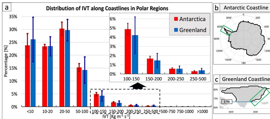
280 Figure 4. (a) Averaged distribution of IVT values based on 6-hourly samples along the coastlines of Antarctica and Greenland in polar regions from 1979 to 2022, using ERA5 reanalysis data. The vertical bars denote the spread (one standard deviation) of the frequency over the 44 years. Panels (b) and (c) depict the coastlines of Antarctica and Greenland in polar regions (thick black lines), respectively. The green boxes in (b) and (c) highlight the coastlines of the Antarctic 285 Peninsula and East Greenland used for the analysis of the AR frequency trend in Figure 13.
