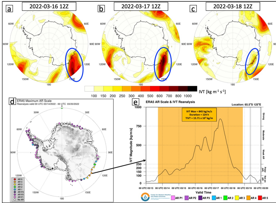
Figure S3 Panels (a)-(c): three snapshots of IVT associated with an extremely strong landfalling AR event (highlighted in the blue ovals) over East Antarctica in the middle of March 2022. The colors in (a)-(c) are the IVT ( \text{kg m}^{-1} \text{s}^{-1} ) from the ERA5 reanalysis data at 1200 UTC on the 16 th , 17 th , and 18 th of March 2022, respectively. Panel (d): maximum AR scale along the coastline of Antarctica during March 14 th –20 th 2022. (e) shows the time series of IVT at the AR landfalling location ( 65.5^{\circ}\text{S} , 125^{\circ}\text{E} ) and the corresponding AR scale.
