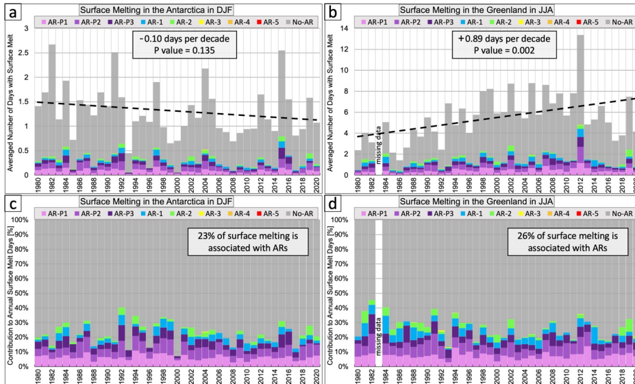
675 Figure 13. (a) Stacked number of days with surface melting over Antarctica in DJF during 1980- 2020; gray indicates surface melting not associated with ARs and the other colors indicate surface melting associated with different AR scales. The dashed line is the linear trend of total melt days. (b) Same as (a) but for Greenland and in JJA. (c) Same as (a) but Y-axis is the 680 percentage of surface melting days not associated with ARs (gray) and associated with different AR scales (other colors). (d) Same as (c) but for the coast of Greenland and in JJA.
