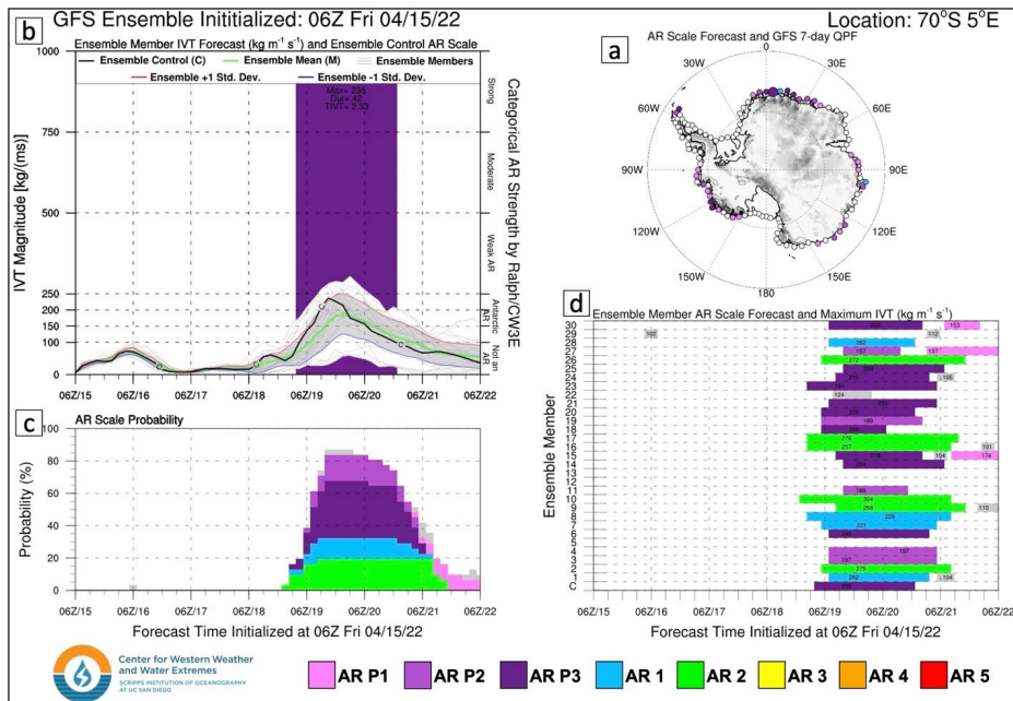
725 Figure 14. CW3E AR scale ensemble diagnostic forecast tool for 70°S, 5°E from the GEFS. 730 initialized at 06Z 04/15/2022. Dots along the Antarctic coast indicate locations where information such as that shown in other panels can be provided; here other panels refer to the larger point at 70°S, 5°E). (a) Maximum Polar AR scale forecast over the next seven days along the Antarctic Coast (colored dots), enlarged dot represents the location shown in panels b-d. (b) 735 Seven day forecast of IVT from each ensemble member (thin gray lines), the ensemble mean (green line), control member (black line) and +/- 1 standard deviation from the ensemble mean (red and blue lines and gray shading). Color shading represents the timing of the Polar AR scale from the control member. (c) Forecasted probability of each Polar AR scale ranking as a function of lead time based on the number of ensemble members predicting an AR. (d) Forecasted Polar AR scale timing and ranking from each ensemble member, text values represent the maximum IVT magnitude and timing during a forecasted AR.
