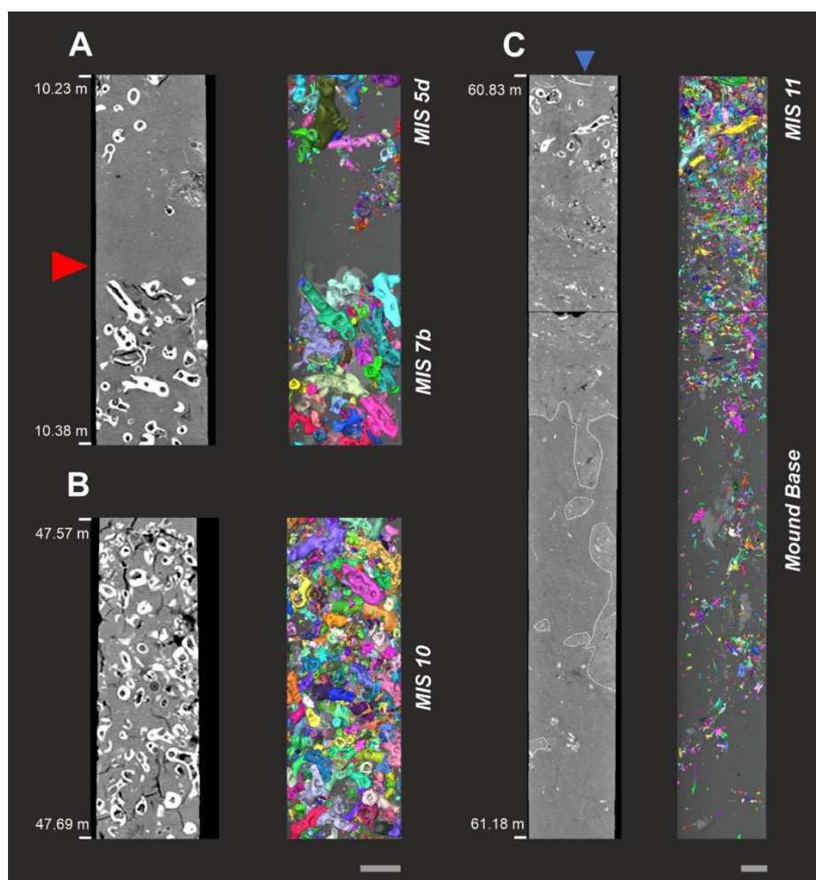
335 Fig. 2: CT-image based core section close-ups of the MeBo on-mound core GeoB18116-2 collected from Dragon Mound (left: orthoslice; right: 3D macrofossils reconstruction, each coral fragment with individual color; core depth given in CSF-B meters below seafloor). (A) Hiatus covering a timespan of ~100 kyr between mound formation phases DM5 and DM6, red arrow indicating the top of DM5 (coral ages ~MIS7b), followed by DM6 (coral ages ~MIS5d). (B) Example of a high-coral carbonate-bearing unit during mound formation phase DM2 (MIS10, ~350 kyr BP). (C) Scan of the mound base (61.1 mbsf), including burrows filled with cold-water coral mound sediments (white outline), the first cold-water coral clasts and several oyster shells (blue arrow), DM1 (~MIS11). Grey scale bars on the bottom represent ~2 cm length.
