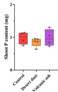
Figure 1 (a-f): Biomass and total P content increases due to dust application treatments at aCO 2 of 412ppm. (a) Image of experiment setting of the root treatment. Image taken immediately after the dust application. The amount of dust remaining on the plant at the end of the experiment was significantly smaller. (b) Image of experiment setting of foliar treatment. (c) Shoot biomass of root treated plants. (d) Shoot biomass of foliar treated plants. (e) Shoot total P content of root treated plants. (f) Shoot total P content of foliar treated plants. The red color represents control plants, orange desert dust treatment and purple volcanic ash treatment. Asterisks represent statistically significant differences between bars ( P < 0.05 , Tukey test). Error bars represent standard deviations ( n = 5 ).
