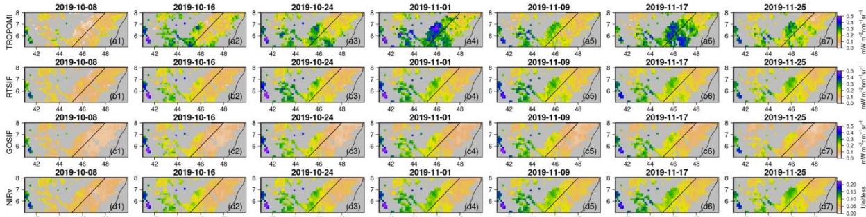
Figure 5: Intra-seasonal variations of (a) TROPOMI SIF, (b) RTSIF, (c) GOSIF, (d) MODIS NIRv in the shrublands of Region 1 during October 8 th and November 25 th , 2019. The date labels represent the starting date of each 8-day period.
