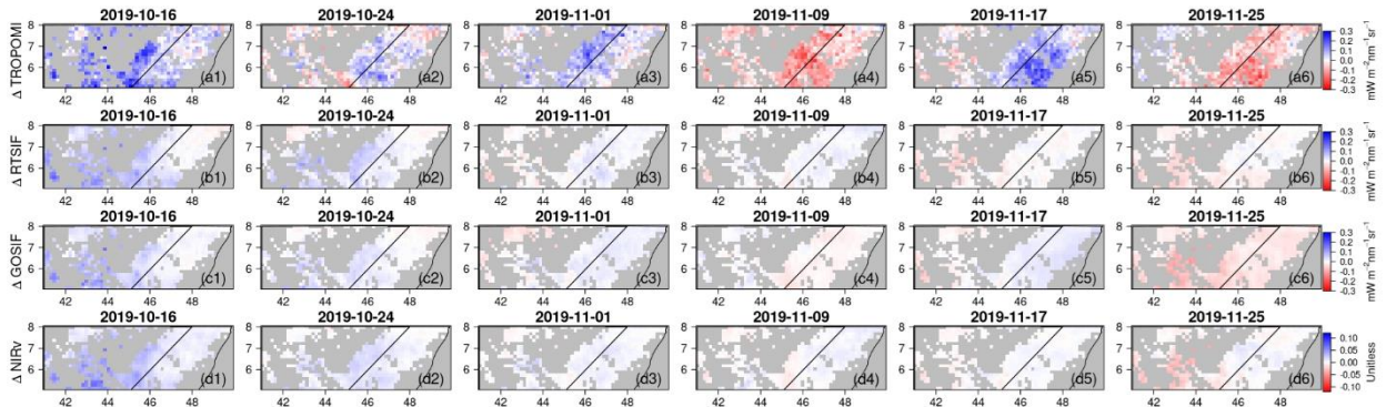
Figure 6: Temporal change rate of (a) TROPOMI SIF, (b) RTSIF, (c) GOSIF, (d) MODIS NIRv in the shrublands of Region 1 during October 16 th and November 25 th , 2019. The date labels represent the starting date of each 8-day period.
