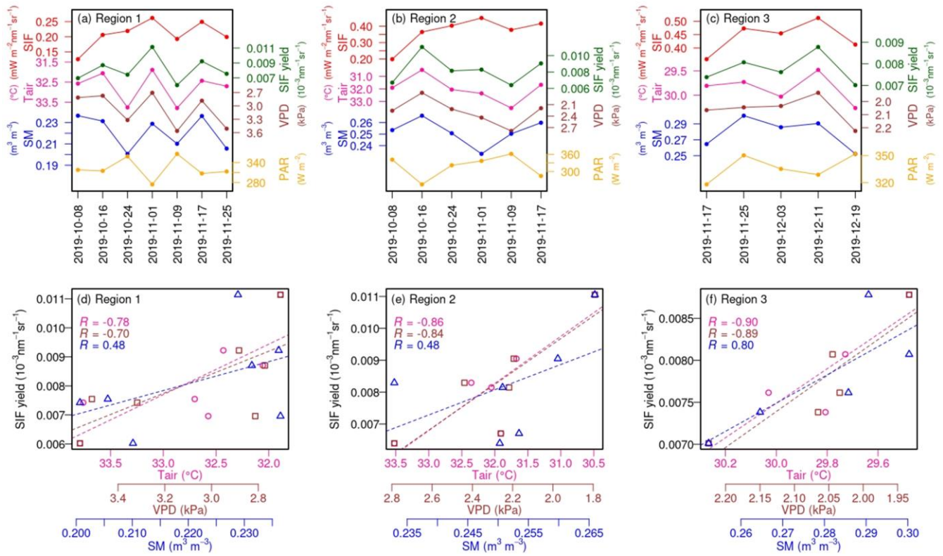
415 Figure 7: (a) – (c) Intra-seasonal variations of TROPOMI SIF, TROPOMI SIF yield, Tair, VPD, SM and PAR for the three sub- domains during the selected time windows (Fig. 4). The y axis-axes for Tair and VPD are reversed for visual clarity. The x axis labels represent the starting date of each 8-day interval. (d) – (f) Scatterplots between TROPOMI SIF yield and Tair (pink circle), VPD (brown square), and SM (blue triangle) for the three sub-domains during the selected time windows. The dashed lines represent fitted linear regression lines, with correlation coefficients (R) noted in the upper left of each panel.
