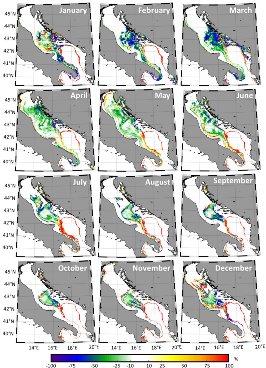
Figure 9. Monthly climatology of the climate adjustments (in percent) associated with the DWH and defined, over the 31 year of the simulations, as the difference between RCP 8.5 and historical monthly medians divided by historical monthly medians.
