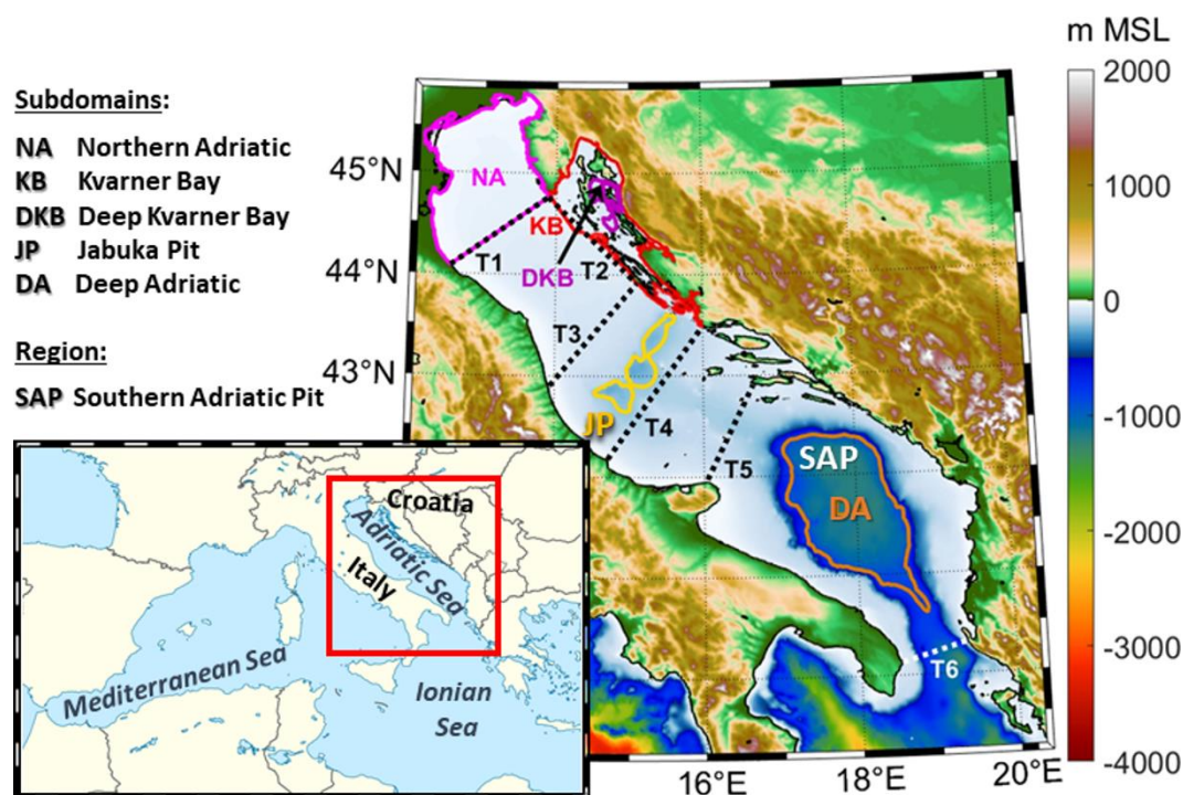
Figure 1. Topo-bathymetry of the AdriSC climate model with the locations of the 5 subdomains (colored polygons) and 6 transects (dotted black and white lines) used in the study.
