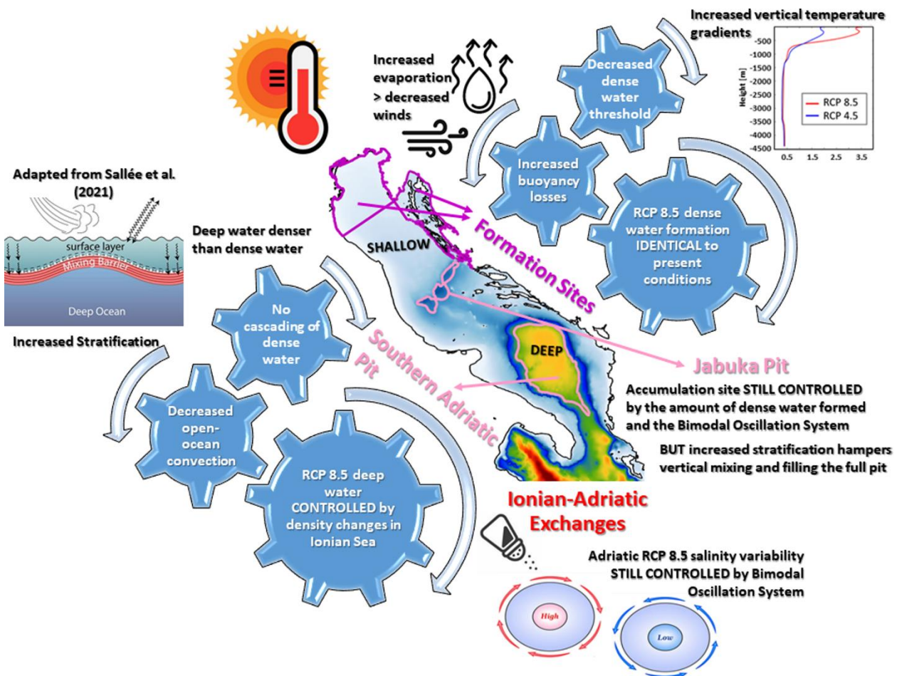
435 Figure 16. Adriatic dense and deep- water far-future dynamics as seen by the kilometre-scale atmosphere-ocean AdriSC model under the Pseudo-Global Warming assumption.
