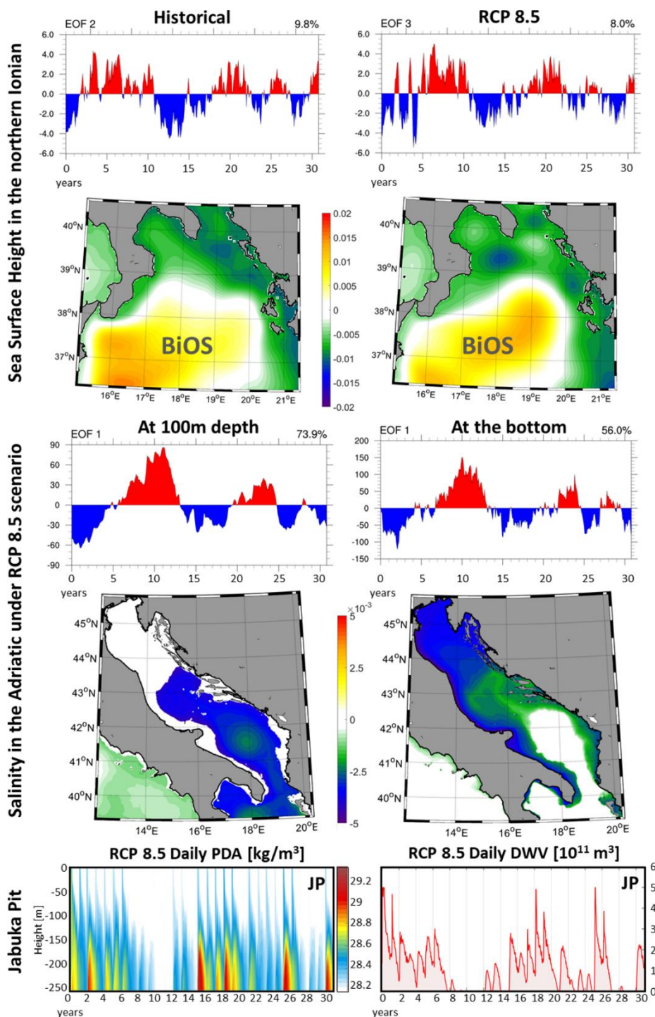
Figure 14. Normalized spatial EOF components and associated time series of amplitude for both the historical and RCP 8.5 AdriSC ROMS 3-km Sea Surface Height (SSH) over the northern Ionian Sea (top panels), RCP 8.5 AdriSC ROMS 1-km salinity at 100 m and the bottom of the Adriatic Sea (middle panels). Time series of the daily vertical Potential Density Anomaly (PDA) and Dense Water Volume (DWV) in the JP subdomain for the RCP 8.5 simulation (bottom panels).
