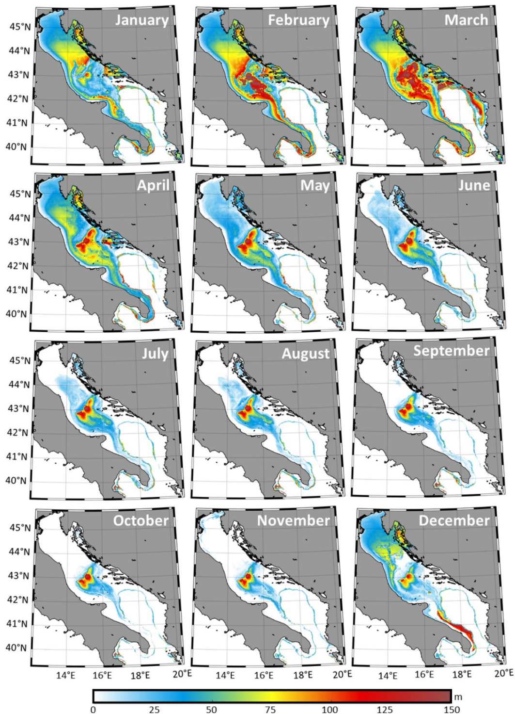
275 Figure 8. Historical monthly climatology of the median Dense Water Height (DWH; defined for \sigma \geq 29.2 kg/m 3 ) over the 31 years of the historical simulation.
