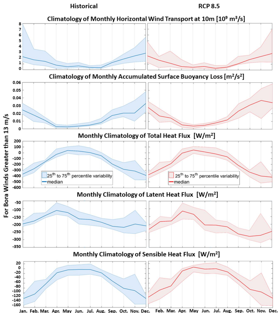
235 Figure 6. Monthly climatologies of the median, 25th and 75th percentiles of the horizontal wind transport at 10 m, the accumulated surface buoyancy loss and the total, latent and sensible heat fluxes defined over the 31 years of the historical and RCP 8.5 simulations for the selected Bora events.
