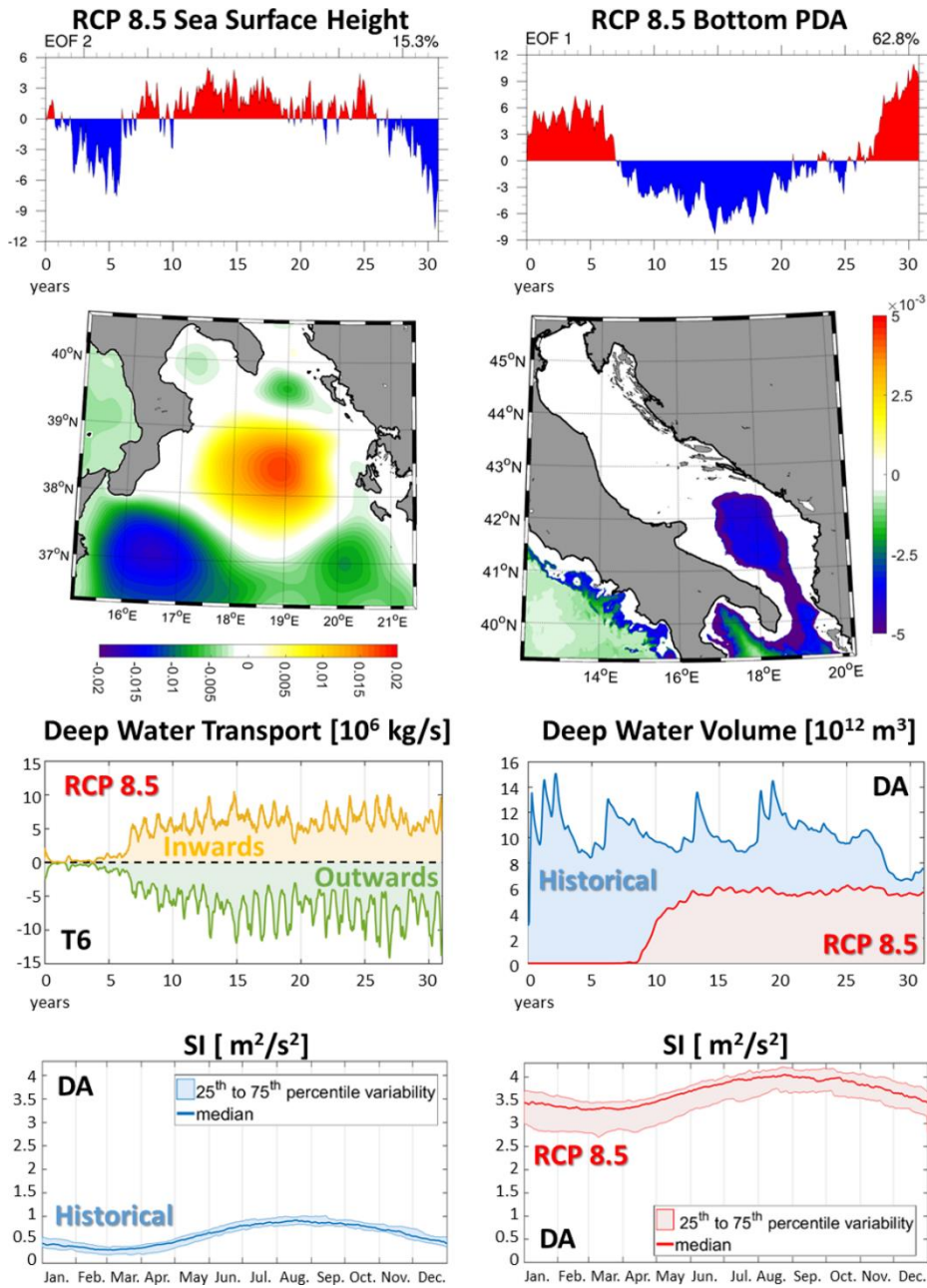
Figure 15. Normalized spatial EOF components and associated time series of amplitude for the RCP 8.5 AdriSC ROMS 3-km Sea Surface Height (SSH) over the northern Ionian Sea (top left panels). RCP 8.5 AdriSC ROMS 1-km bottom PDA, for depths greater than 800 m in the Adriatic Sea (top right panels). Time series of the daily deep-water transport along the T6 transect for the RCP 8.5 simulation (middle left panel). DWV and SI over the DA subdomain for the historical and RCP 8.5 simulations (middle right and bottom panels).
