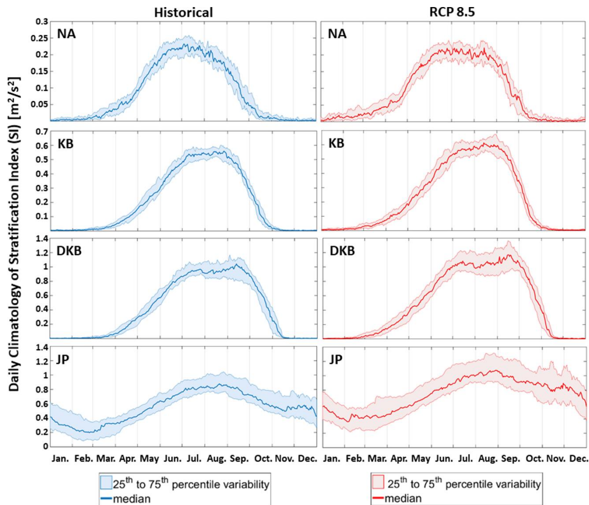
325 Figure 11. Daily climatologies of the median, 25 th and 75 th percentiles of the Stratification Index (SI) defined over the NA, KB, DKB and JP subdomains for the 31 years of the historical and RCP 8.5 simulations.
