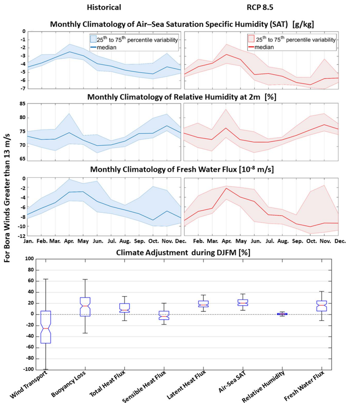
Figure 7. Monthly climatologies of the median, 25th and 75th percentiles of the air minus sea saturation specific humidity, the relative humidity at 2 m and the fresh water flux defined over the 31 years of the historical and RCP 8.5 simulations for the selected Bora events (top panels). Climate adjustments (in percent) for the 8 variables used in the Bora event analyses presented as box plots during DJFM (bottom panel).
