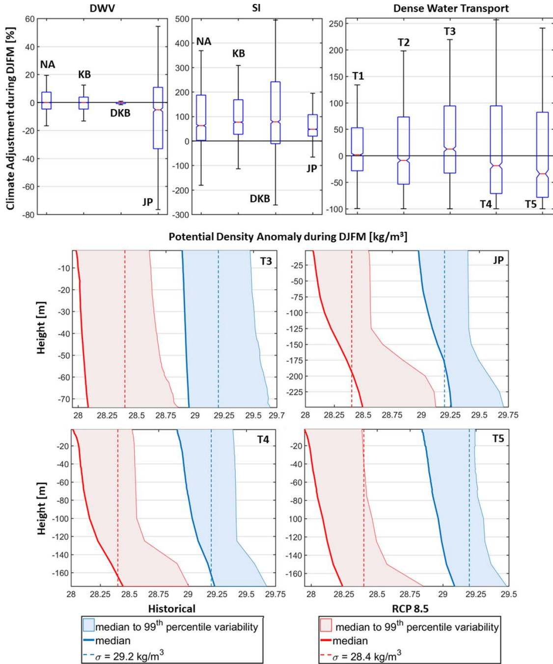
Figure 13. Climate adjustments (in percent) for the 3 variables used in the NAddW dynamics analyses presented as box plots during DJFM (top panels). Variability of the historical and RCP 8.5 pycnoclines defined between the median and 99 th percentile of the PDA along the T3 to T5 transects and within the Jabuka Pit during DJFM (bottom panels).
