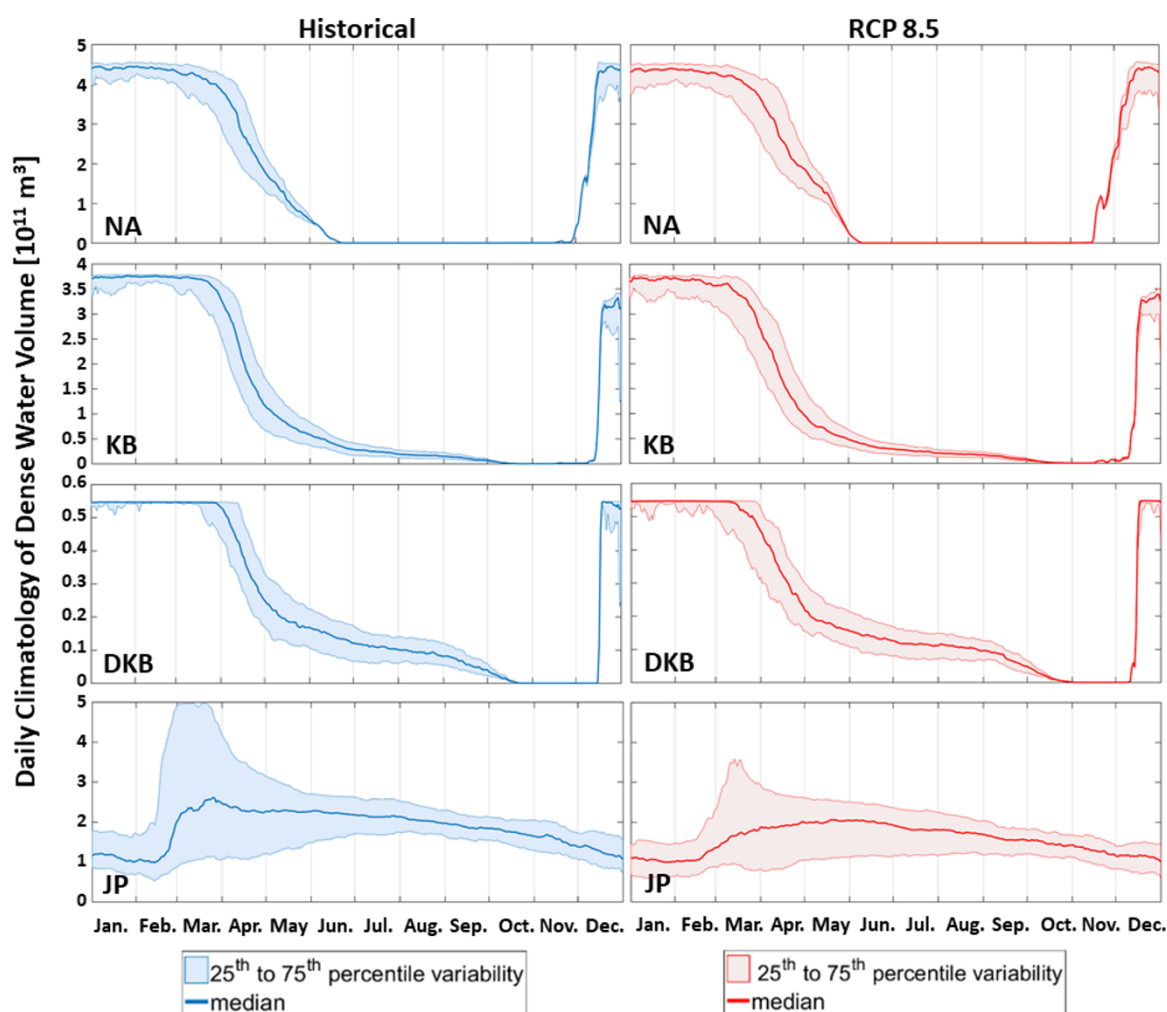
320 Figure 10. Daily climatologies of the median, 25 th and 75 th percentiles of the Dense Water Volume (DWV) defined over the NA, KB, DKB and JP subdomains for the 31 years of the historical (defined for \sigma \geq 29.2 kg/m 3 ) and RCP 8.5 (defined for \sigma \geq 28.4 kg/m 3 ) simulations.
