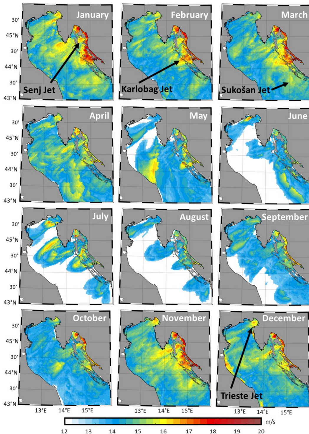
Figure 4. Historical monthly climatology of the spatial extent and intensity of the selected windstorms ( \geq 13 m/s) defined as the monthly median wind speed at 10 m over the 31 years of the historical simulation.
