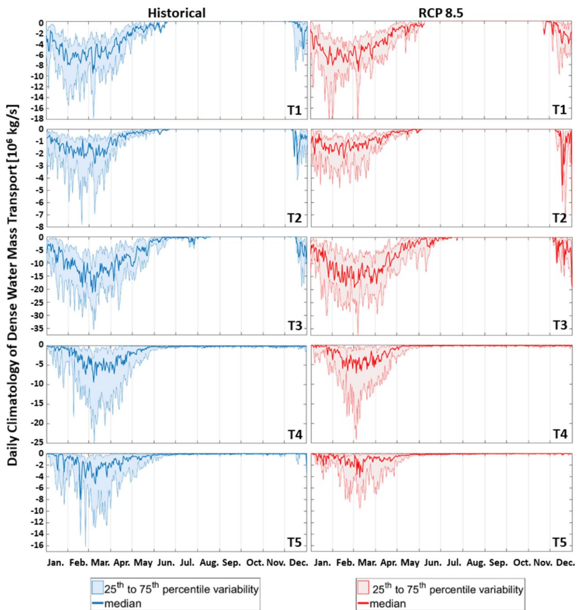
Figure 12. Daily climatologies of the median, 25 th and 75 th percentiles of the dense water transport defined along the T1 to T5 transects for the 31 years of the historical and RCP 8.5 simulations.
