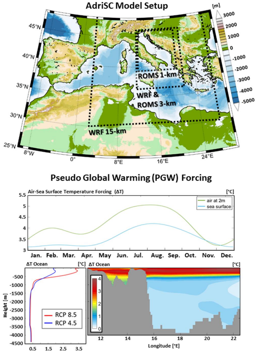
Figure 2. Spatial coverage and horizontal resolution of the different grids used in the AdriSC climate model (top panel) and Pseudo Global Warming temperature forcing imposed in the AdriSC extreme warming simulation (bottom panels).
