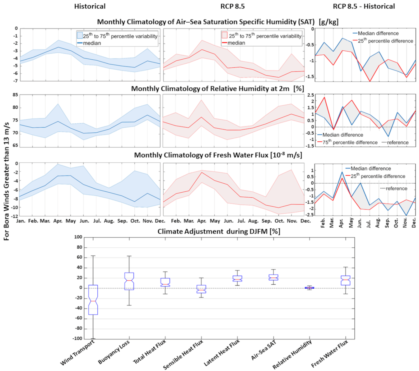
280 Figure 7. For the selected Bora events, monthly climatologies of the median, 25th and 75th percentiles of the air minus sea saturation specific humidity, the relative humidity at 2 m and the fresh water flux defined over the 31 years for the historical, RCP 8.5 and RCP 8.5 minus historical conditions (top panels). Climate adjustments (in percent) for the 8 variables used in the Bora event analyses presented as box plots during DJFM (bottom panel).
