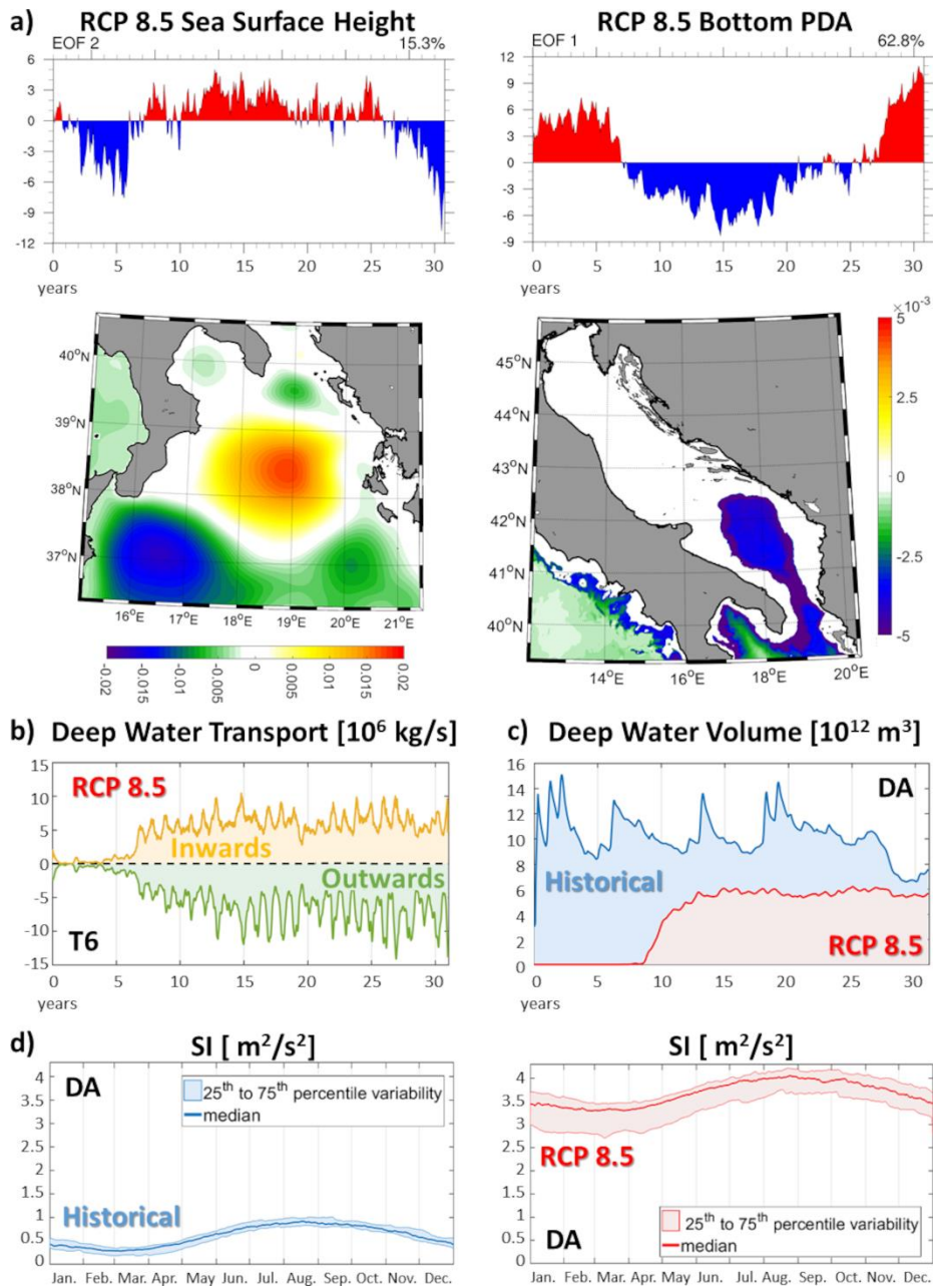
455 Figure 15. a) Normalized spatial EOF components and associated time series of amplitude for the RCP 8.5 AdriSC ROMS 3-km Sea Surface Height (SSH) over the northern Ionian Sea and the RCP 8.5 AdriSC ROMS 1-km bottom PDA, for depths greater than 800 m in the Adriatic Sea. b) Time series of the daily deep-water transport along the T6 transect for the RCP 8.5 simulation. c) DWV and d) SI over the DA subdomain for the historical and RCP 8.5 simulations.
