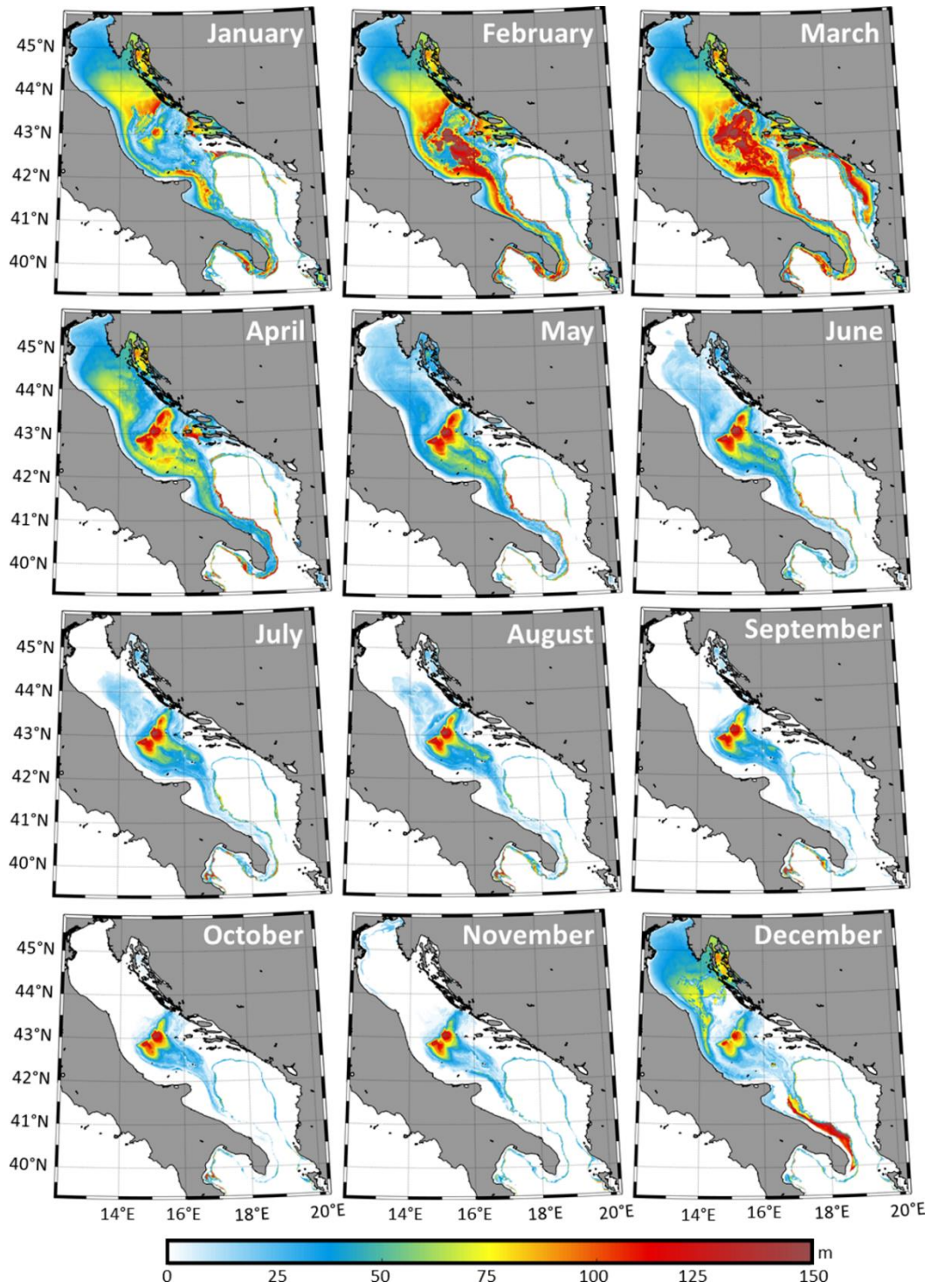
Figure 8. Historical monthly climatology of the median isopycnal depth (ID; defined for \sigma \geq 29.2 \text{ kg/m}^3 ) over the 31 years of the historical simulation.
