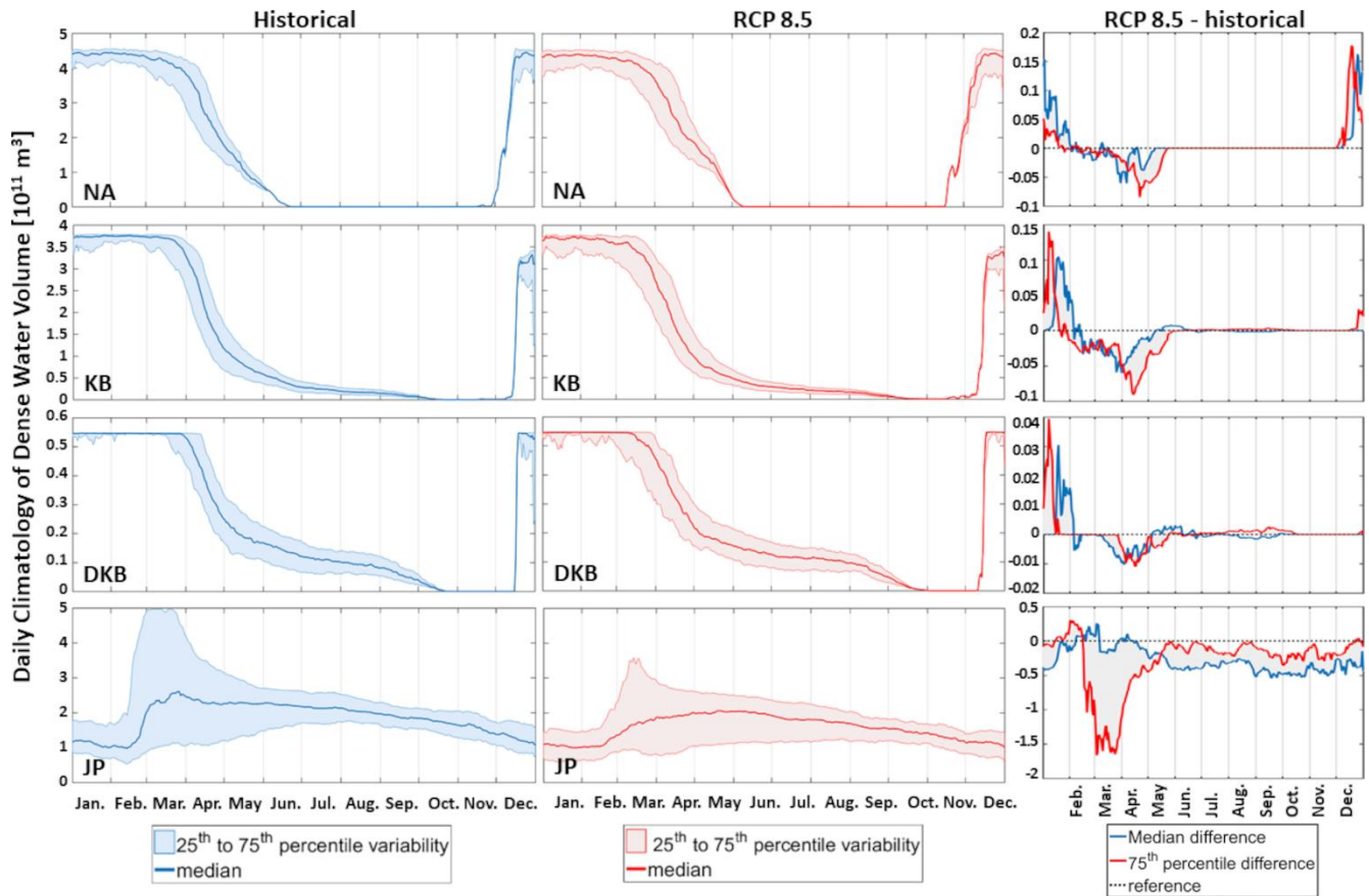
325 Figure 10. Daily climatologies of the median, 25 th and 75 th percentiles of the Dense Water Volume (DWV) defined over the NA, KB, DKB and JP subdomains for the 31 years of the historical (defined for \sigma \geq 29.2 \text{ kg/m}^3 ), RCP 8.5 (defined for \sigma \geq 28.4 \text{ kg/m}^3 ) and RCP 8.5 minus historical conditions.
