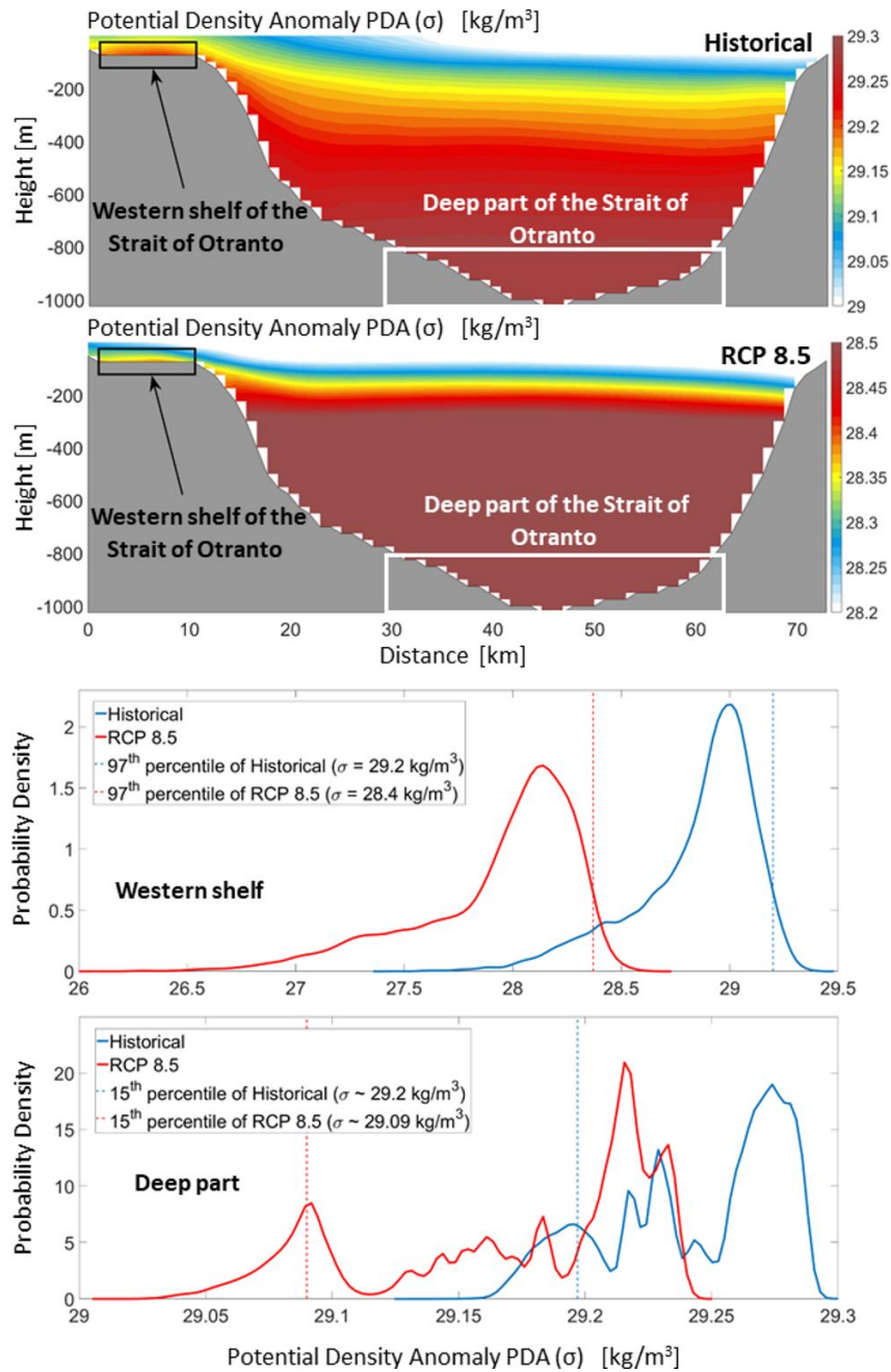
160 Figure 3. Spatial plots of the vertical transect along the Strait of Otranto for the median of the PDAs over the 31-year historical and RCP 8.5 simulations (top panels) and historical and RCP 8.5 PDA probability density functions at the bottom of the western shelf (black box) and for depths greater than 800 m (white box) along the Strait of Otranto. It should be noted that, in the colour plots, historical and RCP 8.5 results are presented with different extrema in density for a better visualization but with identical ranges ( 0.3 \text{ kg/m}^3 ) to emphasize the increased stratification.
