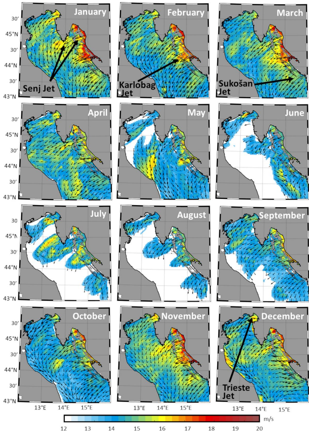
230 Figure 4. Historical monthly climatology of the spatial extent, intensity and direction (as vectors) of the selected windstorms ( \geq 13 m/s) defined as the monthly median wind speed at 10 m over the 31 years of the historical simulation.
