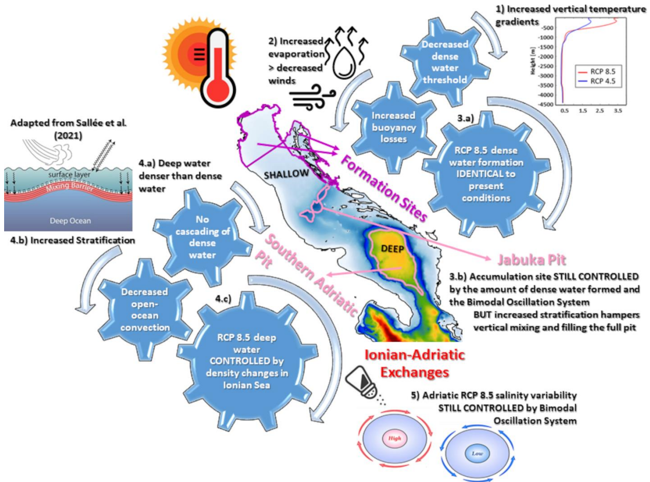
470 Figure 16. Visual summary of the study. Adriatic dense and deep- water far-future dynamics as seen by the kilometre-scale atmosphere-ocean AdriSC model under the Pseudo-Global Warming assumption. The numbers and letters correspond to the description of the different findings as described in the conclusions.
