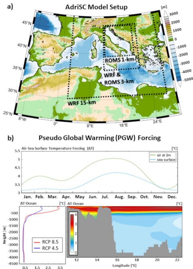
Figure 2. Spatial coverage and horizontal resolution of the different grids used in the AdriSC climate model (top-panel) and Pseudo Global Warming temperature forcing imposed in the AdriSC extreme warming simulation (bottom-panels).
