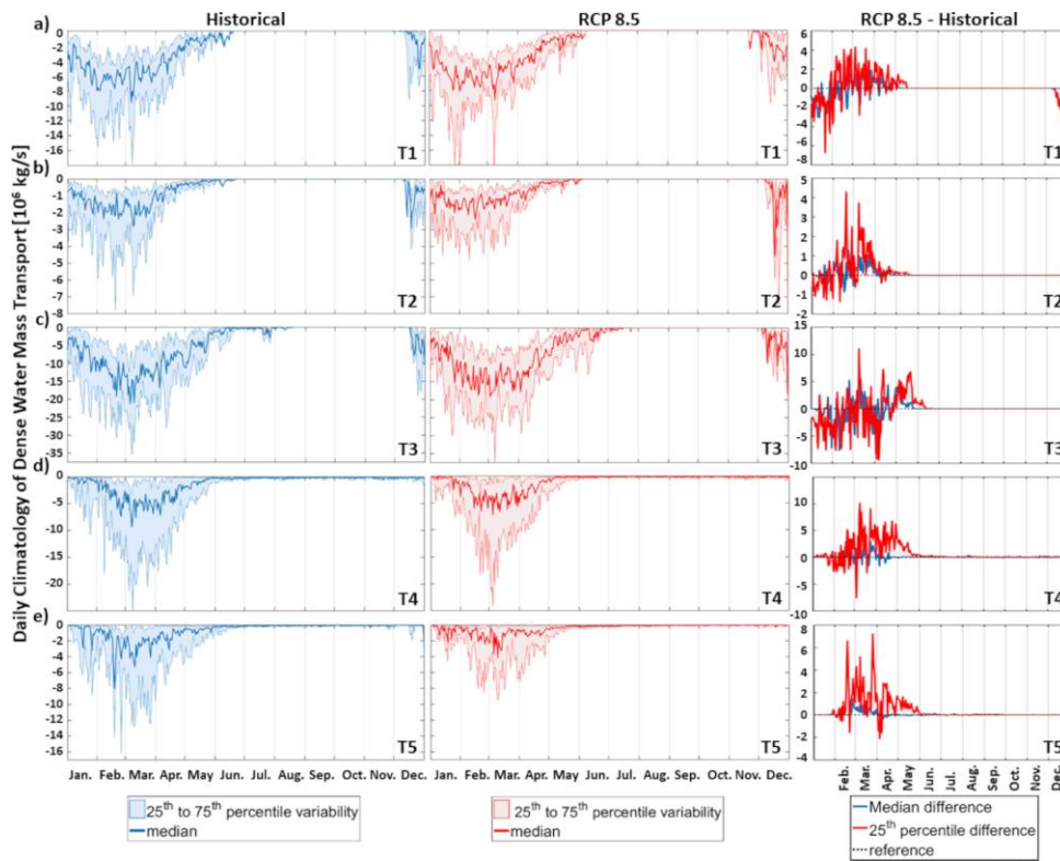
Figure 12. Daily climatologies of the median, 25 th and 75 th percentiles of the dense water transport defined along the T1 to T5 (a to e) transects for the 31 years of the historical, RCP 8.5 and RCP 8.5 minus historical conditions.
