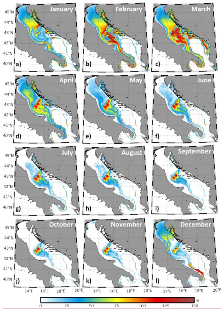
315 Figure 8. Historical monthly climatology of the median isopycnal depth depth (ID; defined for \sigma \geq 29.2 \text{ kg/m}^3 ) over the 31 years of the historical simulation.
