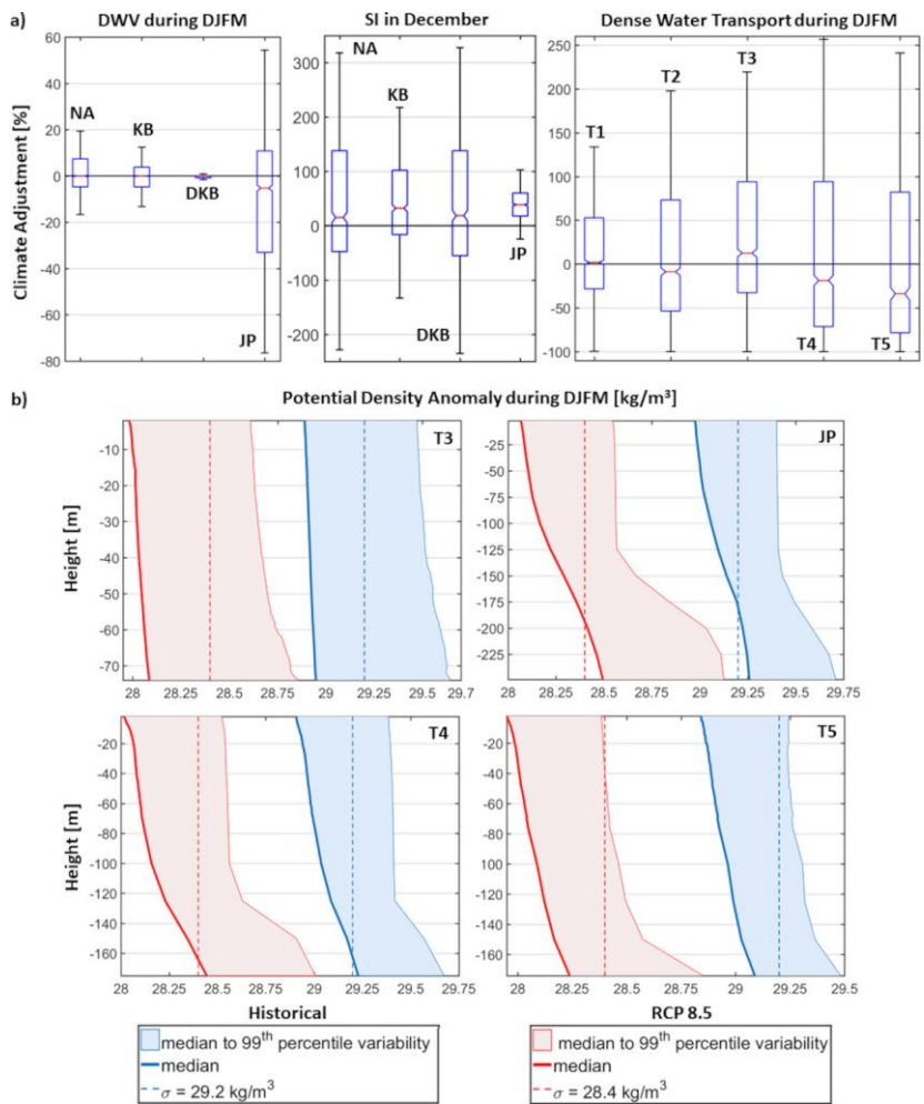
Figure 13. Climate adjustments (in percent) for the 3 variables used in the NAddW dynamics analyses presented as box plots during DJFM for DWV and mass transports and in December for SI ( atop-panels ). Variability of the historical and RCP 8.5 pycnoclines defined between the median and 99 th percentile of the PDA along the T3 to T5 transects and within the Jabuka Pit during DJFM ( bottom-panels ).
