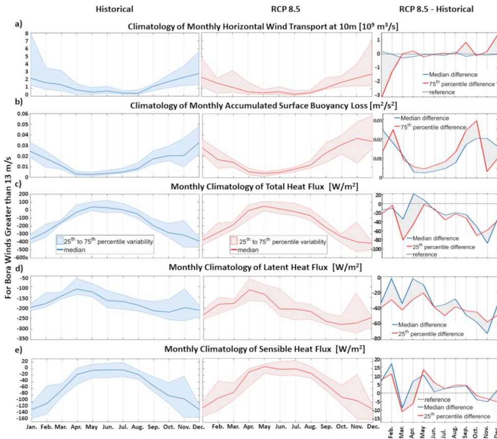
Figure 6. For the selected Bora events, monthly climatologies of the median, 25 th and 75 th percentiles of the horizontal wind transport at 10 m (a), the accumulated surface buoyancy loss (b) and the total (c), latent (d) and sensible (e) heat fluxes defined over the 31 years for the historical, RCP 8.5 and RCP 8.5 minus historical conditions.
