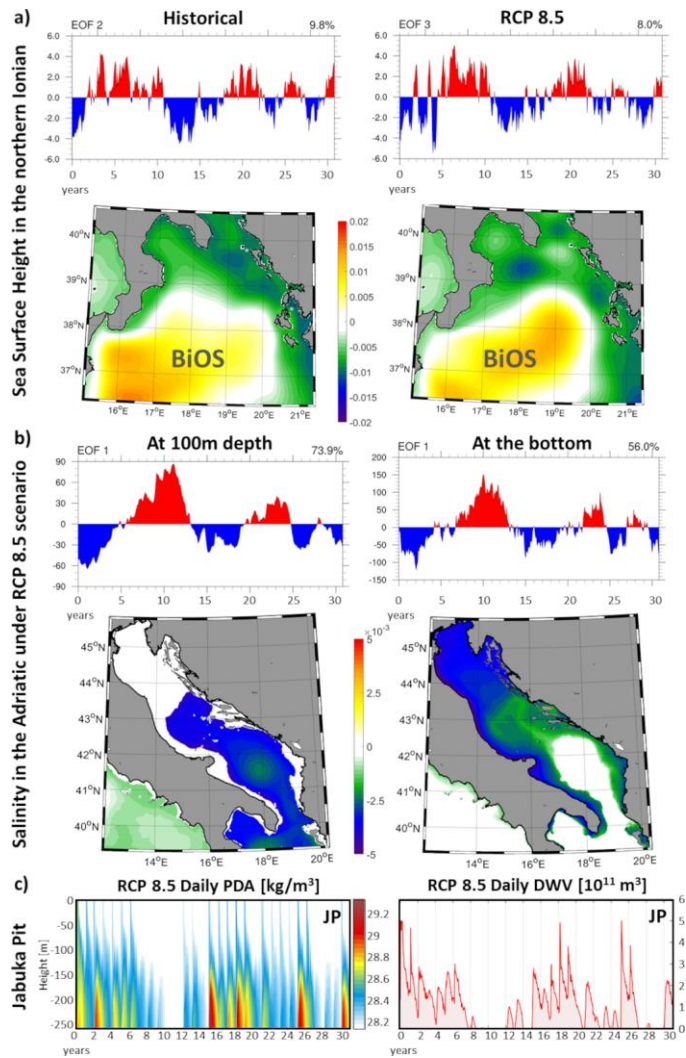
430 Figure 14. a) Normalized spatial EOF components and associated time series of amplitude for both the historical and RCP 8.5 AdriSC ROMS 3-km Sea Surface Height (SSH) over the northern Ionian Sea ( a ). b) RCP 8.5 AdriSC ROMS 1-km salinity at 100 m and the bottom of the Adriatic Sea ( middle-panels ). c) Time series of the daily vertical Potential Density Anomaly (PDA) and Dense Water Volume (DWV) in the JP subdomain for the RCP 8.5 simulation ( bottom-panels ).
