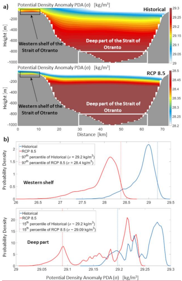
Figure 3. Spatial plots of the vertical transect along the Strait of Otranto for the median of the PDAs over the 31-year historical and RCP 8.5 simulations (atop panels) and historical and RCP 8.5 PDA probability density functions at the bottom of the western shelf (black box) and for depths greater than 800 m (white box) along the Strait of Otranto (b). It should be noted that, in the colour plots, historical and RCP 8.5 results are presented with different extrema in density for a better visualization but with identical ranges ( 0.3 \text{ kg/m}^3 ) to emphasize the increased stratification.
