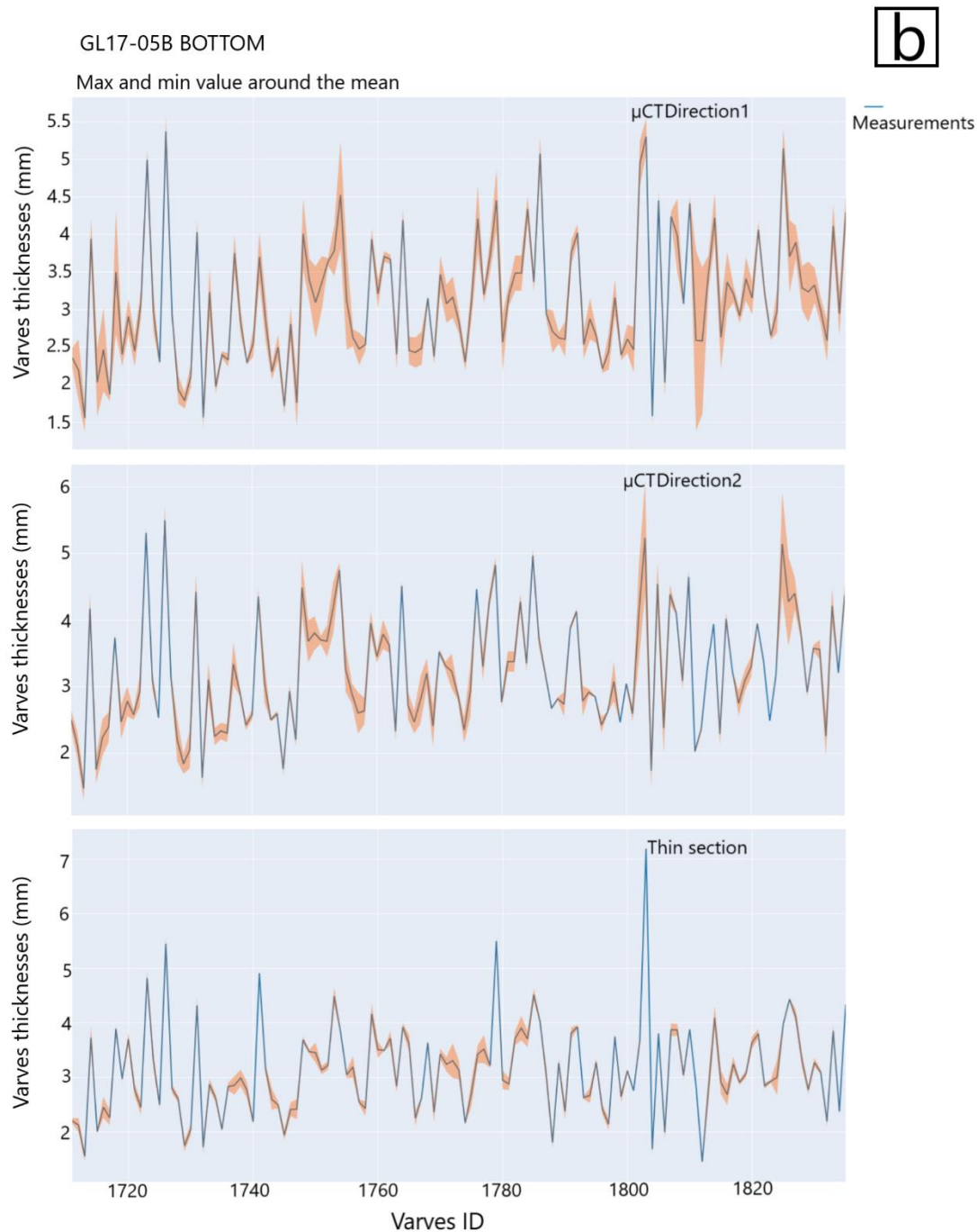
Figure 8: Mean varve thicknesses of the three measurements made in directions 1 (top panels) and 2 (middle panels) using the micro-CT and on thin sections (lower panels) for cores GL17-05B at the top (a), and at the bottom (b). The maximum and minimum values around the mean relating to the measurements are in the orange shaded area, and the varves ID represents the identification of the varve over an interval.
