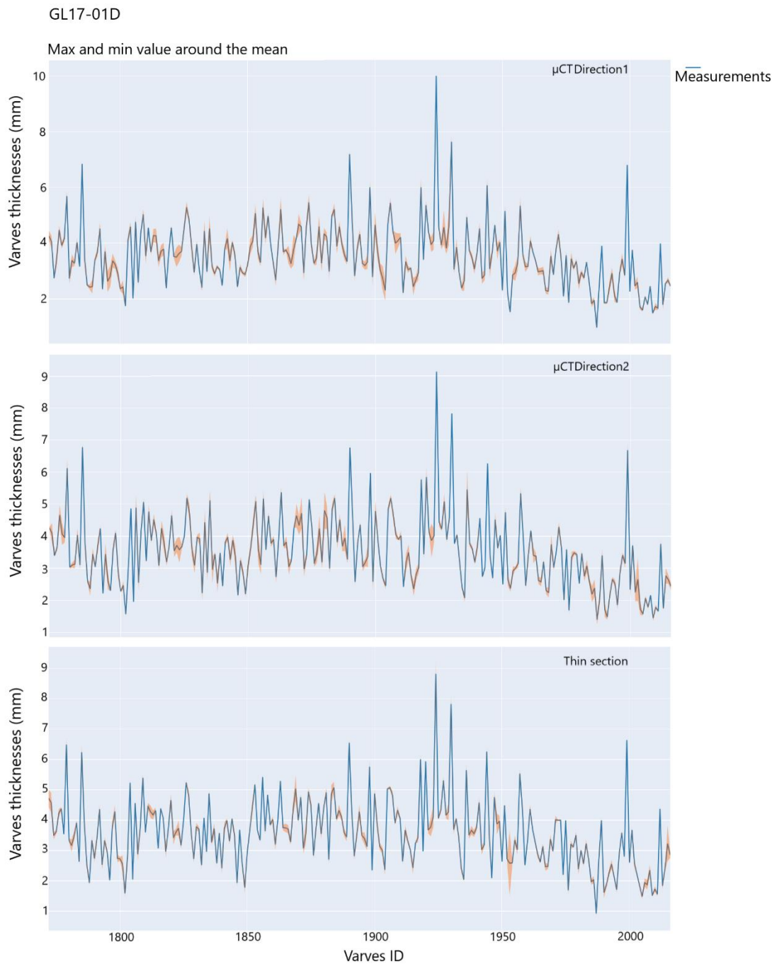
Figure 6: Mean varve thicknesses of the three measurements made in directions 1 (top panels) and 2 (middle panels) using the \mu CT and on thin sections (lower panels) for cores GL17-01D. The maximum and minimum values around the mean relating to the measurements are shown in the orange shaded area, and the varve ID represents the identification of the varve over an interval.
