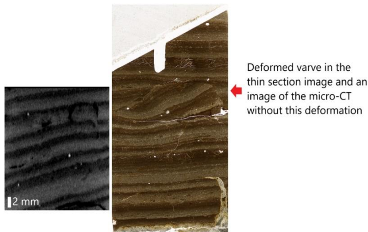
Figure 15: The deformation of varves in the thin section plane and the corresponding varve with \mu CT image in the sediment core GL17-05B.
