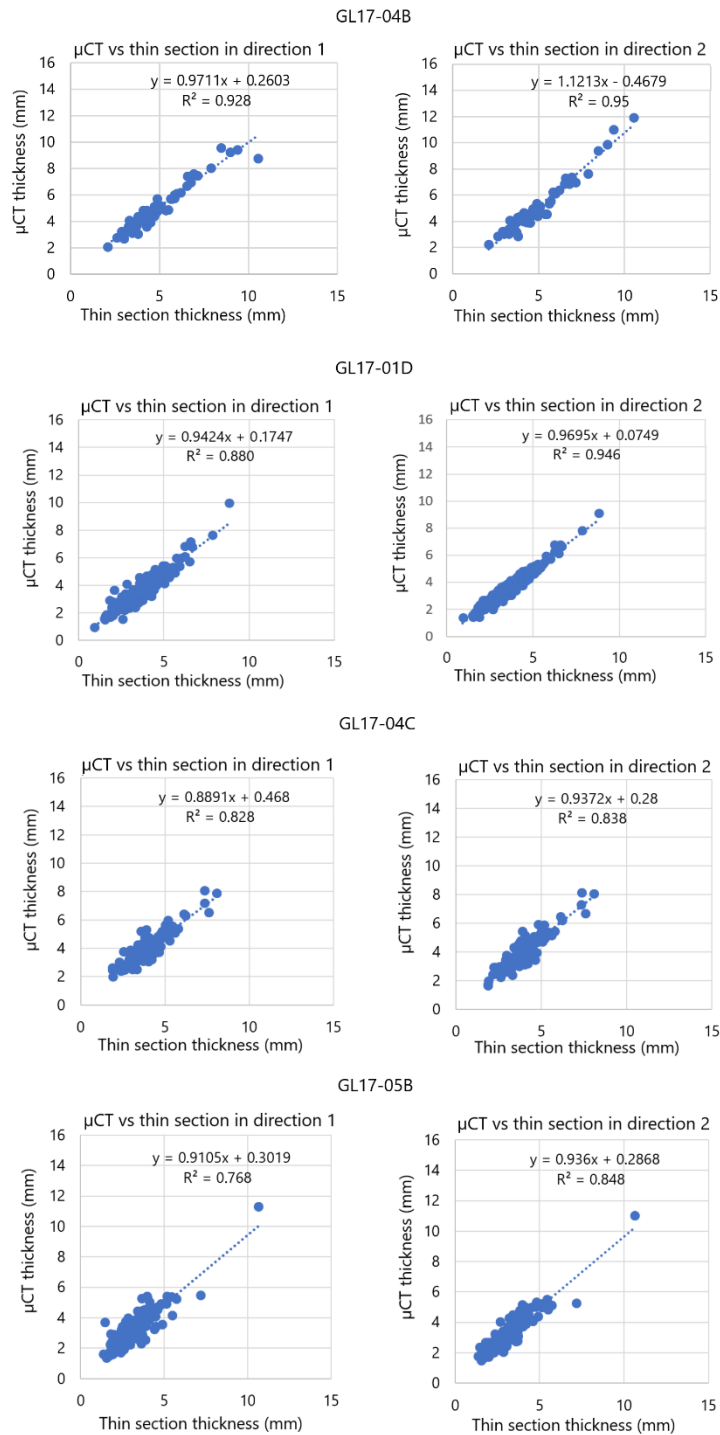
250 Figure 10: Linear regression between mean thickness measurements of μCT and thin sections respectively on the sediment cores GL17-04B, GL17-01D, GL17-04C, and GL17-05B.
