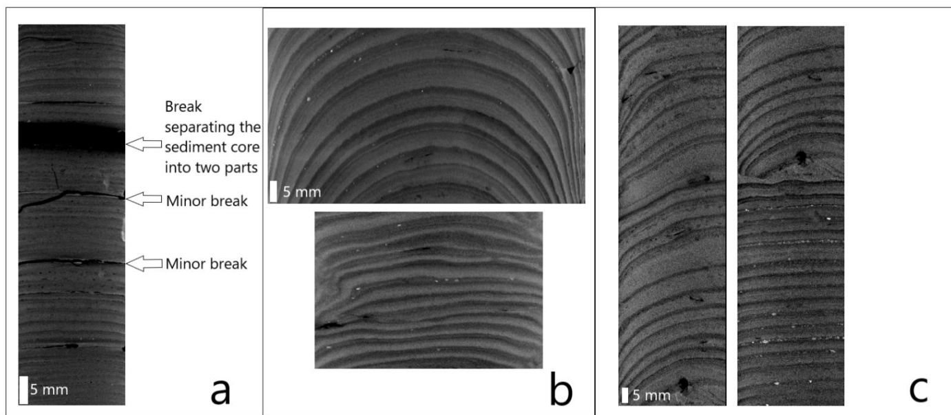
380 Figure 16: (a) The sediment core GL17-01D has broken parts. (b) Deformations are present in the sediment core GL17-05B. (c) The sediment core GL17-04C displays oblique laminations with variable thickness, along with flat and horizontal laminations with constant thicknesses.
