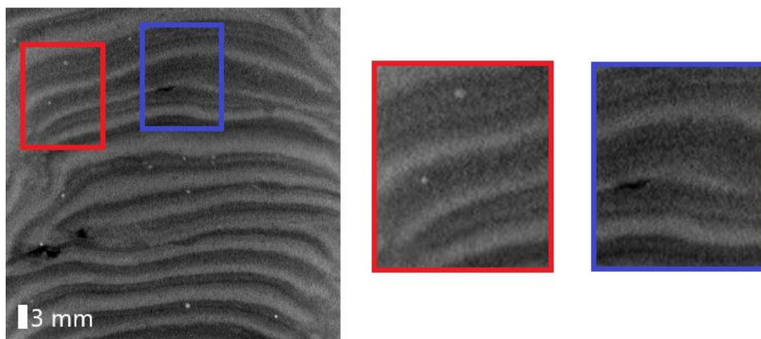
385 Figure 17: Large VOIs allow you to choose where to do more precise scans within small VOIs. The images with red and purple outlines show how the thickness can vary for the same varve.
