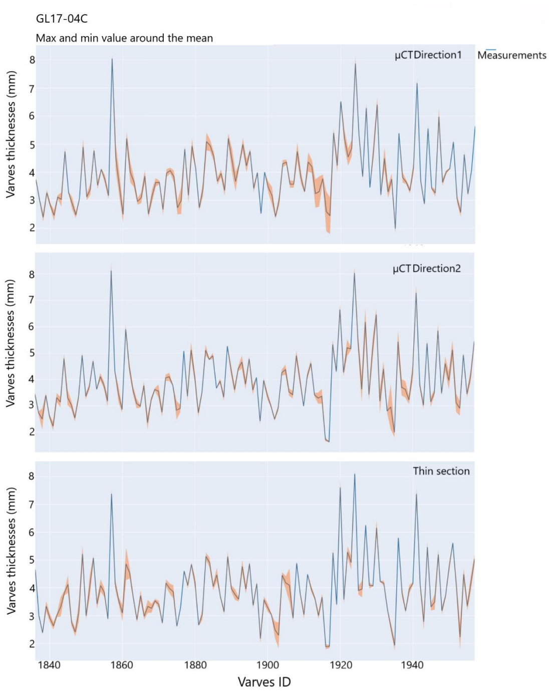
Figure 7: Mean varve thicknesses of the three measurements made in directions 1 (top panels) and 2 (middle panels) using the \mu CT and on thin sections (lower panels) for core GL17-04C. The maximum and minimum values around the mean related to the measurements are shown in the orange shaded area, and the varves ID represents the identification of the varve over an interval.
