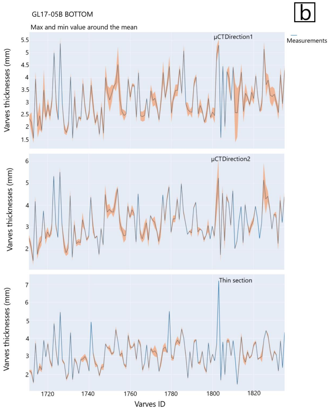
235 Figure 8: Mean varve thicknesses of the three measurements made in directions 1 (top panels) and 2 (middle panels) using the micro-CT and on thin sections (lower panels) for cores GL17-05B at the top (a), and at the bottom (b). The maximum and minimum values around the mean relating to the measurements are in the orange shaded area, and the varves ID represents the identification of the varve over an interval.
