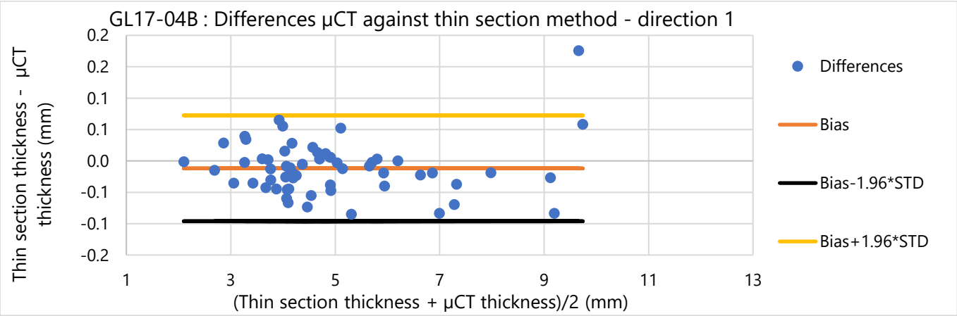
Figure A4: Presentation of the interval in which 95% of the differences between two methods are included. Each blue point represents the result of the difference A_i - B_i between two measurements. The Upper and Lower limits of agreement are the limits of the confidence interval at 95%. The difference A_i - B_i between the two measurement methods is expressed as a function of the mean values (A_i + B_i)/2 of results of the two methods.
