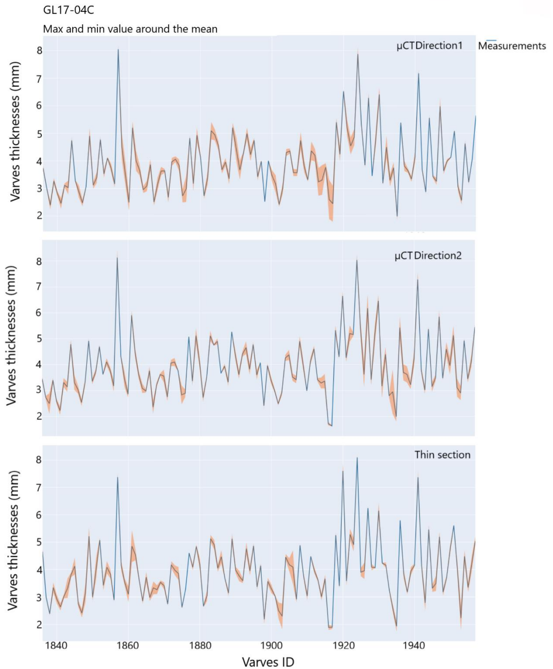
Figure 7: Mean varve thicknesses of the three measurements made in directions 1 (top panels) and 2 (middle panels) using the \mu CT and on thin sections (lower panels) for core GL17-04C. The maximum and minimum values around the mean related to the measurements are shown in the orange shaded area, and the varves ID represents the identification of the varve over an interval.
