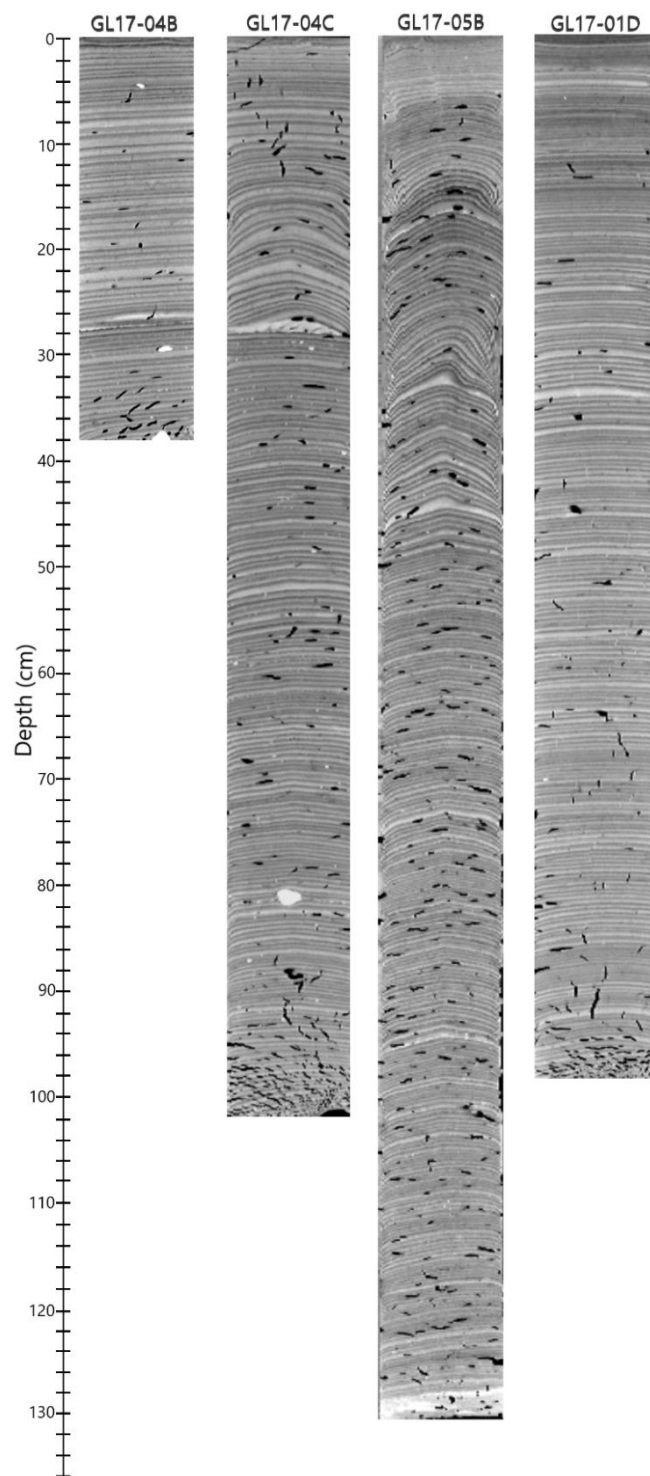
415 Figure A1: CT scan images of the four sediment cores GL17-04B, GL17-04C, GL17-01D and GL17-05B used in this study.
