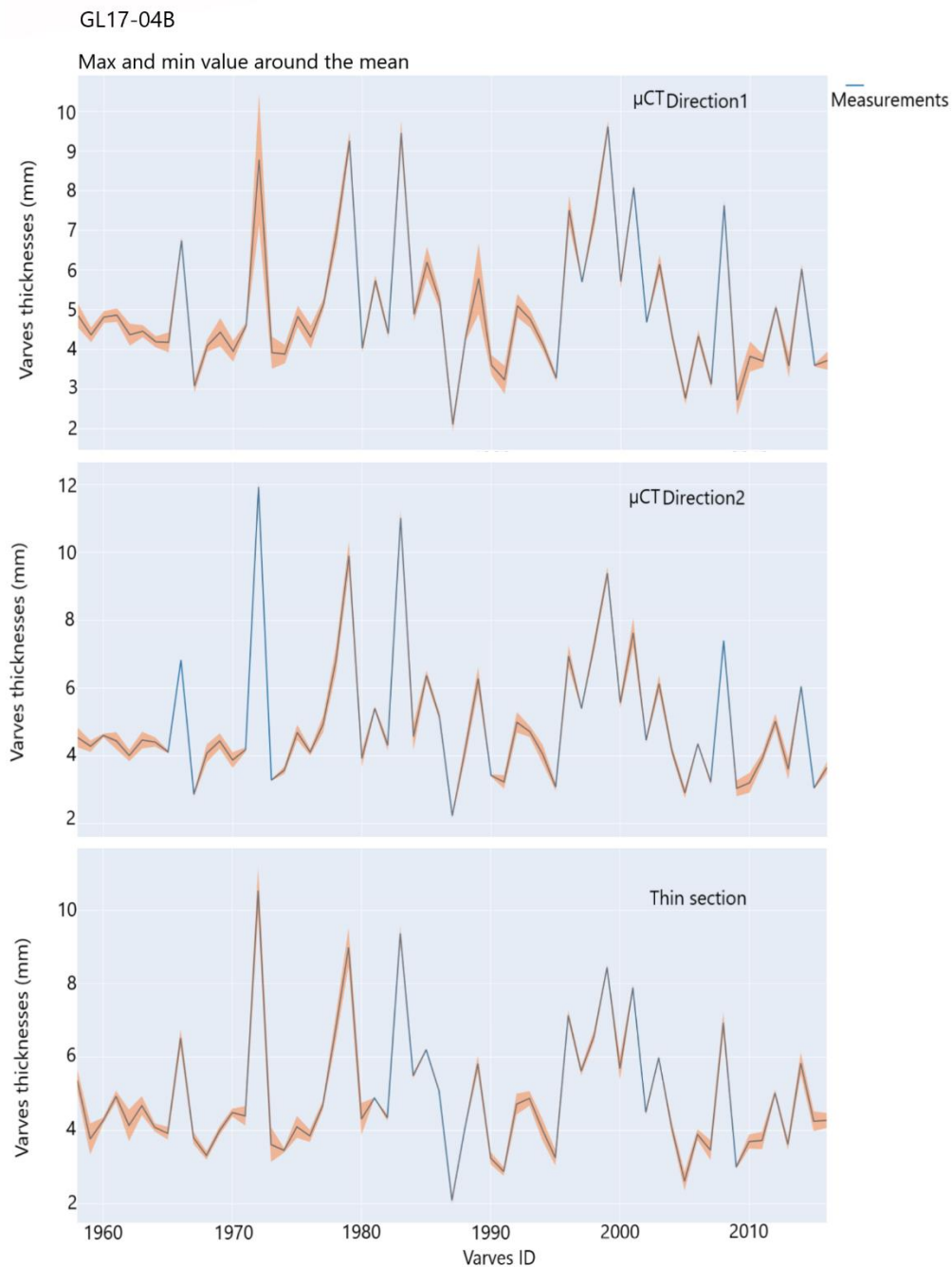
Figure 5: Mean varve thicknesses of the three measurements made in directions 1 (top panels) and 2 (middle panels) using the \mu CT and on thin sections (lower panels) for cores GL17-04B. The maximum and the minimum values around the mean related to the measurements are shown in the orange shaded area, and the varve ID represent the identification of the varve over an interval.
