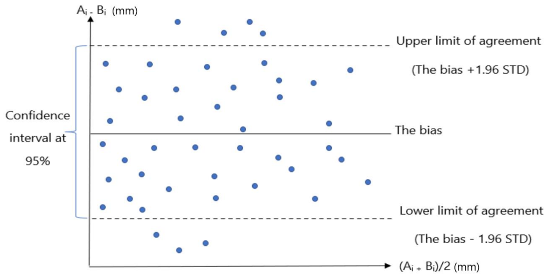
Figure A4: Presentation of the interval in which 95% of the differences between two methods are included. Each blue point represents the result of the difference A_i - B_i between two measurements. The Upper and Lower limits of agreement are the limits of the confidence interval at 95%. The difference A_i - B_i between the two measurement methods is expressed as a function of the mean values (A_i + B_i)/2 of results of the two methods.
