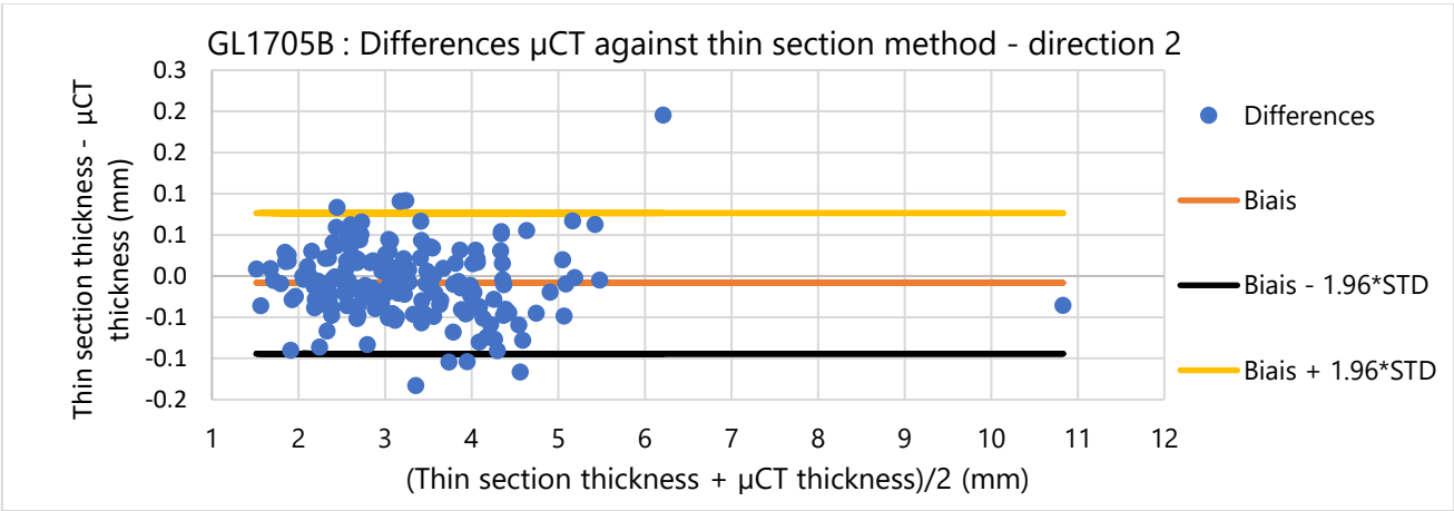
275 Figure 11: Agreement study in direction #2 between the two methods, respectively, on the sediment cores GL17-04B, GL17-01D, GL17-04C, and GL17-05B. The orange line represents the bias, and the two yellow and black lines are the limits of the 95% confidence interval. Note that the vertical axes do not have similar ranges.
