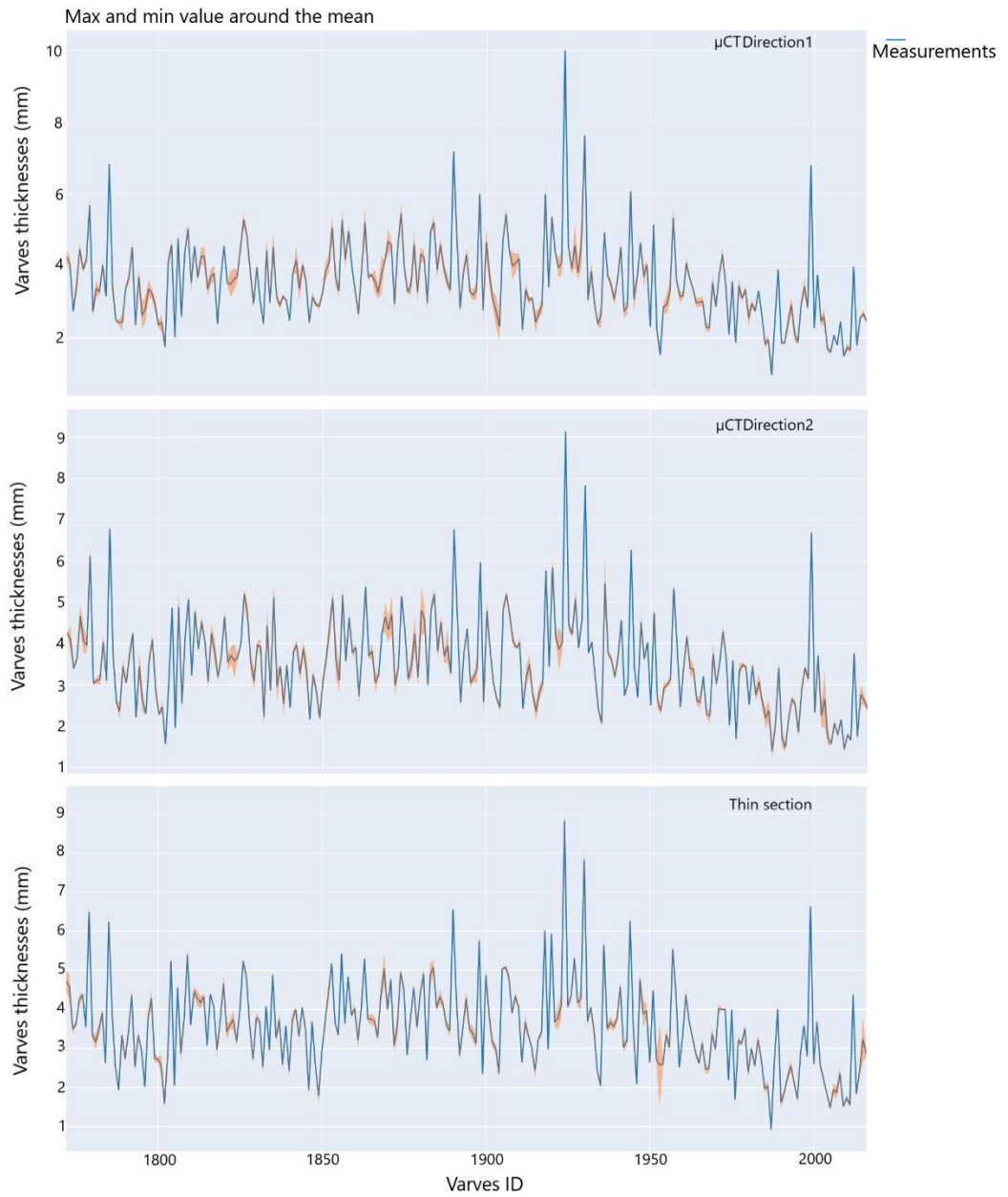
Figure 6: Mean varve thicknesses of the three measurements made in directions 1 (top panels) and 2 (middle panels) using the \mu CT and on thin sections (lower panels) for cores GL17-01D. The maximum and minimum values around the mean relating to the measurements are shown in the orange shaded area, and the varve ID represents the identification of the varve over an interval.
