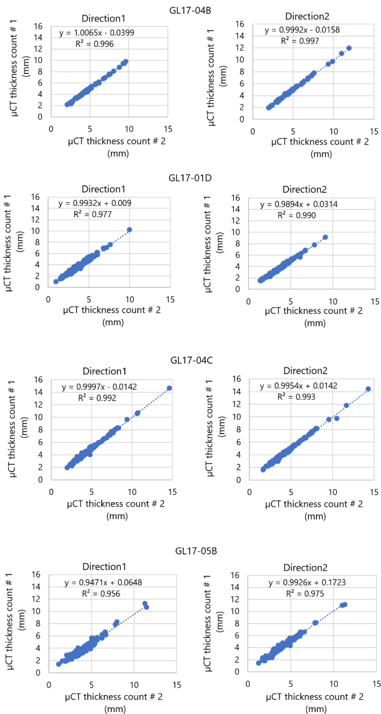
Figure 9: Linear regressions of the mean varve thicknesses measured with \mu CT between directions 1 and 2 for each sediment cores (all measurements are in appendix B).
