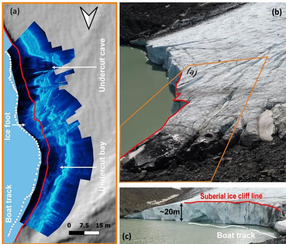
Figure 3. (a) Side scanning sonar (5 th August 2019) plotted over SfM DEM (3 rd August 2019), with red line denoting the top of the subaerial ice front and white dots denoting survey track of the ASV – Note the cave feature near the southern end of the track line (central part of terminus). (b & c) Images of KG looking south across the terminus (3 rd August 2019). Note small crevasse parallel to ice cliff near central portion. Orange inset in (b) denotes area covered by (a).
