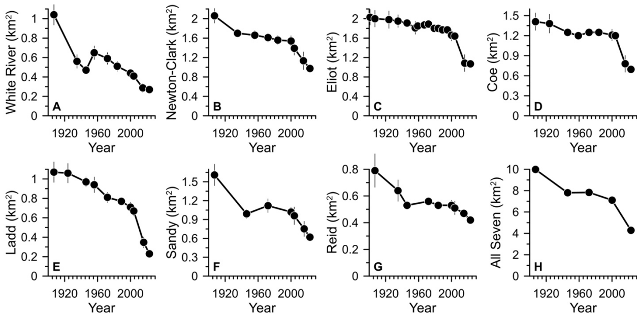
260 Figure 4: Glacier area from 1907 (or 1901 for Eliot Glacier) to 2004 from Jackson and Fountain (2007), 2015 or 2016 from Fountain et al. (2023), and 2023 (new data), with combined area noted in the lower right. Uncertainty noted by vertical bars; note that the uncertainty on the combined record is smaller than the symbol size. A. White River Glacier. B. Newton-Clark Glacier. C. Eliot Glacier. D. Coe Glacier. E. Ladd Glacier. F. Sandy Glacier. G. Reid Glacier. H. Combined record of seven glaciers.
