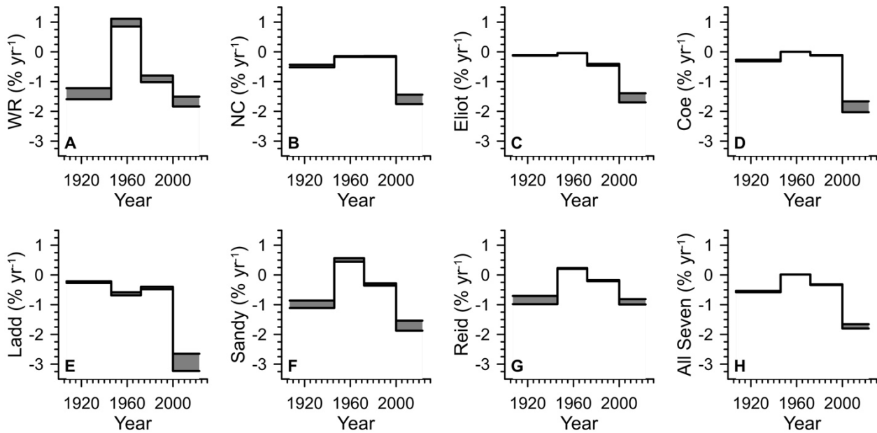
270 Figure 5: Area change with respect to preceding ice area expressed as \% \text{ yr}^{-1} (yr = year) for seven glaciers calculated from Jackson and Fountain (2007) (1907-2000) and 2023 observations, with combined rate in the lower right. Gray shading shows the uncertainty. A. White River (WR) Glacier. B. Newton-Clark (NC) Glacier. C. Eliot Glacier. D. Coe Glacier. E. Ladd Glacier. F. Sandy Glacier. G. Reid Glacier. H. Combined record of seven glaciers.
