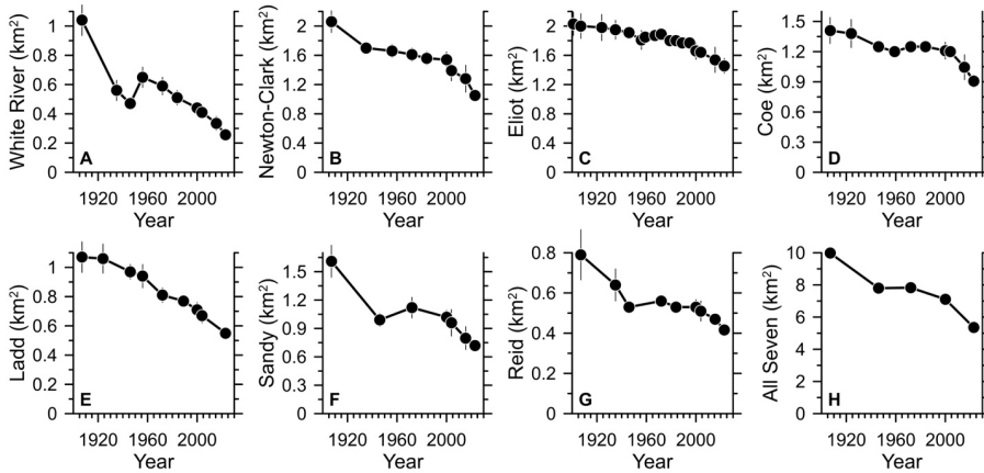
605 Figure 4: Glacier area from 1907 (or 1901 for Eliot Glacier) to 2004 from Jackson and Fountain (2007), 2015 or 2016 from Fountain et al. (2023), and 2023 (new data), with combined area noted in the lower right. Uncertainty noted by vertical bars; note that the uncertainty on the combined record is smaller than the symbol size. A. White River Glacier. B. Newton-Clark Glacier. C. Eliot Glacier. D. Coe Glacier. E. Ladd Glacier. F. Sandy Glacier. G. Reid Glacier. H. Combined record of seven glaciers.
