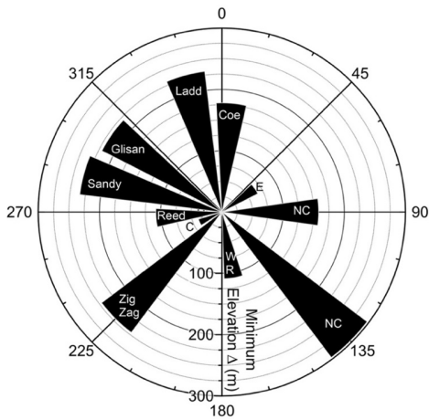
Figure 2: Minimum change ( \Delta ) in the lowest elevation of actively flowing ice from 2003 to 2023 relative to glacier position on Mt. Hood; C = Coalman, WR = White River, NC = Newton-Clark with its two termini labeled, and E = Eliot.
