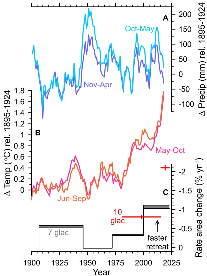
850 855 Figure 7: Hood River County climate change and Mt. Hood glacier area change rate. A. 11-year running mean for change in total October-May (light blue) and November-April (blue) precipitation relative to 1895-1924 average. B. 11-year running mean change in May-October (pink) and June-September (orange) temperature relative to 1895-1924 average. C. Rate of glacier area change for the seven glaciers (glac = glaciers) with records back to 1907 (Jackson and Fountain, 2007) (step plot with gray shading showing the uncertainty) and the rate of area change for 10 glaciers (excludes Ladd and Glisan) between 1981 and 2015/2016 and 2015/2016 and 2023 (Driedger and Kennard, 1986b; Fountain et al., 2023) (red crosses where the length is the period of time covered and the height the uncertainty). Note the inverted axis where faster rate of area loss is oriented up.
