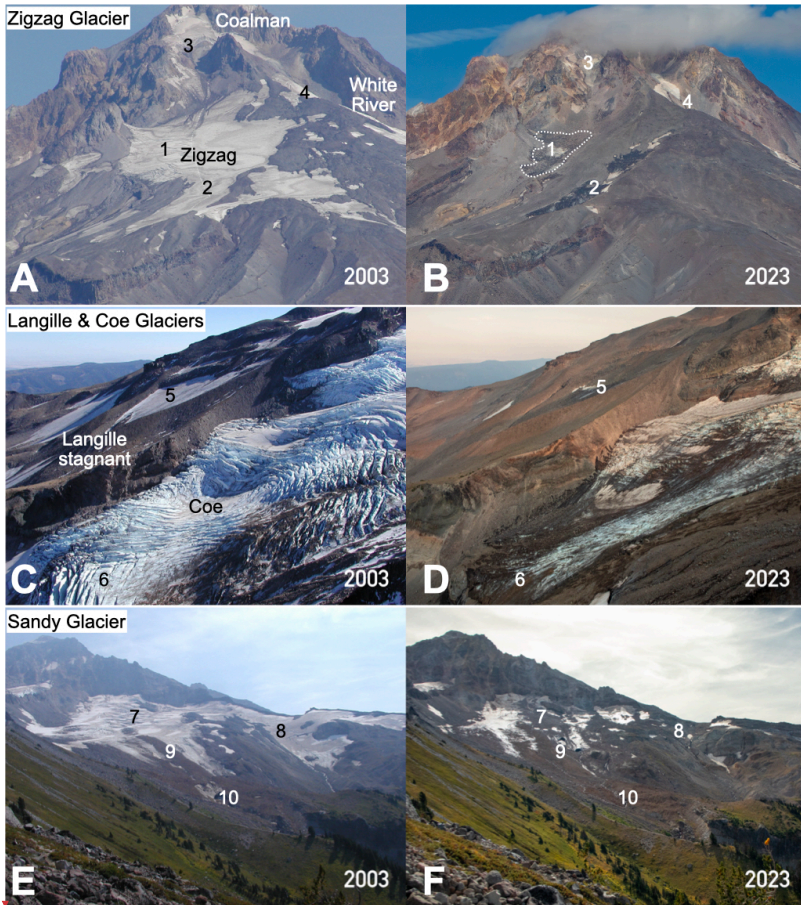
Figure 3: Select repeat photographs from Mt. Hood; see Fig. 1B for photo locations. A and B: Zigzag Glacier across the valley (shot location 45.29275°, -121.80044°) repeat photograph from 2003 (A) and 2023 (B). 1. Denotes the reduction in area of Zigzag Glacier to its 2023 actively flowing limit (dashed white line). 2. Remnant stagnant ice that used to be part of the actively flowing glacier. 3. Western terminus of Coalman Glacier that has retreated but is still visible in 2023 at edge of cloud. 4. Top of White River Glacier that has retracted since 2003. C and D: Langille and Coe Glaciers (shot location 45.39459°, -121.69982°) in 2003 (C) and 2023 (D). 5. Near-complete disappearance of remnant ice of Langille Glacier. 6. Loss of an ice fall on Coe Glacier due to terminus retreat to just below the 6 in D. E and F: Sandy Glacier (shot location 45.39477°, -121.73124°) in 2003 (E) and 2023 (F). 7. Accumulation of rock fall on the glacier in the last 20 years. 8. Retreat of glacier ice that is now exposed bedrock. 9. 2023 terminus location and ice caves (F) that were in the center of the glacier in 2003 (E). 10. 2003 terminus with ice cave (E) that is now stagnant, debris-covered ice (F).
