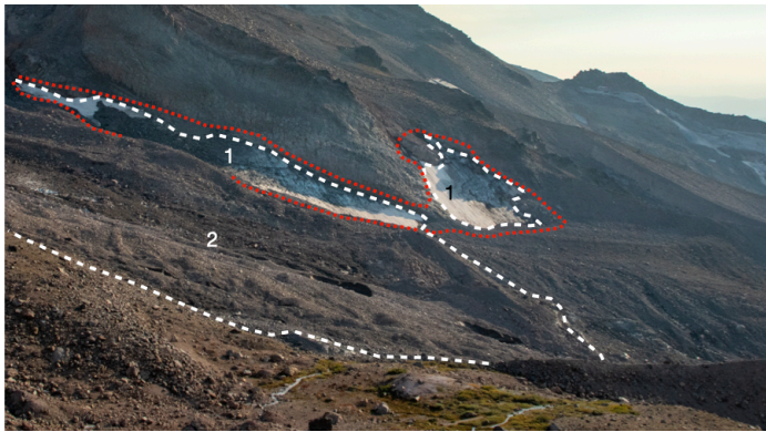
Figure 6: Ladd Glacier terminus in 2023 (see Fig. 1B for photo location). White dashed lines are the 2023 limit while red dotted lines are the 2015/2016 ice limit of Fountain et al. (2023). 1. Notes ice bodies that Fountain et al. (2023) included in Ladd's 2015/2016 area. 2. Debris covered stagnant ice that Fountain et al. (2023) did not include in the 2015/2016 area of the glacier that remained in 2023 and was included in its 2023 limit.
