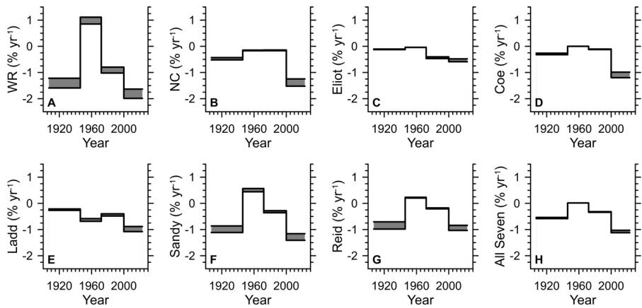
Figure 5: Area change with respect to preceding ice area expressed as % yr -1 (yr = year) for seven glaciers calculated from Jackson and Fountain (2007) (1907-2000) and 2023 observations, with combined rate in the lower right. Gray shading shows the uncertainty. A. White River (WR) Glacier. B. Newton-Clark (NC) Glacier. C. Eliot Glacier. D. Coe Glacier. E. Ladd Glacier. F. Sandy Glacier. G. Reid Glacier. H. Combined record of seven glaciers.
