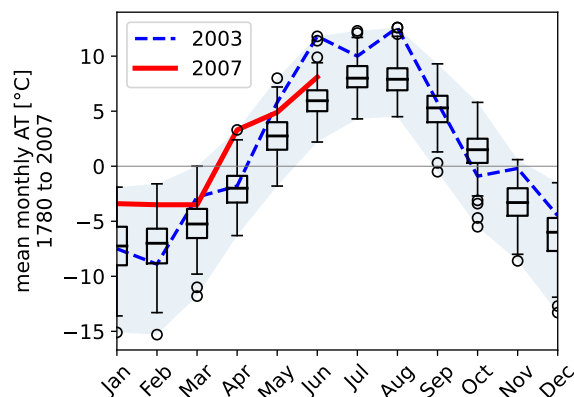
Figure 9. Climatic conditions at the study site during a 228-year record, including monthly temperatures from 1780 to 2007. The shaded area illustrates the range of historic air temperatures for the respective months. The red line illustrates the monthly temperature in 2007 prior to the formation of the rock slide (HISTALP dataset of corresponding 5-minute grid cell, GeoSphere Austria).
