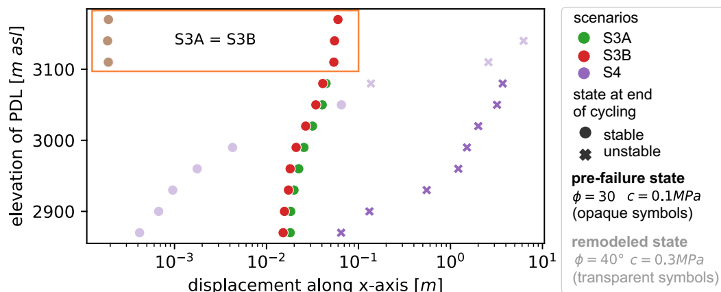
Figure 15. Semi-log plot: x-displacement of monitoring point Rm_x after 10.000 mechanical timesteps for scenarios S3 and S4 versus the elevation of the Polythermal Dividing Line (PDL). The model geometry is according to S1E (see Figure 12), and parameters are assigned according to Figure ???. Results are displayed for shear parameters of discontinuities given in the lower right of the graph. The values represented within the orange box demonstrate that, for the specified elevation of the PDL, there is no discernible difference in x-displacement between scenario S3A and S3B, for both assumed original conditions of discontinuities: the pre-failure and the remodeled state.
