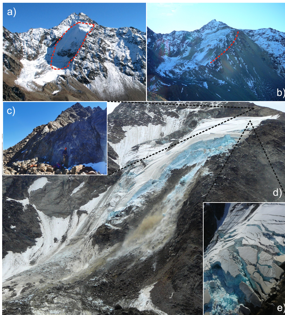
Figure 2. Photographs of the Bliggspitze rock slope taken of the pre-, at- and post-failure stadium showing a) an overview from the Northwest with the Northern Bliggferner glacier in the center - the glacier is divided into an upper and lower section by the rock outcrop in the middle (pre-failure stadium in Summer 2003), b) the post-failure stadium indicated by the fragmented glacier at the top and the sedimentation of debris at the lower part of the glacier (October 2007) - the inferred shear plane is illustrated with a dashed red line in the figure. Debris flows altered the west-facing slope in the years and days previous to the first time formation of the rock slide in June 2007, c) the basal shear zone at the head scarp with polished slickenside and the fragmented rock mass underneath, d) rock and ice falls (secondary processes related to the rock slide: at-failure stadium) and e) the widening of crevasses and fragmentation of glacier ice at the upper section favoring meltwater infiltration into bedrock (at-failure stadium). Dashed black lines indicated the location of more detailed, zoomed-in views. Photographs kindly provided by M. Krautblatter and G. Heißel.
