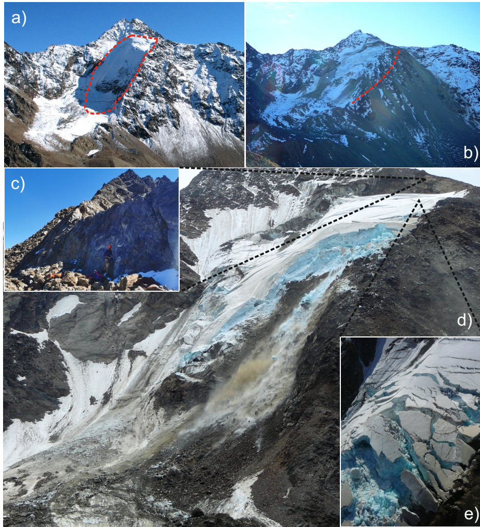
Figure 2. Photographs of the Bliggspitze rock slope taken of the pre-, at- and post-failure stadium-stage showing a) an overview from the Northwest with the Northern Bliggferner glacier-Glacier in the center - the glacier is divided into an upper and lower section by the rock outcrop in the middle (pre-failure stadium-stage in Summer 2003), b) the post-failure stadium-stage indicated by the fragmented glacier at the top and the sedimentation of debris at the lower part of the glacier (October 2007) - the inferred shear plane is illustrated with a dashed red line in the figure. Debris flows altered the west-facing slope in the years and days previous to the first time formation of the rock slide in June 2007, c) the basal shear zone at the head scarp with polished slickenside and the fragmented rock mass underneath, d) rock and ice falls (secondary processes related to the rock slide: at-failure-stadium-sudden-failure stage ) and e) the widening of crevasses and fragmentation of glacier ice at the upper section favoring meltwater infiltration into bedrock ( at-failure-stadium-sudden-failure stage ). Dashed black lines indicated the location of more detailed, zoomed-in views. Photographs kindly provided by M. Krautblatter and G. Heißel. The position and direction of the photographs are indicated in Figure 1, with all photos facing approximately SE.
