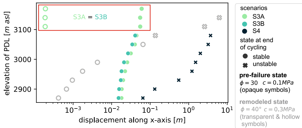
Figure 15. Semi-log plot of x-displacement of monitoring point Rm_x after 10.000 mechanical timesteps for scenarios S3 and S4 versus plotted against the elevation of the Polythermal Dividing Line (PDL). The model geometry is according to S1E (see Figure 12), and parameters are assigned according to Figure 223. Results are displayed for shear parameters of discontinuities given in the lower right of the graph. The values represented within the orange box demonstrate that, for the specified elevation of the PDL, there is no discernible difference in x-displacement between scenario S3A and S3B, for both assumed original conditions of discontinuities: the pre-failure and the remodeled state.
