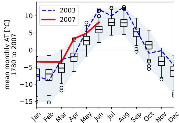
Figure 9. Climatic conditions at the study site during over a 228-year record 227-year period (1780–2007) , including represented by monthly air temperatures from 1780 to 2007. (AT) using boxplots. The boxplots illustrate the distribution of temperatures for each month, highlighting median values, interquartile ranges IQR, whiskers (marked by 1.5·IQR ) and outliers. The shaded area illustrates the range of historic air temperatures for the respective months. The red line illustrates the monthly temperature in 2007 prior to the formation of the rock slide (HISTALP dataset of corresponding 5-minute grid cell, GeoSphere Austria).
