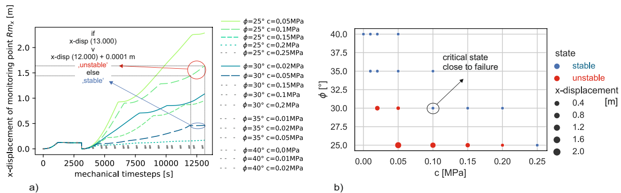
Figure 13. Sensitivity study of shear parameters, attributed to discontinuities in scenario S1 with geometry E, by analyzing the mechanic response by the history of monitoring monitoring point Rm_x . a) Relationship between mechanical timesteps versus x-displacement of the observed grid point for given pairs of shear parameters ("p25c0.05" equals \phi = 25^\circ, c = 0.05MPa ). The given equation checks whether the model reaches equilibrium state at the end of cycling. b) Model states plotted for given pairs of shear parameters as a result of analysis of the x-displacement functions and maximum displacement in the x-direction at the end of cycling. The first 3000 mechanical timesteps show the cycling of the initialized model until reaching equilibrium.
