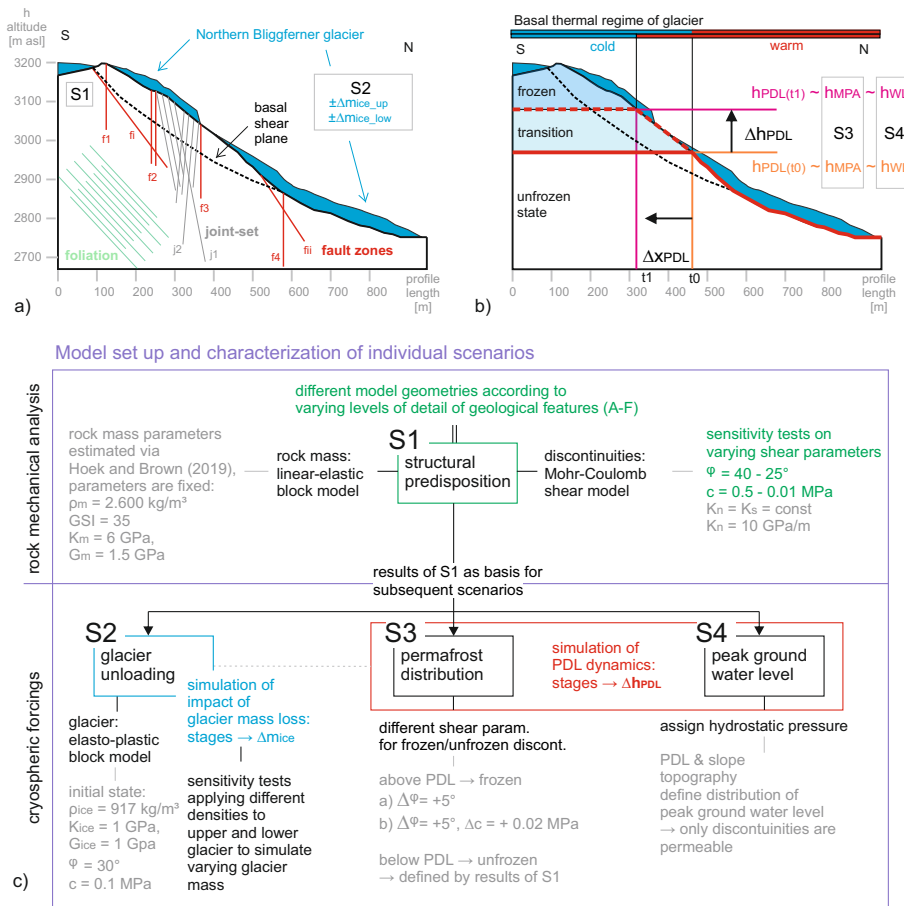
Figure 3. Conceptual scenarios S1 to S4 for investigating rock slope mechanics and interdependencies with environmental forcings in a UDEC model. a) 2D cross-section for the Bliggspitze rock slide, including geological features and glacier extents of upper and lower sections of the Northern Bliggferner Glacier. b) The Polythermal Dividing Line (PDL) marks the border between cold and warm glacier bases in polythermal glaciers. The PDL poses implications on permafrost and water table within the rock mass: The elevation of PDL h_{PDL} at its current state equals the Mountain Permafrost Altitude h_{MPA} and the possible peak groundwater level h_{WL} . c) Description of the UDEC model setup and parameters for simulating the individual scenarios. Abbreviations: S1: \rho_m : density of rock mass, GSI: Geological Strength Index, K_m : bulk modulus of rock mass, G_m : shear modulus of rock mass, \varphi : joint friction angle, c : joint cohesion, K_n : joint normal stiffness, K_s : joint shear stiffness. S2: m_{ice} : mass of glacier ice ( m_{ice\_up/low} refers to the distinctly modeled ice bodies located at the upper or lower part of the slope), \rho_{ice} : density of glacier ice, K_{ice} : bulk modulus of glacier ice, G_{ice} : shear modulus of glacier ice, \phi : internal friction angle of glacier ice, c : cohesion of glacier ice.
