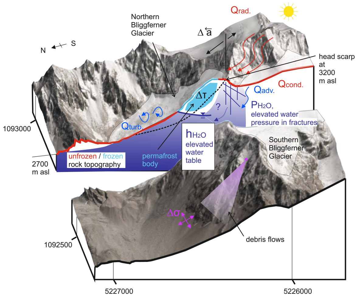
Figure 16. Holistic view on the manifold processes leading to the Bliggspitze rock slope failure. For discussion discussion of individual concepts and abbreviation refer to the text. Various heat transport mechanisms such as Q_{rad.} , radiative heat, Q_{cond.} , conductive heat, Q_{adv.} , advective heat, and Q_{turb.} , turbulent heat, lead to a change in temperature within bedrock \Delta T . Unloading due to loss of glacier/rock mass leads to a change of the stress distribution within the rock mass \Delta\sigma . Both, \Delta T and \Delta\sigma influence local hydrogeology in permafrost rock favoring the buildup of hydrostatic pressure P_{H_2O} within fractures. All of the aforementioned changes (i.e. +\Delta T, -\Delta\sigma, +P_{H_2O} ) negatively affect the mechanical shear strength of geological discontinuities. The thick blue/red lines indicate cold/warm-based glacier conditions. The black dashed line indicates the basal shear plane, while h_{H_2O} illustrates the local water table. \Delta a represents the acceleration of the rock mass triggered by the combined effects described above.
