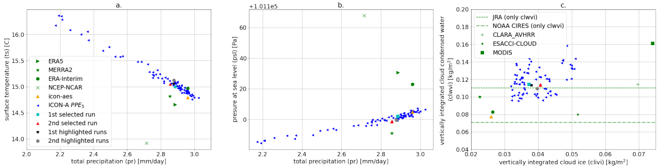
Figure 10. Five evaluation metrics averaged on the 1980-1989 (included) period for the PPE 5 (blue, cyan, red, black, gray), the ICON-aes-1.3 (orange triangle), and reanalysis datasets and observational datasets (green). For the datasets starting after 1980, the time period considered is the earliest available 10 years: for CLARA (AVHRR) and ESACCI CLOUD (AVHRR-fv3.0) it is 1982-1991, for MODIS it is 2002-2011.
