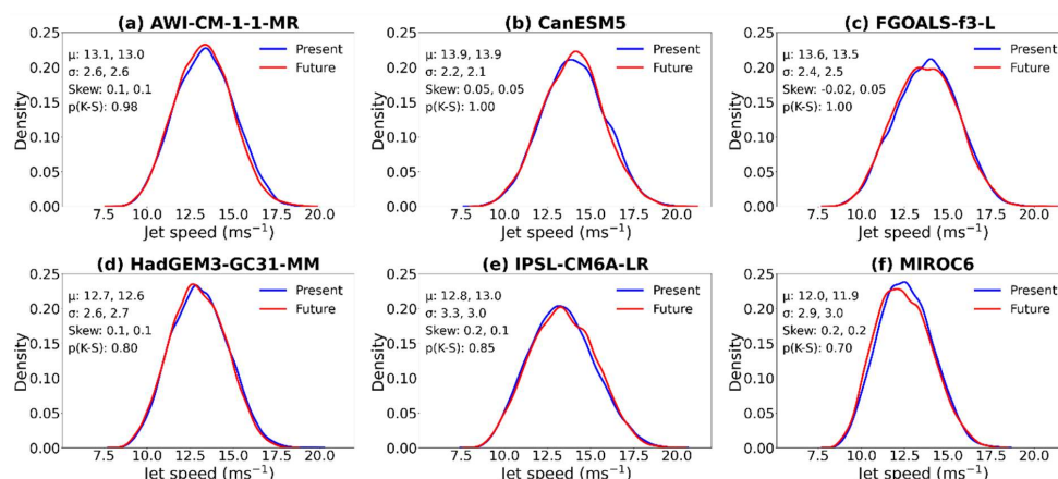
Figure 7: Distributions of daily jet speed in winter for simulations forced by present-day (blue) and future (red) SIC. Data are for the largest mass jet object on each day and distributions have been fitted with a kernel density estimate. Ensemble mean ( \mu ), standard deviation ( \sigma ), skew and K-S test p-value for the distributions are shown in the legend.
