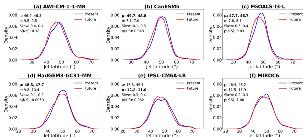
Figure 6: Distributions of daily jet latitude in winter for simulations forced by present-day (blue) and future (red) SIC. Data are for the largest mass jet object on each day and distributions have been fitted with a kernel density estimate. Ensemble mean ( \mu ), standard deviation ( \sigma ), skew and K-S test p-value for the distributions are shown in the legend. Means are bold where the difference between present-day and future simulations is statistically significant based on a t-test at the 95% confidence level. Standard deviations are bold where the difference between time periods is greater than for random sampling.
