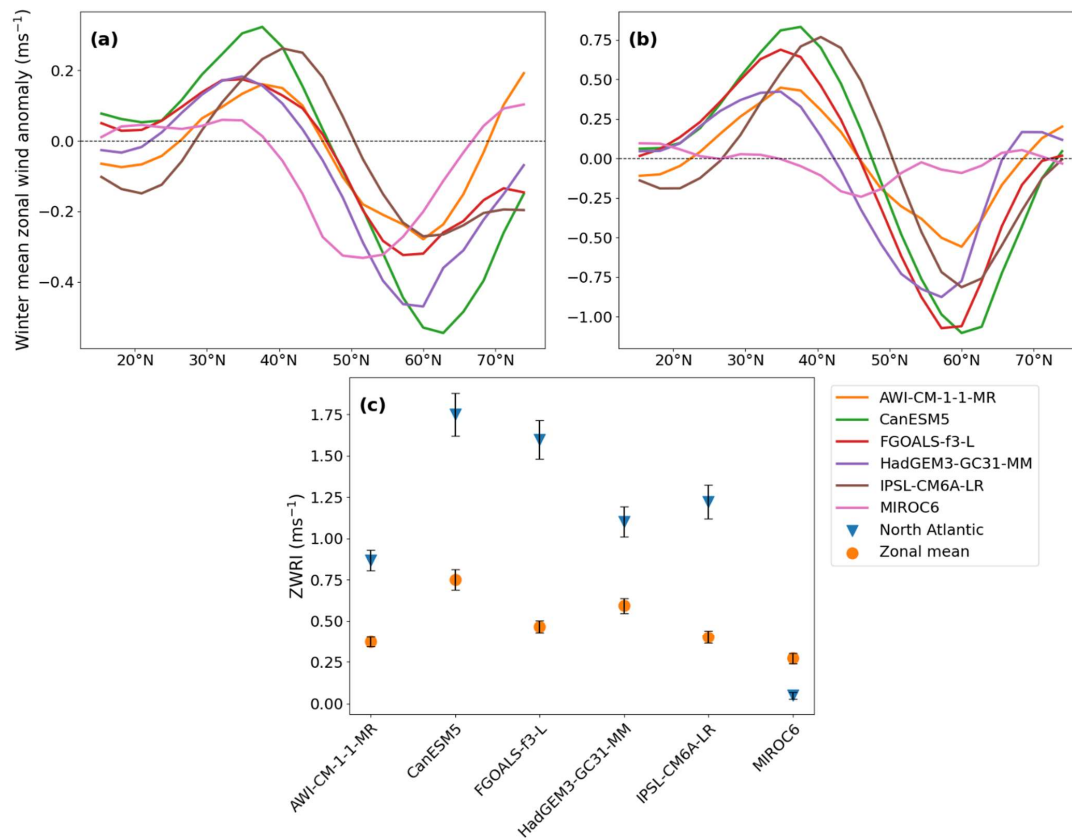
Figure 4: DJF mean U_{850} anomaly due to Arctic sea ice loss in PAMIP models for a) zonal mean and b) North Atlantic (0-60°W) mean. Note the different vertical scales on (a) and (b). (c) the ZWRI of Smith et al. (2022) for the zonal mean (yellow circles) and North Atlantic sector (blue triangles).
