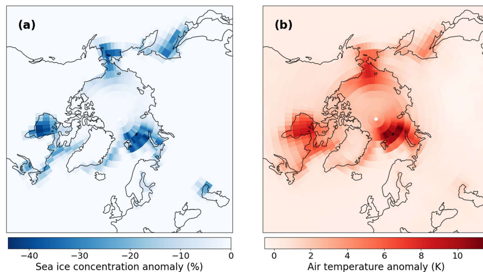
95 Figure 1: DJF multi-model mean difference in (a) SIC and (b) near-surface air temperature between present-day and future PAMIP experiments.
