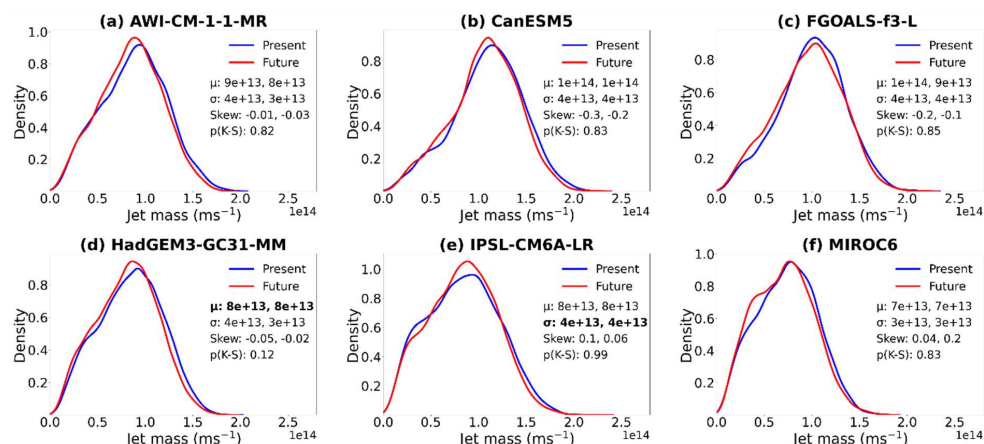
Figure 8: Distributions of daily jet mass in winter for simulations forced by present-day (blue) and future (red) SIC. Data are for the largest mass jet object on each day and distributions have been fitted with a kernel density estimate. Ensemble mean ( \mu ), standard deviation ( \sigma ), skew and K-S test p-value for the distributions are shown in the legend. Means are bold where the difference between present-day and future simulations is statistically significant based on a t-test at the 95% confidence level. Standard deviations are bold where the difference between time periods is greater than for random sampling.
