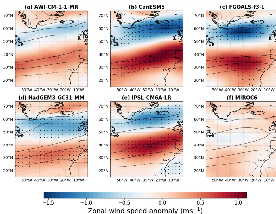
170 Figure 3: DJF ensemble mean U_{850} anomaly in selected PAMIP models between simulations forced by present-day and future SIC. Stippling indicates objects where the difference is significant based on a two-sample Student's t -test at the 95% confidence level. Black contours signify the present-day winter U_{850} climatology at 5 ms -1 intervals with dashed lines showing negative values.
