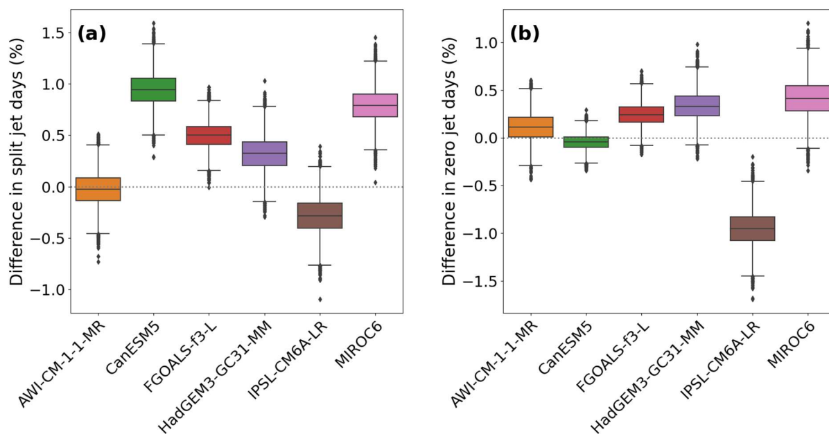
330 Figure 9: Difference in the occurrence of split jet and zero jet days between present-day and future simulations. The percentage of a) split and b) zero jet days are shown between bootstrap resamples of present-day and future ensembles. Coloured boxes
