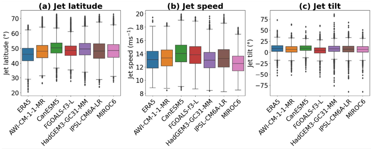
225 Figure 5: Distribution of daily jet features for present-day PAMIP models compared with ERA5 reanalysis. Comparisons shown are for a) jet latitude, b) jet speed and c) jet tilt. Coloured boxes show the interquartile range, the horizontal line shows the median, the whiskers show the overall distributions with diamonds representing outliers.
