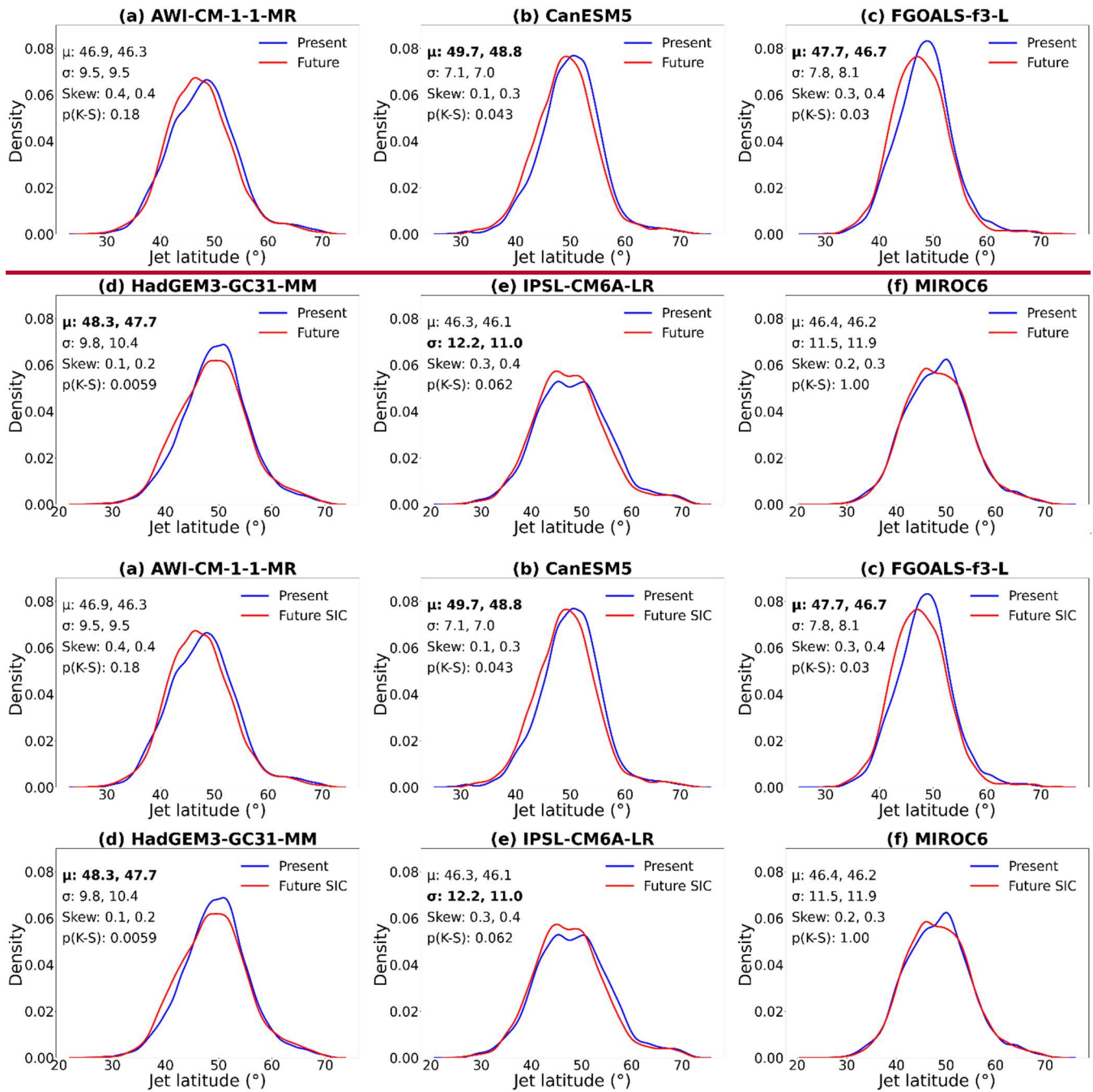
250 Figure 6: Distributions of daily jet latitude in winter for simulations forced by present-day (blue) and future (red) SIC. Data are for the largest mass jet object on each day and distributions have been fitted with a kernel density estimate. Ensemble mean
