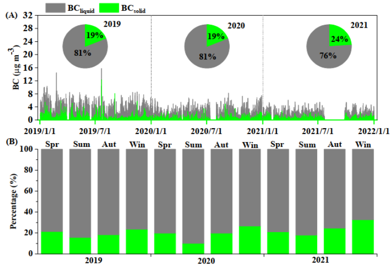
Figure 4 (A) Hourly variation of BC_{liquid} and BC_{solid} , and (B) their relative contribution to BC. The pie charts in (A) are annual average relative contribution of BC_{liquid} and BC_{solid} to BC.
