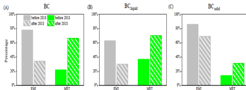
Figure 8 Contributions of Emission Reduction Policies and Meteorological Conditions to the Decrease in BC Concentrations Before and After 2018. The (A), (B) and (C) panels represent BC, BC_{\text{liquid}} and BC_{\text{solid}} .
