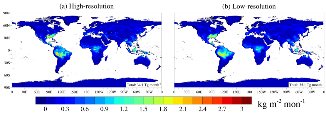
27 Fig. S1 Spatial distribution of isoprene emissions. Shown are results at high- 28 resolution ( 0.25^\circ \times 0.325^\circ ) and low-resolution ( 2^\circ \times 2.5^\circ ) simulations based on Weng et 29 al. (2020).
