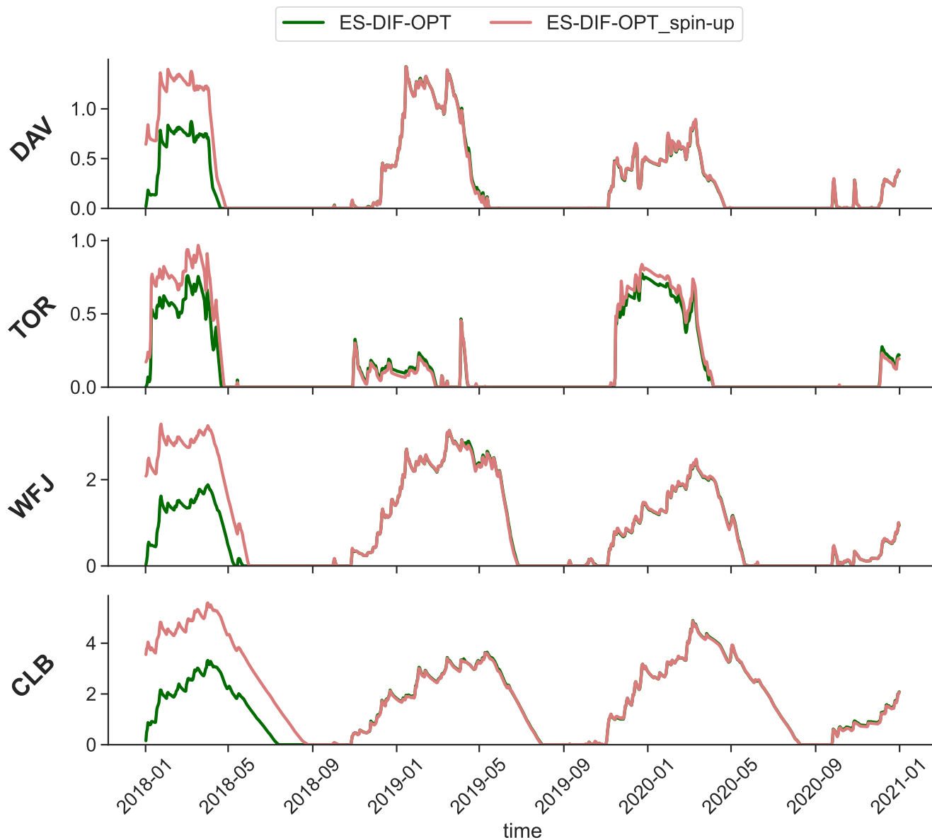
Figure A2. Time series of the snow depth at four sites over the 01/01/2018 to 31/12/2020 using the ES-DIF-OPT configuration, either with the default initialisation field (darkgreen continuous line) or the initialisation field resulting from 13 years of offline spin-up (lightred continuous line).
