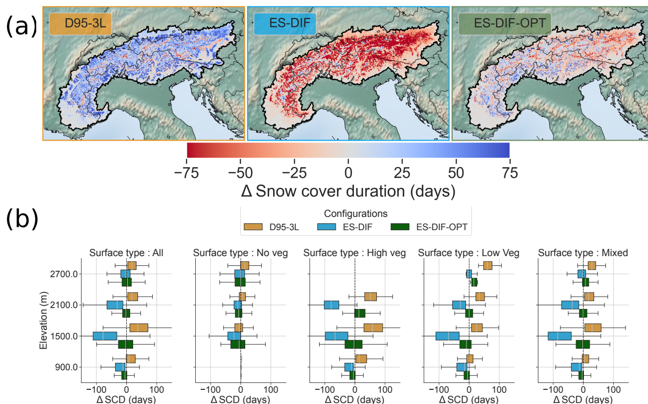
Figure 7. Snow cover duration differences between the simulation results using the different configurations and MODIS observations in the European Alps. Note that MODIS products initially at 500 m horizontal resolution have been regridded over CNRM-AROME horizontal resolution (2.5 km) grid using a first-order conservative method. (a) Map of the average differences (mean error) of the snow cover duration (SCD) over 2 seasons (2018-2019 and 2019-2020) for each configurations compared to MODIS SCD. (b) Boxplot representing the spatial distribution of the average differences (mean error) of the SCD over 2 seasons (2018-2019 and 2019-2020) compared to MODIS SCD for each datasets for the six elevation bands 900 m \pm 150 m, 1500 m \pm 150 m, 1800 m \pm 150 m, 2100 m \pm 150 m, 2400 m \pm 150 m and 2700 m \pm 150 m above sea level. Each column corresponds to the values classified by prevailing type of surface (see section 2.6.2 for details).
