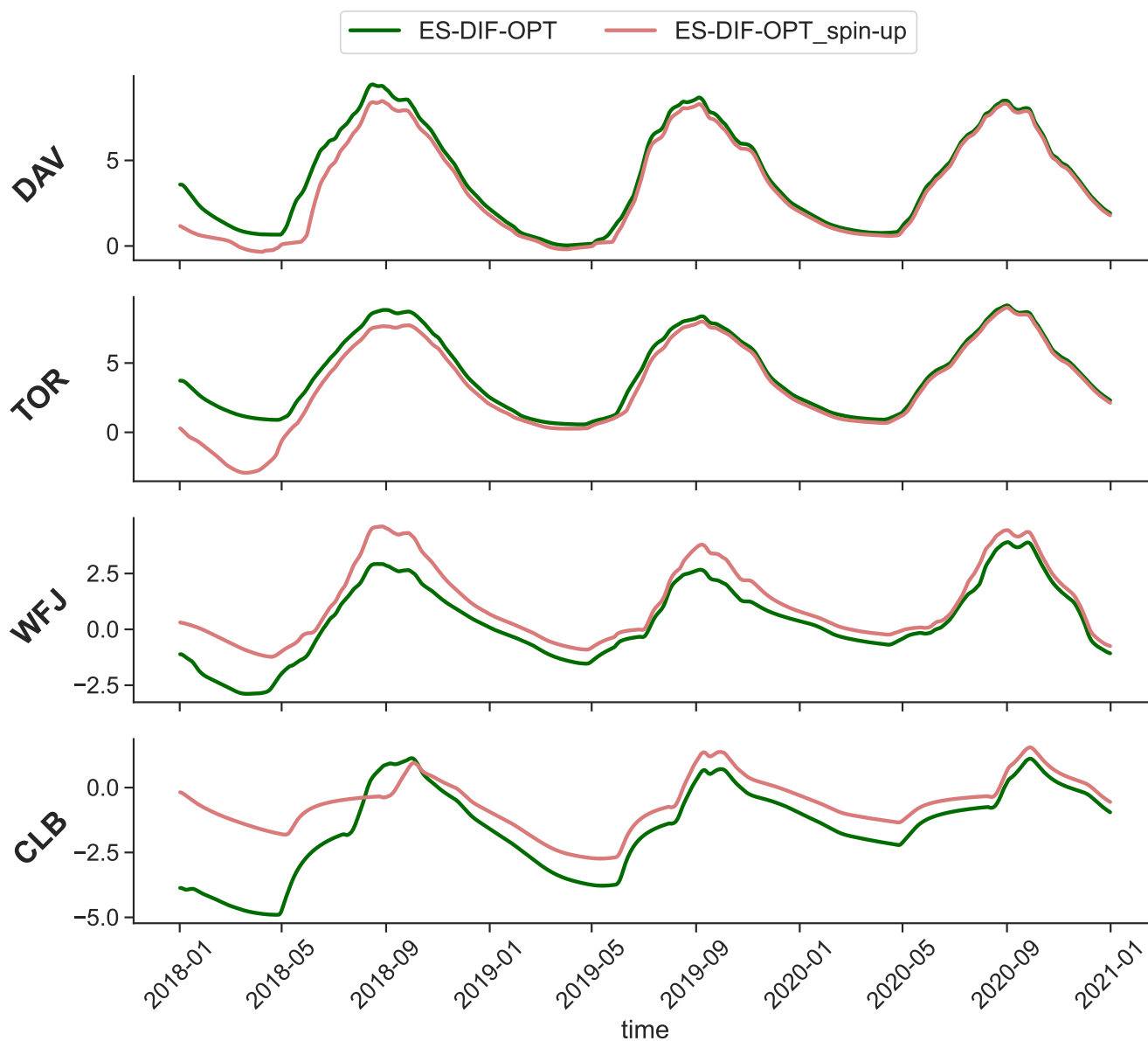
Figure A4. Time series of the soil temperature at 2 m below surface at four sites over the 01/01/2018 to 31/12/2020 using the ES-DIF-OPT configuration, either with the default initialisation field (darkgreen continuous line) or the initialisation field resulting from 13 years of offline spin-up (lightred continuous line).
