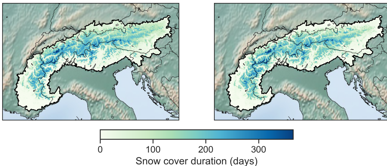
Figure 4. MODIS Snow Cover Duration (SCD) over 2 seasons (2018-2019 and 2019-2020) within the contour of the Alpine convention, regridded at 2.5 km horizontal resolution over the CNRM-AROME mesh grid.
