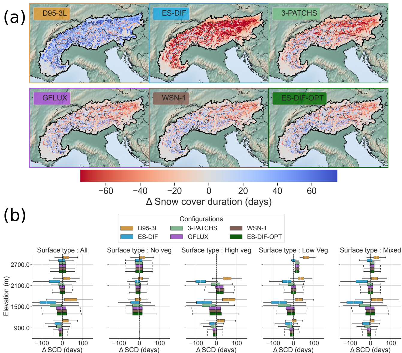
Figure B2. Snow cover duration differences between the different configurations and MODIS observations in the European Alps. Note that MODIS products initially at 500 m horizontal resolution have been regridded over CNRM-AROME horizontal resolution (2.5 km) grid using a first-order conservative method. (a) Map of the average differences (mean error) of the snow cover duration (SCD) over 2 seasons (2018-2019 and 2019-2020) for each configurations compared to MODIS SCD. (b) Boxplot representing the spatial distribution of the average differences (mean error) of the SCD over 2 seasons (2018-2019 and 2019-2020) compared to MODIS SCD for each datasets for six elevation bands of 300 m (900 m \pm 150 m, 1500 m \pm 150 m, 1800 m \pm 150 m, 2100 m \pm 150 m, 2400 m \pm 150 m and 2700 m \pm 150 m). Each column corresponds to the values classified by prevailing type of vegetation (see section 3.2 for details).
