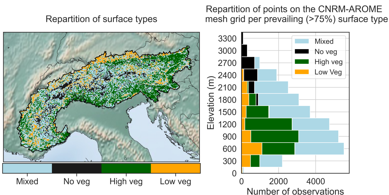
Figure 5. Location of the prevailing surface type (i.e. if the surface type represents more than 75% of the cover, otherwise is it classified as "mixed") for the CNRM-AROME mesh grid within the contour of the Alpine convention. The horizontal barplot on the right shows the number of grid points per bins of 300 m width elevation bands, classified by prevailing surface type.
