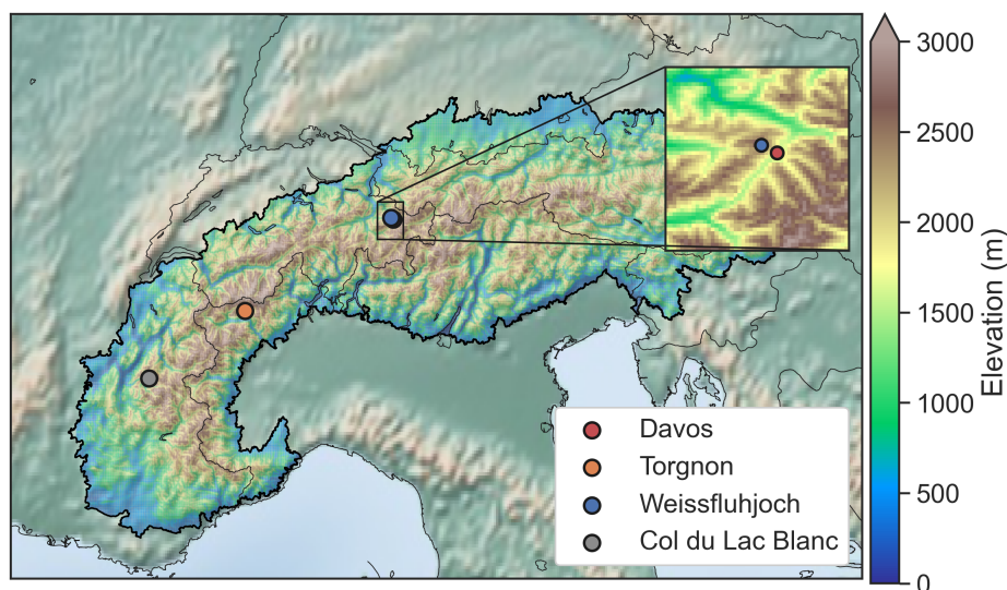
Figure C1. Location of the well instrumented in-situ stations together with the digital elevation model at 1 km horizontal resolution
