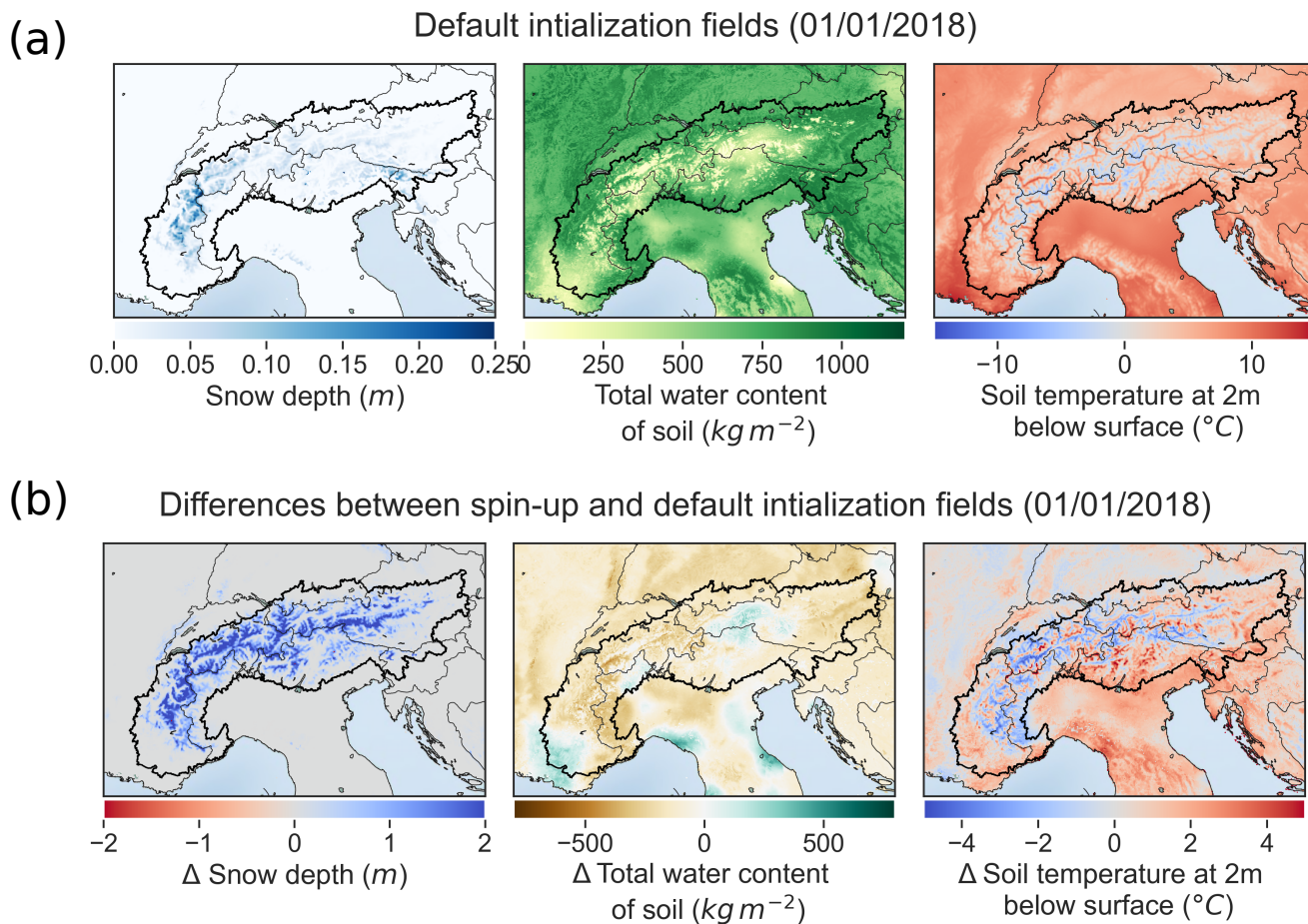
Figure A1. (a) Maps of the snow depth, the total water content of soil and the soil temperature at 2 m fields of our experiments at the initialisation date (01/01/2018) using the default initialisation procedures. (b) Maps of the differences between the default initialisation procedures and the initialisation resulting from 13 years of offline spin-up for the snow depth, the total water content of soil and the soil temperature at 2 m fields at the initialisation date (01/01/2018).
