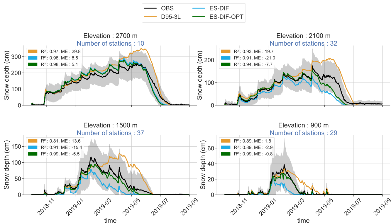
Figure 6. Multi-stations average time series of snow depth values for the 2018-2019 winter for the four elevation bands centered at 900\text{ m} \pm 150\text{ m} , 1500\text{ m} \pm 150\text{ m} , 2100\text{ m} \pm 150\text{ m} and 2700\text{ m} \pm 150\text{ m} above sea level. Colored continuous lines correspond to the simulated multi-stations average time series for each of the configuration : D95-3L in orange, ES-DIF in blue and ES-DIF-OPT in green. Black circle markers correspond to the multi-stations mean time series of the in-situ measurements with the inter-stations standard deviation represented in gray shaded areas. For each elevation bands, the number of stations used to compute the mean and the standard deviation are displayed in blue font. At each elevation bands and for all configurations, the correlation ( R^2 ) and the mean error ( ME ) computed using the multi-station time series between the simulated and the in-situ measurements are displayed.
