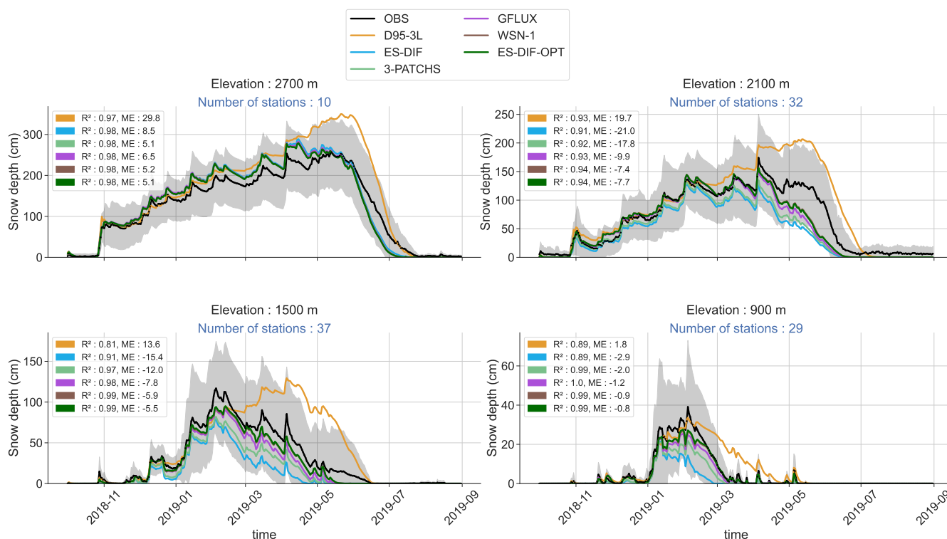
Figure B1. Multi-stations mean time series of the height of snow for the 2018-2019 winter for four elevation bands of 300 m ( 900\text{ m} \pm 150\text{ m} , 1500\text{ m} \pm 150\text{ m} , 2100\text{ m} \pm 150\text{ m} and 2700\text{ m} \pm 150\text{ m} ). Colored continuous lines corresponds to the simulated multi-stations mean time series for each of the configuration. Black lines with circle markers correspond to the multi-stations mean time series of the in situ measurements with the inter-stations standard deviation represented in gray shaded areas. For each elevation bands, the number of stations used to construct the mean and the standard deviation are displayed in blue font. At each elevation bands and for all configurations, the correlation ( R^2 ) and the mean error (ME) computed using the multi-mean time series between the simulated and the in-situ measurements are displayed.
