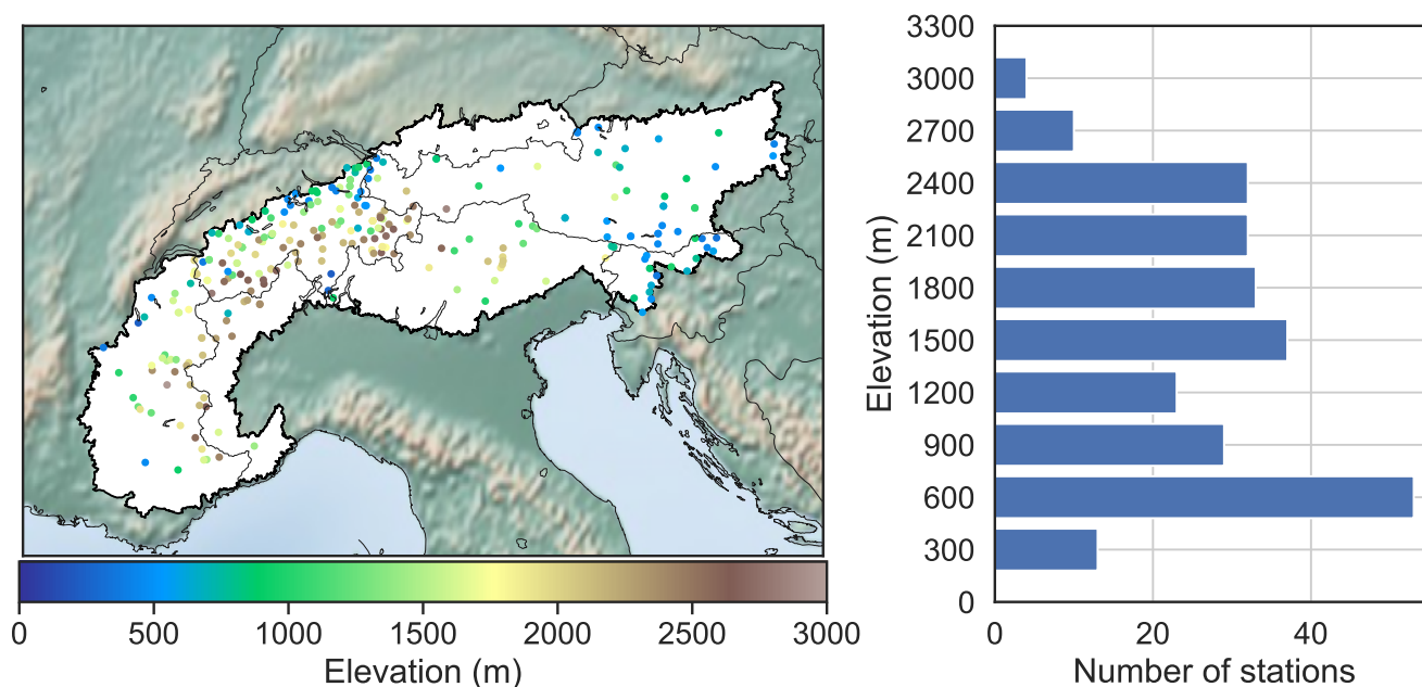
Figure 3. Location of the in-situ snow depth observations with their associated number per bins of 300 m width elevation bands.
