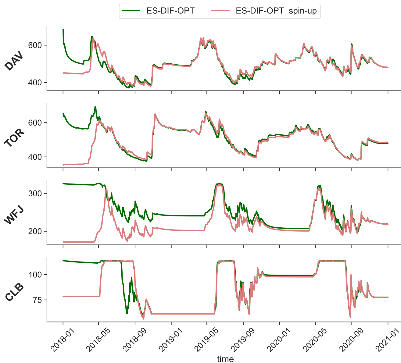
Figure A3. Time series of the total soil water content at four sites over the 01/01/2018 to 31/12/2020 using the ES-DIF-OPT configuration, either with the default initialisation field (darkgreen continuous line) or the initialisation field resulting from 13 years of offline spin-up (lightred continuous line).
