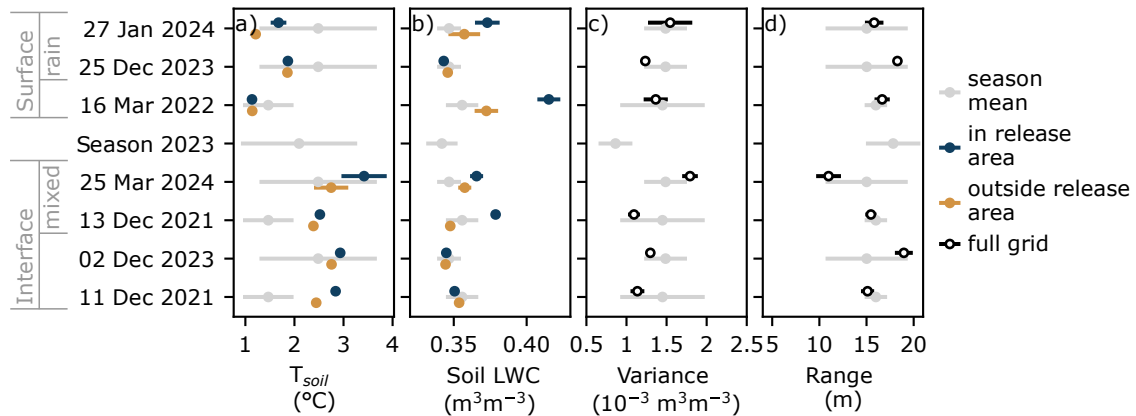
Figure 7. Comparison of average the soil properties before avalanche release with the season mean (gray) sorted by the source of interfacial water. The mean soil properties were calculated as the mean across the sensors by group and all snow-covered time-steps within 8 days before avalanche release. For rain-on-snow events the average was calculated from the start of the rain to the time of avalanche release. The season mean was calculated across all sensors and snow-covered measurements recorded between 15 Oct and 15 Apr. The standard deviation refers to the temporal distribution of mean sensor measurements. The a) soil temperature and b) soil LWC were separated in sensors in (blue) and outside (yellow) the release area. The spatial distribution of the soil LWC was quantified across the entire grid (black) using c) the soil LWC variance and d) the soil LWC range (Appendix A). The average for the avalanche events was calculated for the snow-covered time-periods 8 days before avalanche release. For rain-on-snow events the average was calculated from the start of the rain to the time of avalanche release.
