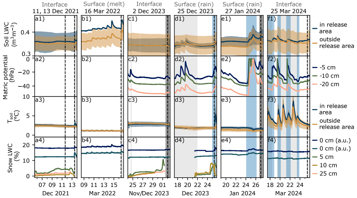
Figure 6. Soil and snow properties before glide-snow avalanche release: events are separated in columns (a-f) and the rows (1-4) show the measurements starting throughout the 8 days before avalanche release (a-f). The background color indicates a patchy (gray), continuous (white) snow cover, or rain (blue). The dashed line indicates the time of avalanche release in the Seewer Berg slope with the range of uncertainty in dark gray. Results from sensor groups (in/outside release area) are visualized as the mean (line) and standard deviation (shading) between the sensors within the group. The parameters include: _1) the soil LWC separated between for sensors that were located in the avalanche release area (orange/blue) and the remaining sensors in the grid outside (blue/yellow) the release area. _2) The soil matric potential - which was recorded since summer 2022. _3) The soil temperature shown separately for the sensors that were located in (blue) and outside (yellow) the avalanche release area and the remaining sensors. _4) The snow LWC sensors at three heights and the interface sensors (in arbitrary units) and at three snow heights. When there are no measurements available (b4, e4, f4) this was due to insufficient snow heights which caused preferential melt around the wedges.
