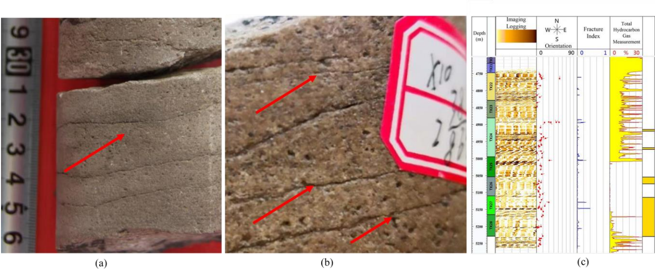
195 Figure 2 The evidence for the horizontal fractures in the area. Figure 2a and 2b are cores with developed horizontal fractures (The red arrows point to the horizontal fractures.). Figure 2c is the imaging logging of the horizontal fracture formation.
