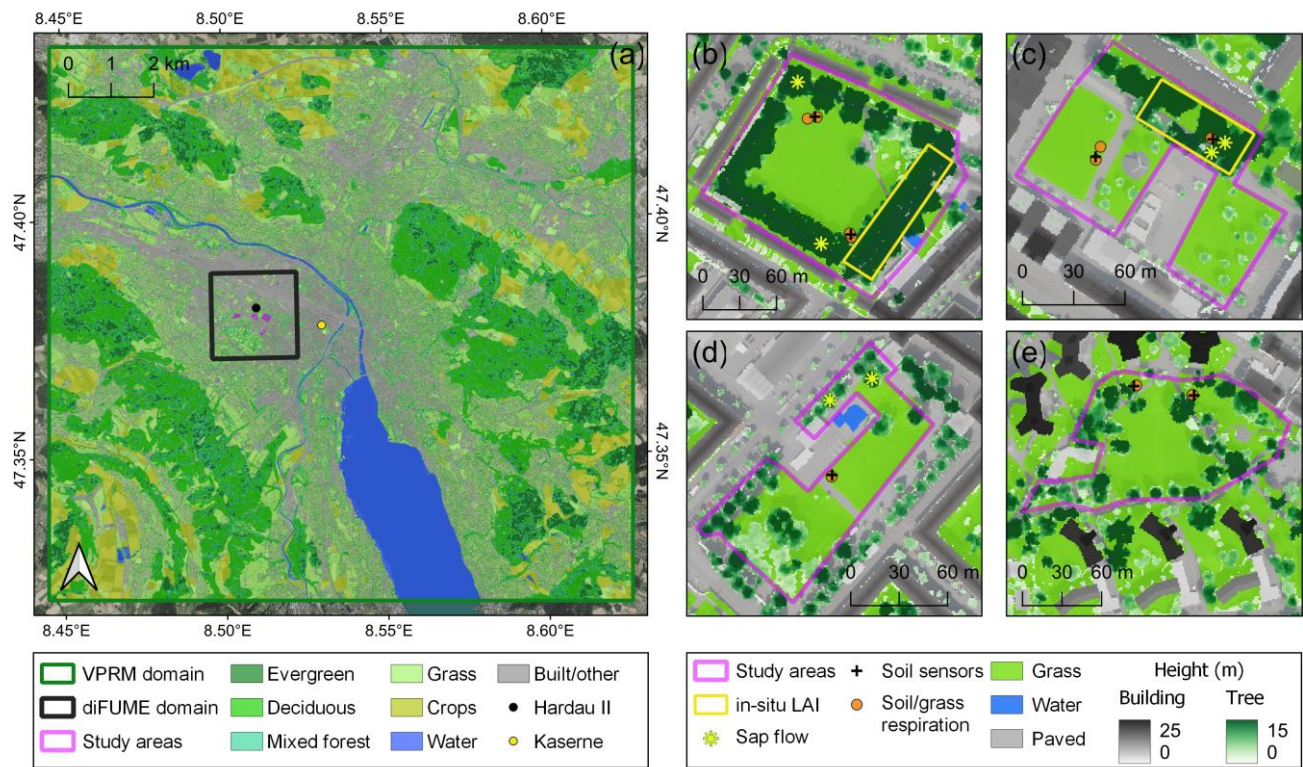
145 Figure 1: (a) Locations of the study areas, meteorological stations (Hardau II, Kaserne) and the model domains over the land cover map of the Zurich region. Locations of the in-situ observations in (b) Bullingerhof, (c) Hardaupark, (d) Fritschwiese, and (e) Heiligfeld parks over the land cover map and with the building and tree heights overlaid. All maps are projected in the Swiss CH1903+LV95 coordinate system (EPSG: 2056) in a semi-transparent format over a basemap of aerial orthophotos (Orthofoto, 2024).
