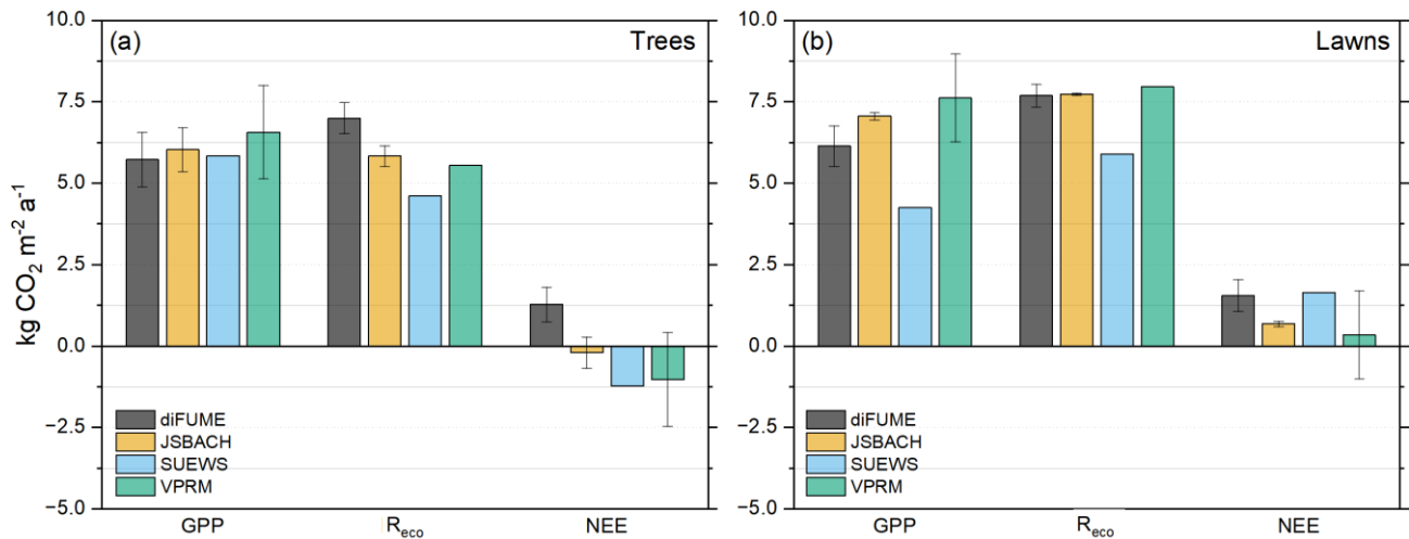
Figure 5. Annual totals for gross primary production (GPP), ecosystem respiration ( R_{eco} ) and net ecosystem exchange (NEE) for (a) trees and (b) lawns of the study parks. The whiskers express the standard deviation between the four parks. The period used to estimate the totals is between July 2022 and June 2023.
