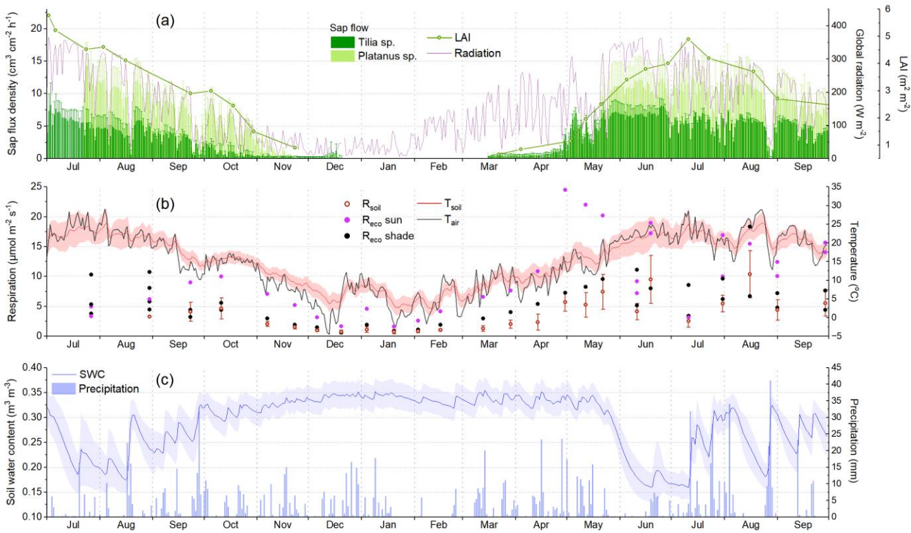
450 Figure 2. Time-series of the in-situ observations in the study parks (Fig. 1) during the campaigns from May 2022 to Sep 2023. (a) Average leaf area index (LAI) from the two Platanus sp. stands, daily averages and standard deviations of the sap flux densities per tree species and daily average incoming global radiation. (b) Average and standard deviation of the measured soil respiration ( R_{soil} ), measured lawn ecosystem respiration ( R_{eco} ) (sunny and shaded locations in different colour) and daily average air and soil temperatures where the shading refers to the standard deviation of the seven soil sensors. (c) Daily average (line) and standard deviation (shade) of the measured soil water content (SWC) and daily precipitation (bars). 455
