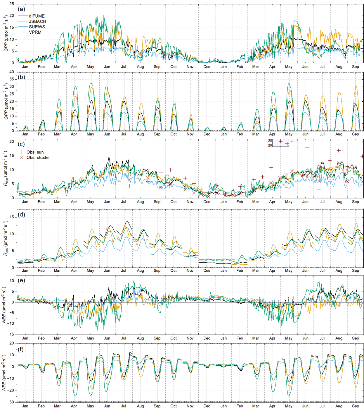
Figure 4. Time-series of model outputs for park lawns (averages of the four parks). Daily averages of (a) gross primary production (GPP), (c) ecosystem respiration ( R_{\text{eco}} ) and (e) net ecosystem exchange (NEE) estimates and diurnal hourly averages per month of
