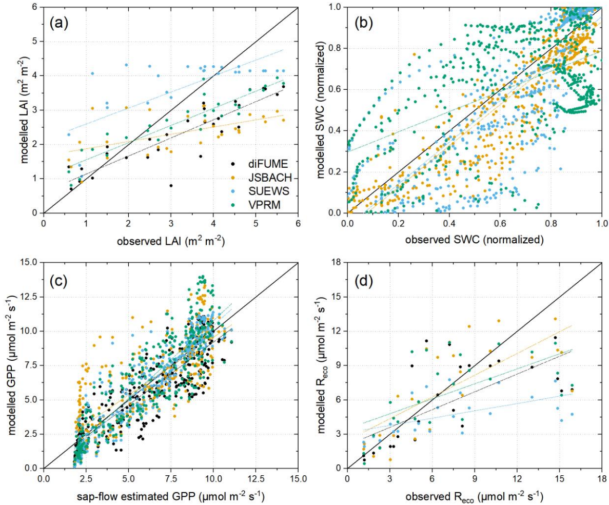
Figure B2. Scatterplots between (a) observed and modelled tree leaf area index (LAI, b) normalised observed and modelled soil water content (SWC) of lawns, (c) observed and modelled tree gross primary production (GPP), and (d) observed and modelled lawn ecosystem respiration ( R_{\text{eco}} ). The 1:1 lines are thick black lines and the linear fits for each model are presented with the respective colour. The evaluation metrics of the comparisons are presented in the Taylor diagram (Fig. 6). For the conversion of VPRM EVI to LAI, VPRM LSWI to SWC and tree sap flow observations to tree GPP, see Section 2.5.
