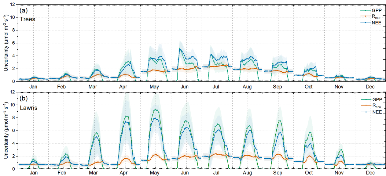
610 Figure 7. Monthly diurnal hourly averages (dots) and standard deviations (shading) of the estimated GPP, R_{\text{eco}} and NEE uncertainties, for (a) park trees and (b) lawns. The monthly averages consider the years 2022 and 2023 together.
