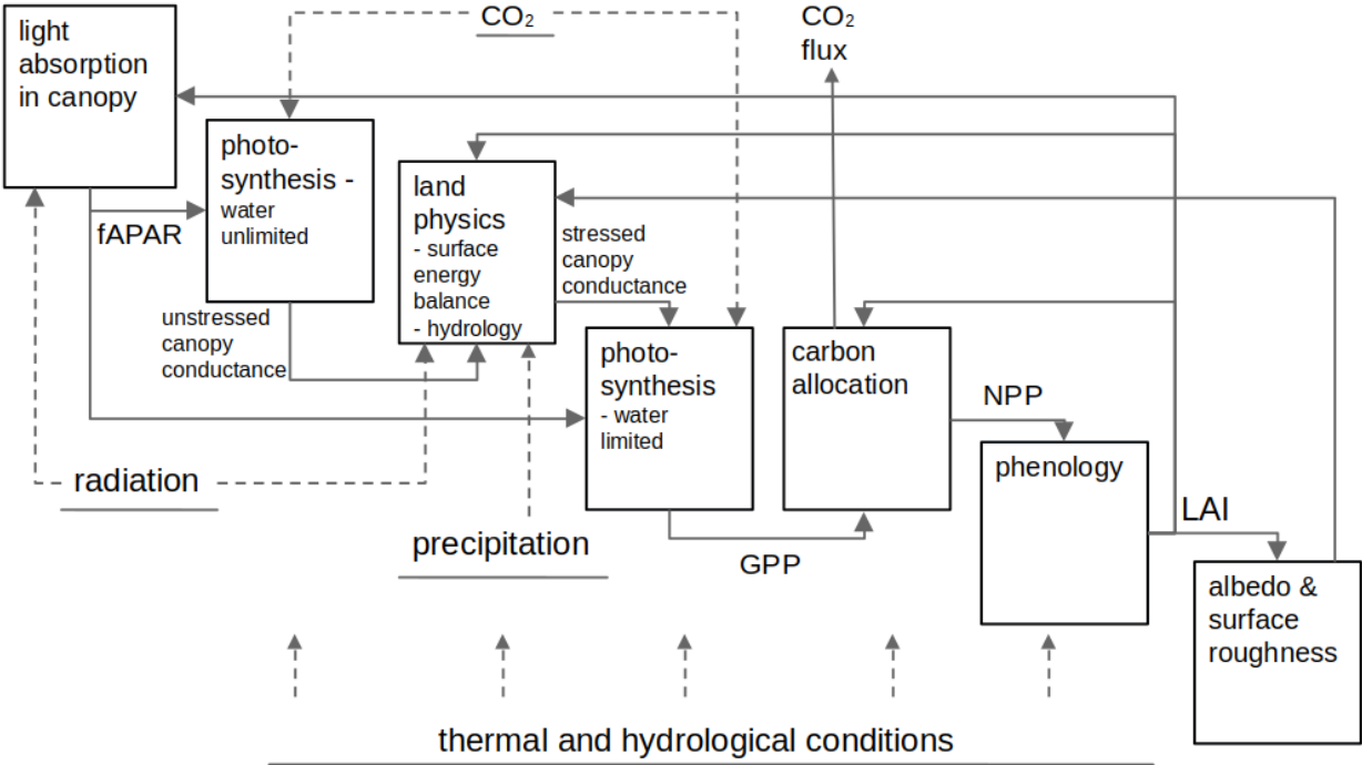
Figure A1. Process flow diagram of the diFUME model. The detailed description of the model can be found in Stagakis et al. (2023a).
