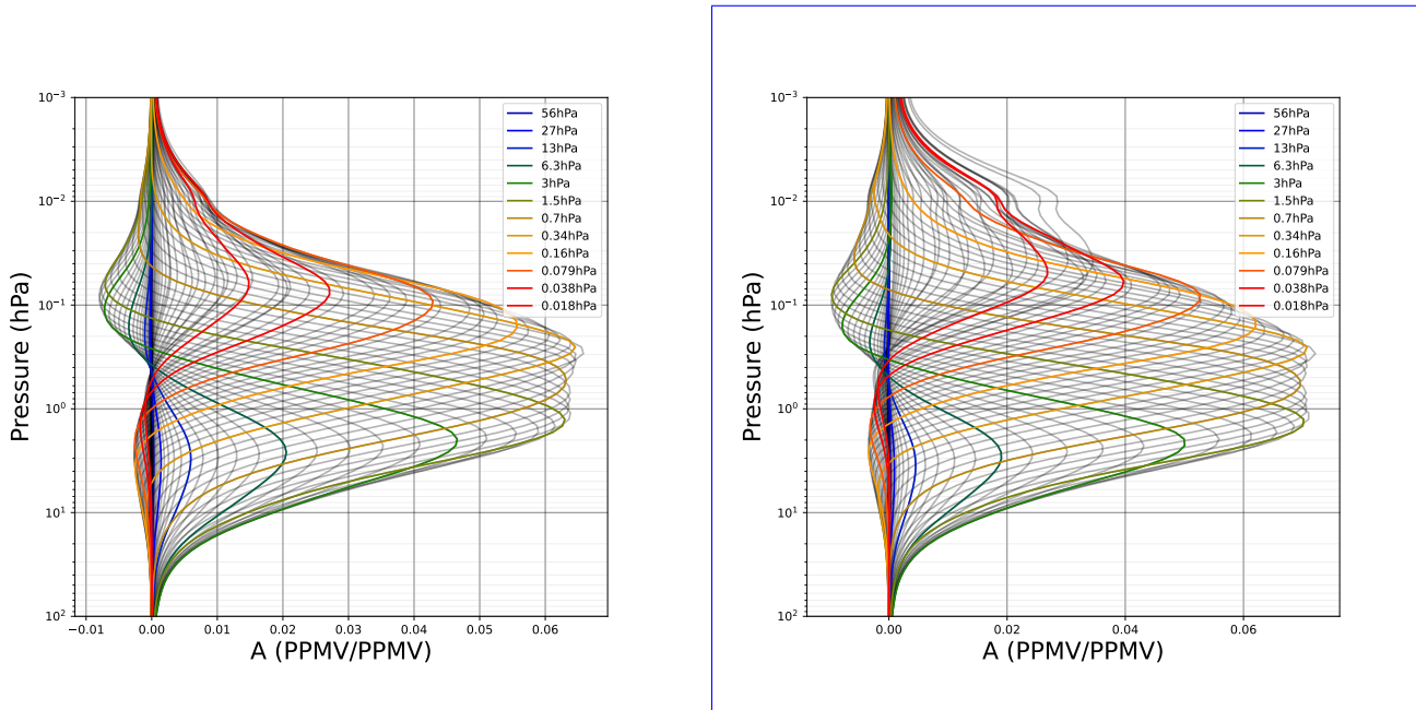
Figure 5. Mean averaging kernel for retrievals made with the AC-240 (left) and USRP (right) spectrometers between November 2022 and October 2023.
