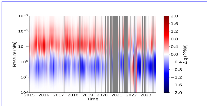
Figure 10. Time series of the difference between MLS water vapour and MIAWARA measurements made with the corrected spectra.
