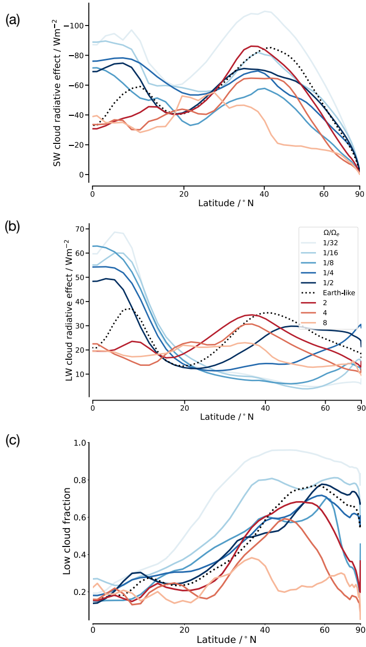
Figure 9. Zonal mean of the (a) shortwave, (b) longwave cloud radiative effect, and (c) low cloud fraction for different rotation rates.
