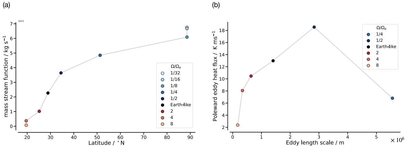
Figure 2. (a) Latitudinal extent vs. strength of the Hadley cell, based on the mass stream function at different rotation rates. (b) Eddy length scale vs. Eddy heat flux at different rotation rates.
