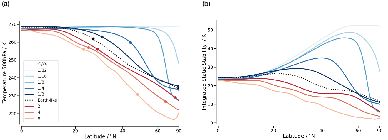
Figure 3. Zonal mean (a) temperature at 500 hPa and (b) integrated static stability from 1000 to 400 hPa for different rotation rates. The dots in (a) mark the outermost edges of the baroclinic zone.
