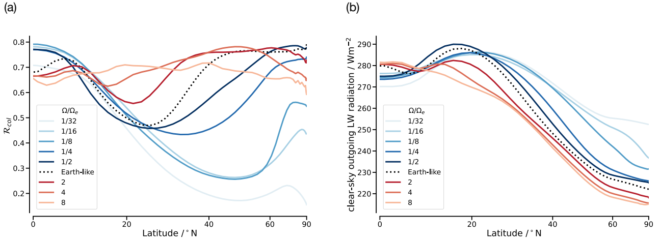
Figure 6. Zonal mean of (a) column relative humidity \mathcal{R}_{col} and (b) clear-sky outgoing longwave radiation for different rotation rates.
