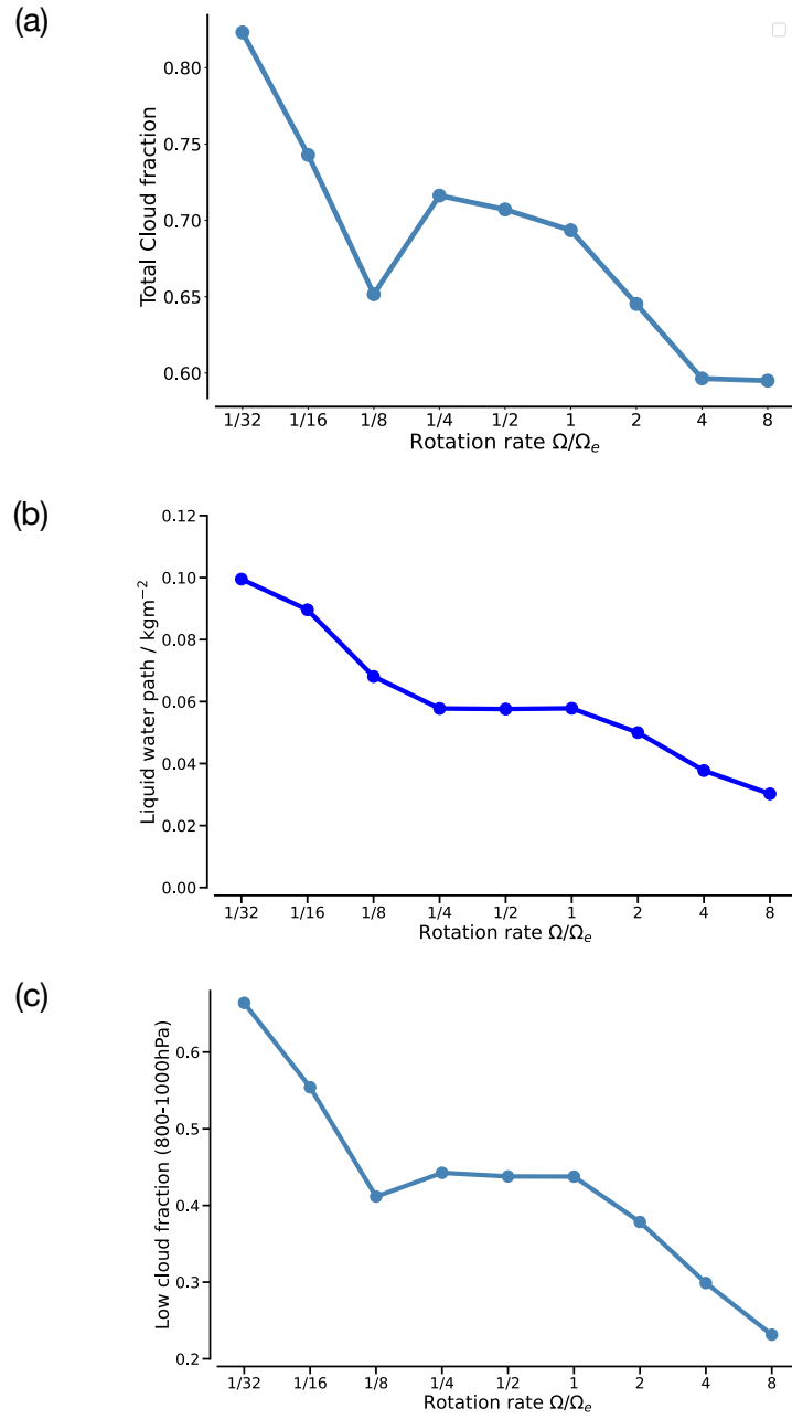
Figure 10. Global mean of (a) total cloud fraction, (b) liquid water path, and (c) total low cloud fraction for different rotation rates
