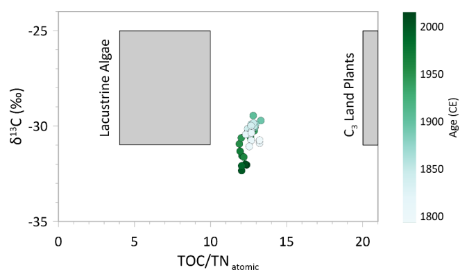
Figure 7. C/N– \delta^{13}\text{C} –plot showing sediment samples of the short core EN18232-1. In general, lacustrine algae have a C/N ratio between 4 to 10, \text{C}_3 land plants have a ratio > 20 (Meyers and Teranes, 2001). Figure is based on the values given by Meyers and Teranes (2001).
