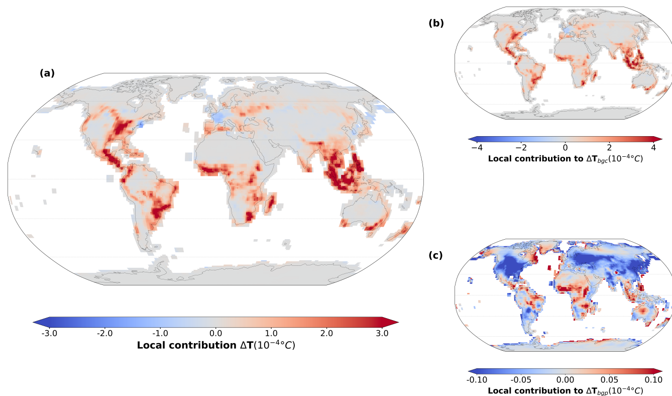
Figure 6. (a) Combined biogeochemical (BGC) and biogeophysical (BGP) contribution to global temperature change computed from the sum of the local BGC (6b) and BGP (6c) contribution computed using Equations (6) and (7) respectively, (b): local BGC contribution of each grid cell to global temperature change computed across 11 Earth system models (ESMs) as the product of the mean grid cell land-use emissions over 30 years (1985–2014) and the model-specific TCRE value, and (c) local BGP contribution of each grid cell to global temperature change computed across 13 ESMs, as the product of the mean grid cell temperature over 30 years (1985–2014) and the grid cell weighted area. Both BGC and BGP contributions are computed from the difference between the historical and hist-noLu simulation. Panels (b): and (c) are identical to Figs. S8a and S9a, respectively and have been reproduced here for the purpose of comparison. The ocean surface is masked out in panel (c) to isolate the local contribution resulting only from land surfaces. Refer to Fig. S9a for the full local BGP contribution including over ocean surfaces.
