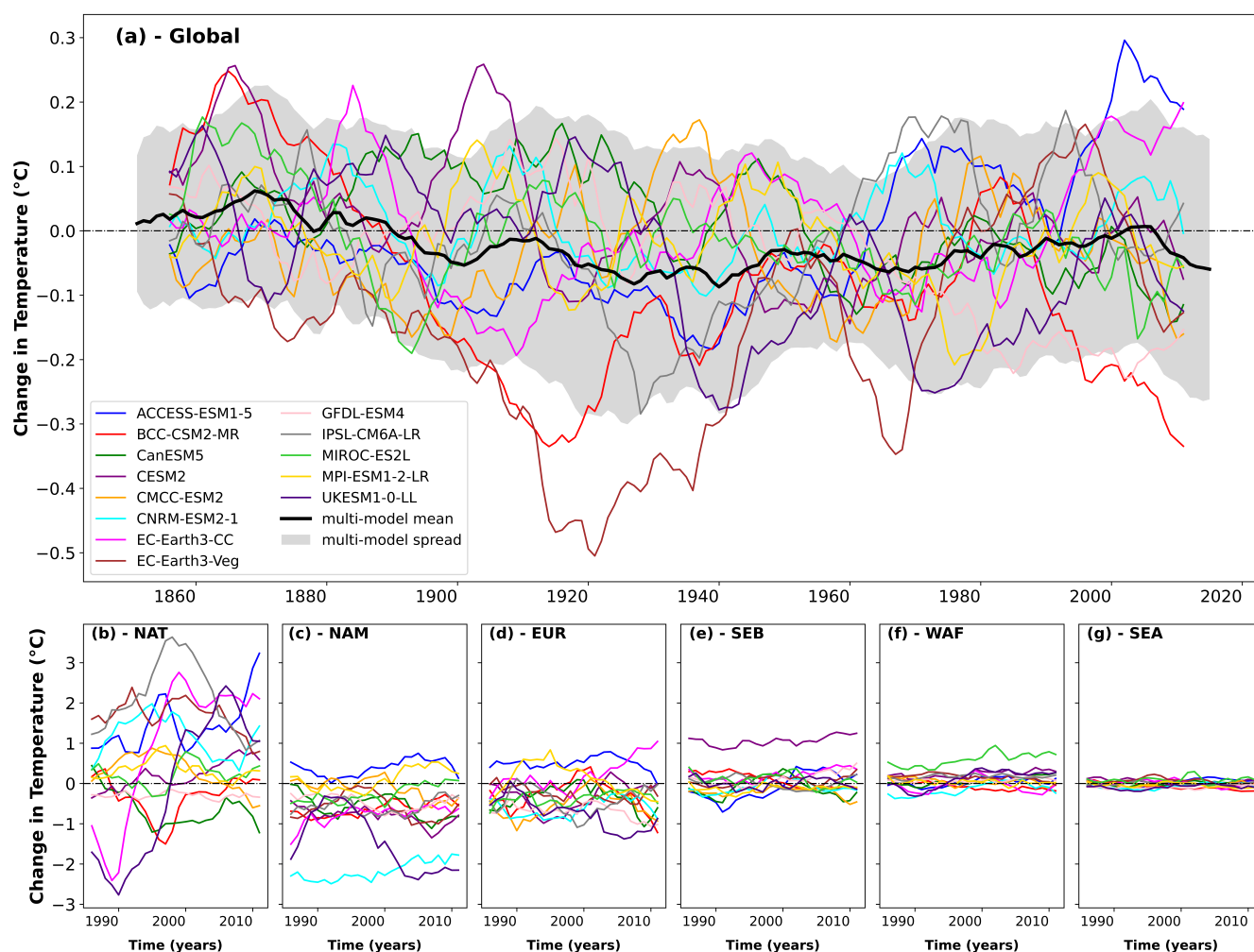
Figure 5. Time series of the global (a) and regional (b) - (g) response of near-surface air temperature due to biogeophysical effects of LUC ( \Delta T_{bgp} ) across 13 Earth System Models (ESMs). Results are computed as the difference between the historical and hist-noLu simulation from 1850–2014 for the global estimate in panel (a) and 1985–2014 for the regional estimates in panels (b) - (g). A 10-year running average is applied across both global and regional estimates. The thick black line and the grey shaded area in (a) represent the ensemble mean estimate and the standard deviation, respectively across all ESMs. The dash-dotted line represents the zero line. The acronyms are NATL = North Atlantic, NAM = North America, EURA = Eurasia, SEB = South East Brazil, WAFR = West Africa, SEA = Southeast Asia. Refer to Fig. 4a for the spatial extents used in computing panels (b) - (g).
