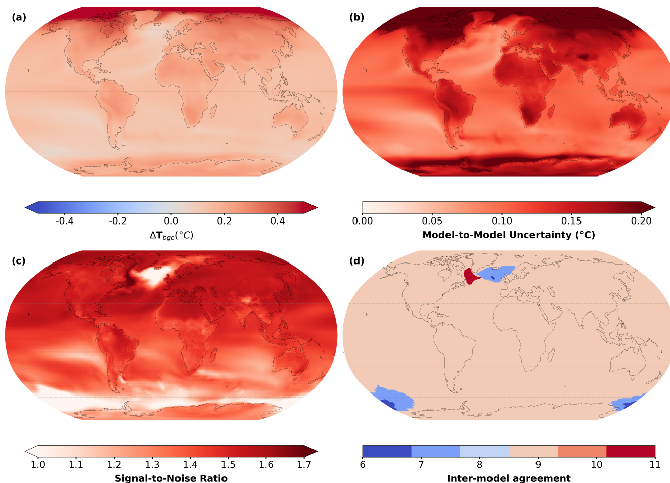
Figure 3. Estimated temperature response to cumulative LUC emissions as ( \Delta T_{bgc} ) (a) the multi-model mean, and (b) the inter-model spread, computed as the standard deviation, showing the uncertainty in estimates over each grid cell. The signal-to-noise ratio (c) indicates the strength of the signal as compared to the inter-model uncertainty. It measures the relative weight of the multi-model mean anomalies in (a) with respect to the model coherence in (b) where a high absolute number means a robust signal. And finally, (d) the inter-model agreement shows the sum of the sign of \Delta T_{bgc} (-1 or +1) across all models (direction, rather than magnitude) for each grid cell (blues: negative/decreasing; reds: positive/increasing). Results computed across 11 Earth system models, as the temperature response due to the cumulative land \text{CO}_2 fluxes at the end of the simulation (year 2014) for each model from the difference between the historical and hist-noLu simulation.
