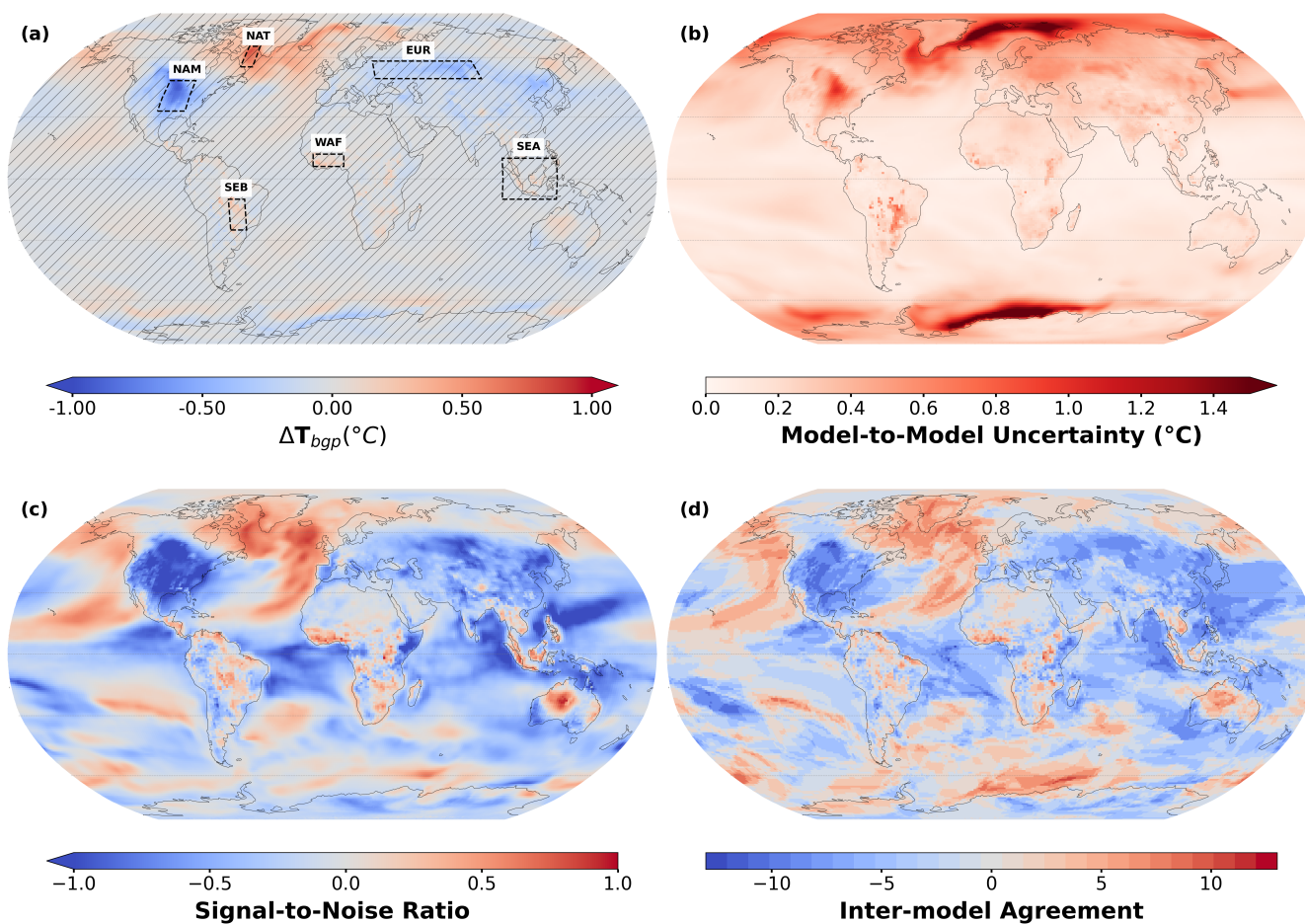
Figure 4. Response of near-surface air temperature due to biogeophysical effects of LUC ( \Delta T_{bgp} ) across 13 Earth System Models (ESMs): (a) the multi-model mean, indicating the average temperature response (stippling indicates regions not statistically significant at the 5% level; the dashed boxes show the spatial extents of the regions considered in Fig. 5) (b) the inter-model spread, computed as the standard deviation across models, shows the uncertainty in estimates over each grid cell. The signal-to-noise ratio (c) indicates the strength of the signal as compared to the inter-model uncertainty. It measures the relative weight of the multi-model mean anomalies in (a) with respect to the model coherence in (b) where a high absolute number means a robust signal. And finally, (d) the inter-model agreement shows the sum of the sign of \Delta T_{bgp} (-1 or +1) across all models (direction, rather than magnitude) for each grid cell (blues: negative/decreasing; reds: positive/increasing). Results are computed as the difference between the historical and hist-noLu simulations in 1985–2014.
