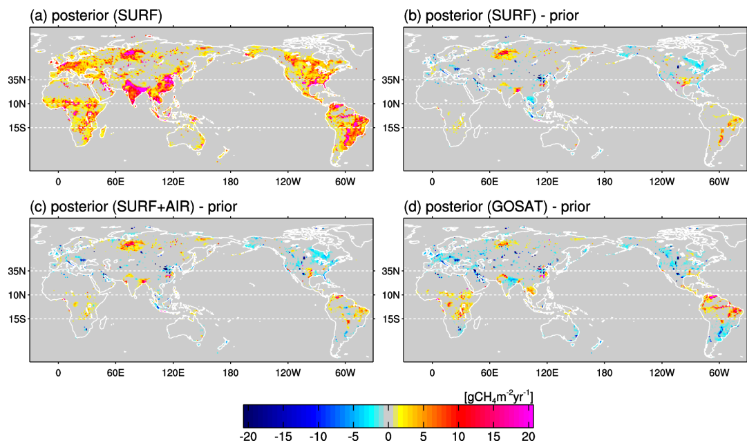
380 Figure 3 Spatial pattern of posterior total net CH 4 emissions by the SURF inversion averaged for 2016–2019 (a) and the (posterior – prior) difference pattern (b). Also shown are the other (posterior – prior) emissions patterns for the SURF+AIR (c) and GOSAT (d) inversions.
