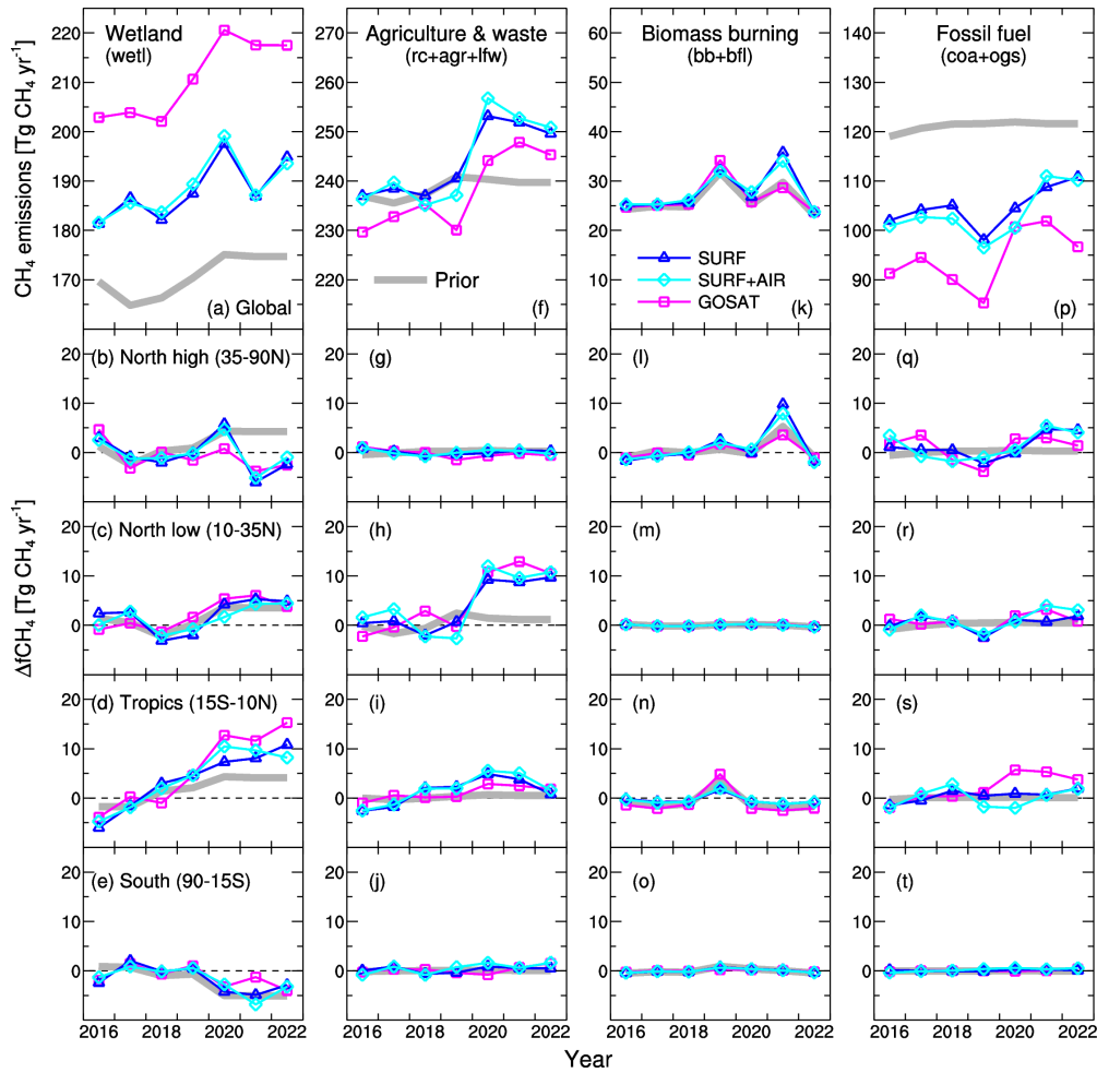
Figure 9 Same as Fig. 5, but separated for sectoral emissions from wetland (wetl) (a–e), agriculture & waste (rc+agr+lfw) (f–j), biomass burning (bb+bff) (k–o), and fossil fuels (coa+ogs) (p–t). Sectoral emissions are merged as shown in Table 1.
