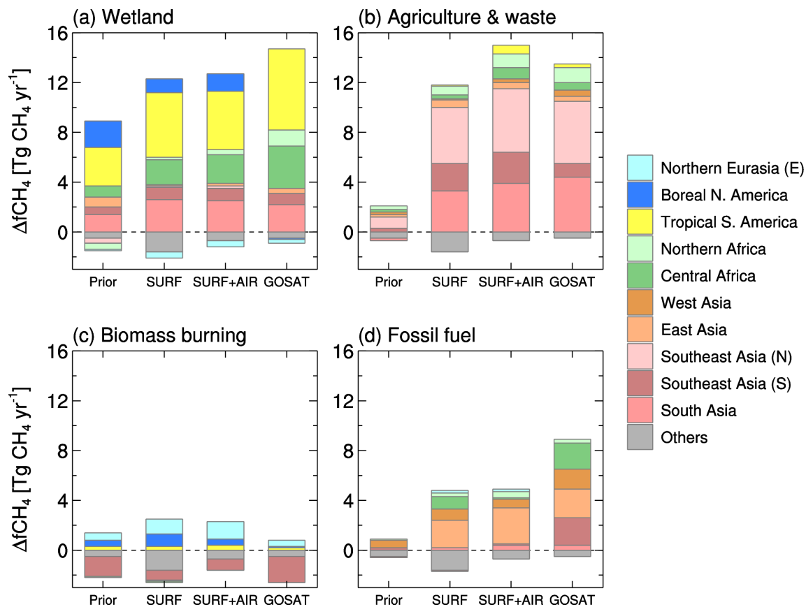
Figure 10 Same as Fig. 7, but separated for sectoral emissions from wetland (wetl) (a), agriculture & waste (rc+agr+lfw) (b), biomass burning (bb+bf) (c), and fossil fuels (coa+ogs) (d). Sectoral emissions are merged as shown in Table 1.
