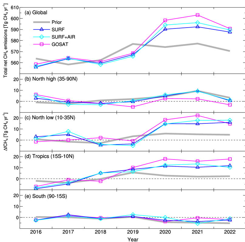
Figure 5 Year-to-year variations of total net \text{CH}_4 emissions integrated globally (a) and those of \Delta f\text{CH}_4 integrated in each latitudinal band: northern high-latitudes ( 35\text{--}90^\circ\text{N} ) (b), northern low-latitudes ( 10\text{--}35^\circ\text{N} ) (c), tropics ( 15^\circ\text{S}\text{--}10^\circ\text{N} ), and southern latitudes ( 90\text{--}15^\circ\text{S} ) (e).
