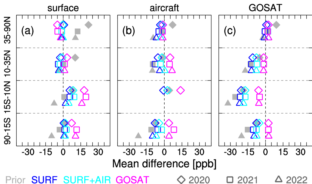
710 Figure B1 Mean differences between observations and prior or posterior mole fractions of atmospheric CH 4 in northern high-latitudes (35–90°N), northern low-latitudes (10–35°N), tropics (15°S–10°N), and southern latitudes (90–15°S) for 2020 (diamond), 2021 (square), and 2022 (triangle). The mean differences are calculated for different observational types of surface (a) and aircraft (b) flask observations, and for the GOSAT data (c). The prior and posterior mole fractions are derived from atmospheric simulations of NICAM-TM with the prior (gray) and posterior fluxes: SURF (blue), SURF+AIR (cyan), and GOSAT (magenta), respectively.
