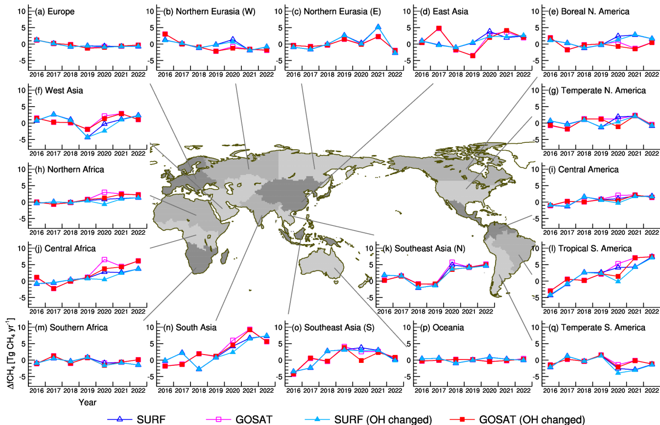
740 Figure C1 Same as Fig. 6, but including the sensitivity tests with OH reduced in 2020 for the surface (light blue closed triangles) and GOSAT (red closed squares) inversions.
