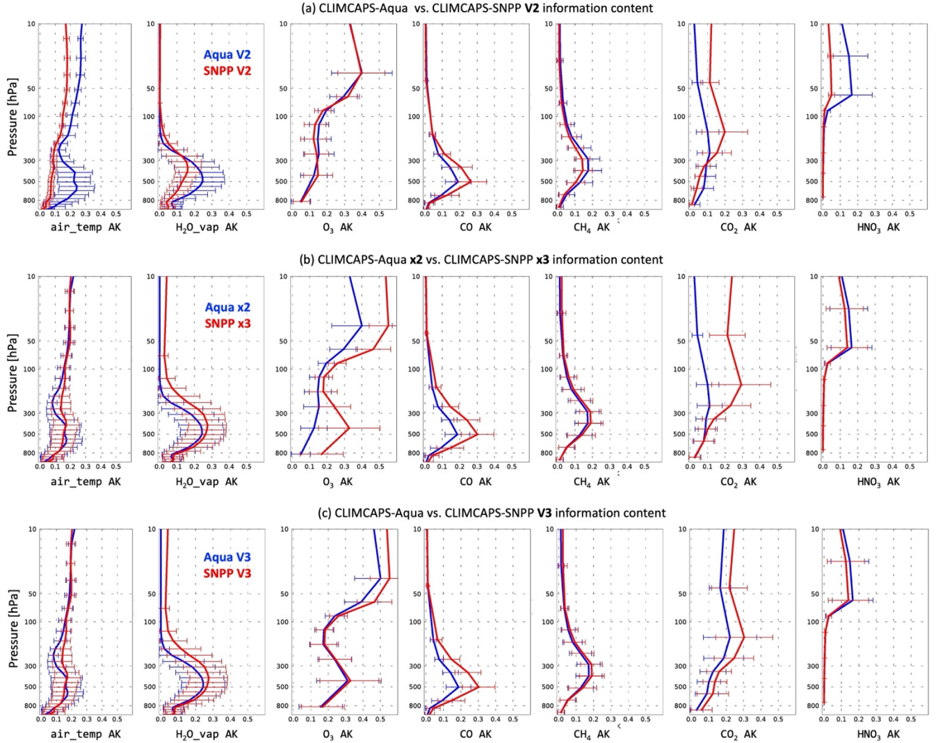
505 Figure 8: CLIMCAPS AKs for [air_temp] as well as six atmospheric gases, [h2o_vap], O 3 , CO, CH 4 , CO 2 and HNO 3 , as the mean and standard deviation (error bars) for all retrievals in ascending and descending orbits that passed quality control on 1 September 2016. A comparison of CLIMCAPS AKs from (blue) Aqua and (red) SNPP using three different configurations, (a) V2, (b) experimental SNPP-x3 and Aqua-x2, as well as the proposed (c) V3 for both instrument suites.
