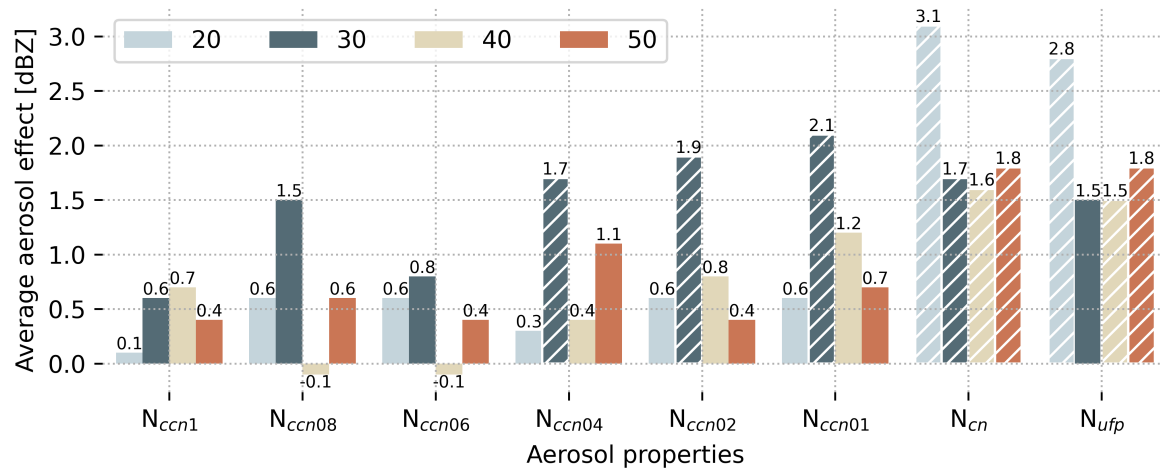
Figure 10. Same as Figure 7a but using maximum reflectivity as outcome dependent variable and CAPE as confounding variable.
