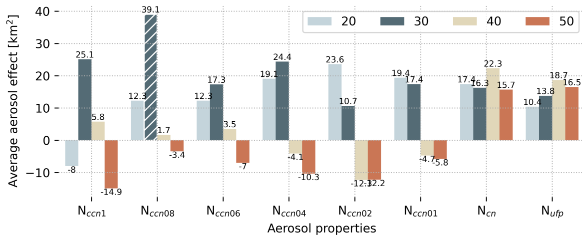
Figure 9. Same as Figure 7a but for cell area as outcome dependent variable and CAPE as confounding variable.
