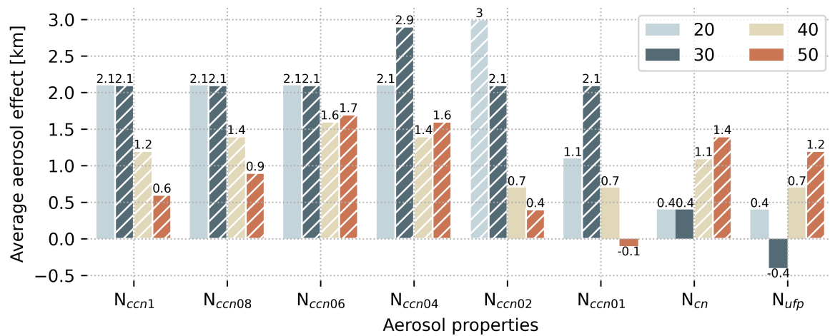
Figure 8. Average causal aerosol effects on 30-dBZ ETH estimated for each potential exposure variable after controlling for confounders ( ELR_3 and CAPE) for DCCs identified during sea-breeze days only. The post-sounding aerosol averaging period is considered. Different colors represent different maximum distances between measurements of environments and DCCs. The meteorological variables are calculated using ARM soundings (6-hr) when assuming the most-unstable parcel would rise to form a convection. The white hatch lines indicate "valid" results.
