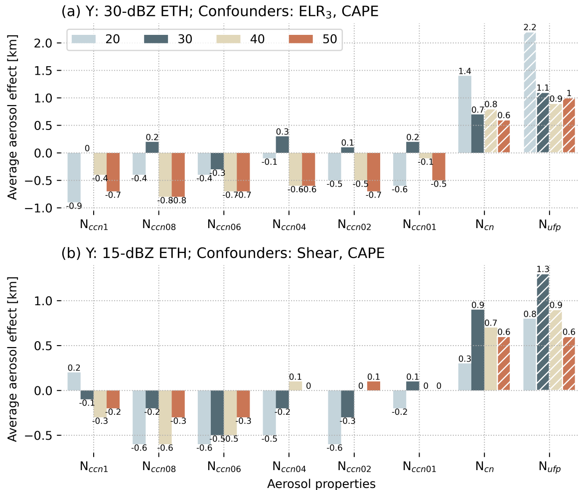
Figure 7. Average causal -aerosol effects on (a) 30-dBZ ETH and (b) 15-dBZ ETH estimated for each potential exposure variable after controlling for confounders . Different colors represent different maximum distances between measurements of environmental variables and DCC properties. The meteorological variables are calculated using ARM soundings (6-hr) when assuming the most-unstable parcel would rise to form a convection. The white hatch lines indicate "valid" results.
