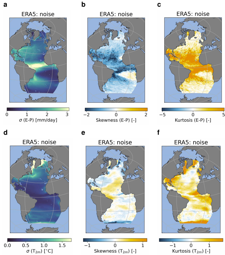
Figure 1. Standard deviation ( \sigma ), skewness and excess kurtosis over time for the ERA5 noise for the E – P flux (a-c) and T_{2m} (d-f).
