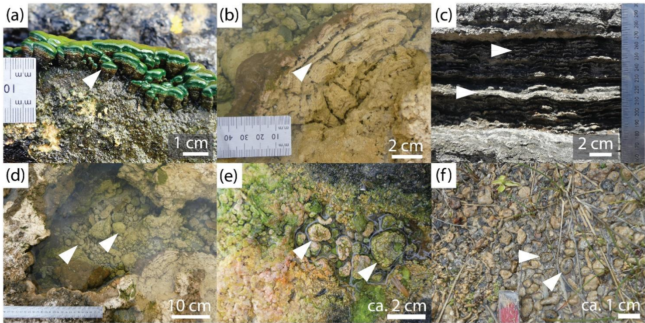
655 Figure 8. Rock coast microbialite internal organisation (mesostructure): (a) stromatolitic columns coalescing to form colloform mat topography (Bundoran, Ireland); (b) stromatolitic (laminar) internal organisation of a colloform stromatolite (Lauries Bay, South Africa); (c) stromatolite (laminar) barrage (Quarry Bay, Western Australia); (d) barrage pool associated oncoids; (e) fluvial crust with small oncoids and proto-oncoids (Sligo Bay, Ireland); (f) vegetation-associated oncoids (Islay, Scotland).
