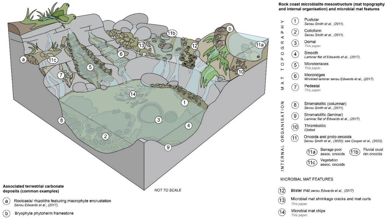
Figure 6. Block diagram of rock coast microbialite mesostructures including mat topography (surface morphology), internal organisation, and microbial mat features; and common associated features of terrestrial carbonate deposits.
