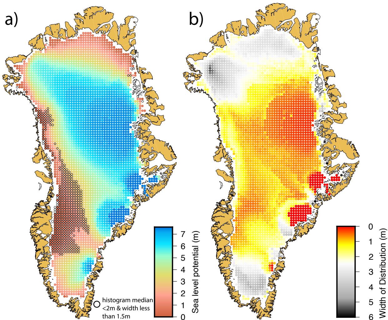
320 Figure 3. Greenland's sea level potential. a) Colors indicate sea level potential, defined as the median amount that Greenland has contributed to global sea level when that grid cell has become ice-free. Black outline highlights regions where ice-free conditions are associated with median sea-level potential less than 2 meters, and the spread is less than 1.5 meters. Dots are plotted for areas where the ice thickness is greater than 600 meters and sea level potential is greater than zero within a 20 by 20 kilometer area; areas within the modern limit of the ice sheet (underlying white area) that do not meet these criteria are not plotted. b) Width of the ensemble spread for each location (meters sea level equivalent).
