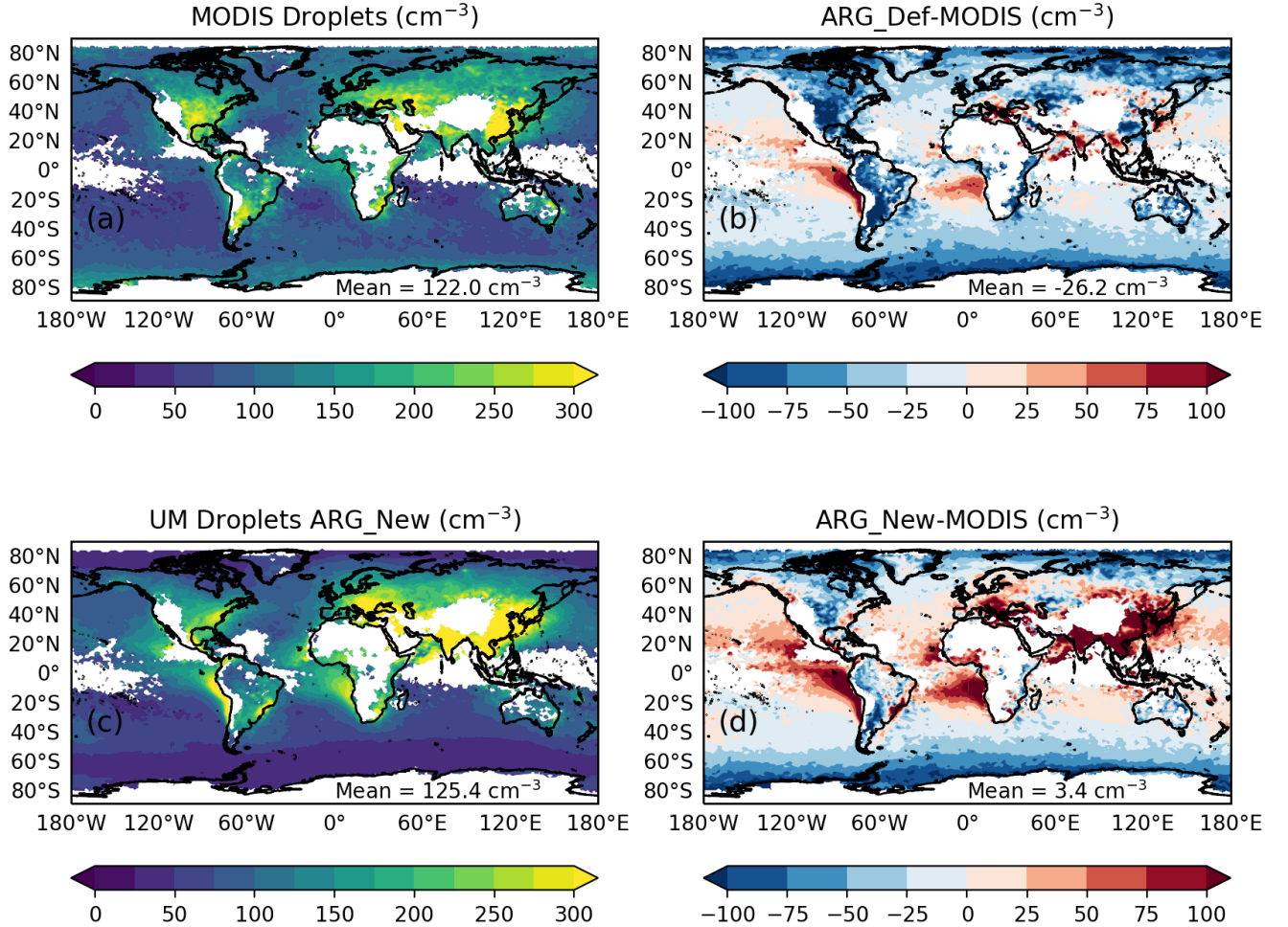
Figure 3. (a) Annual average of daytime top of cloud droplet number concentrations from MODerate Imaging Spectroradiometer (MODIS) satellite data (Grosvenor et al., 2018) regridded to the N96 UM grid. (b) Bias in the UM simulation with default ARG (ARG_Def). (c) Annual average of daytime top-of-cloud droplet number concentrations from UM simulation with updated ARG (ARG_New). (d): Bias in UM simulation with updated ARG.
