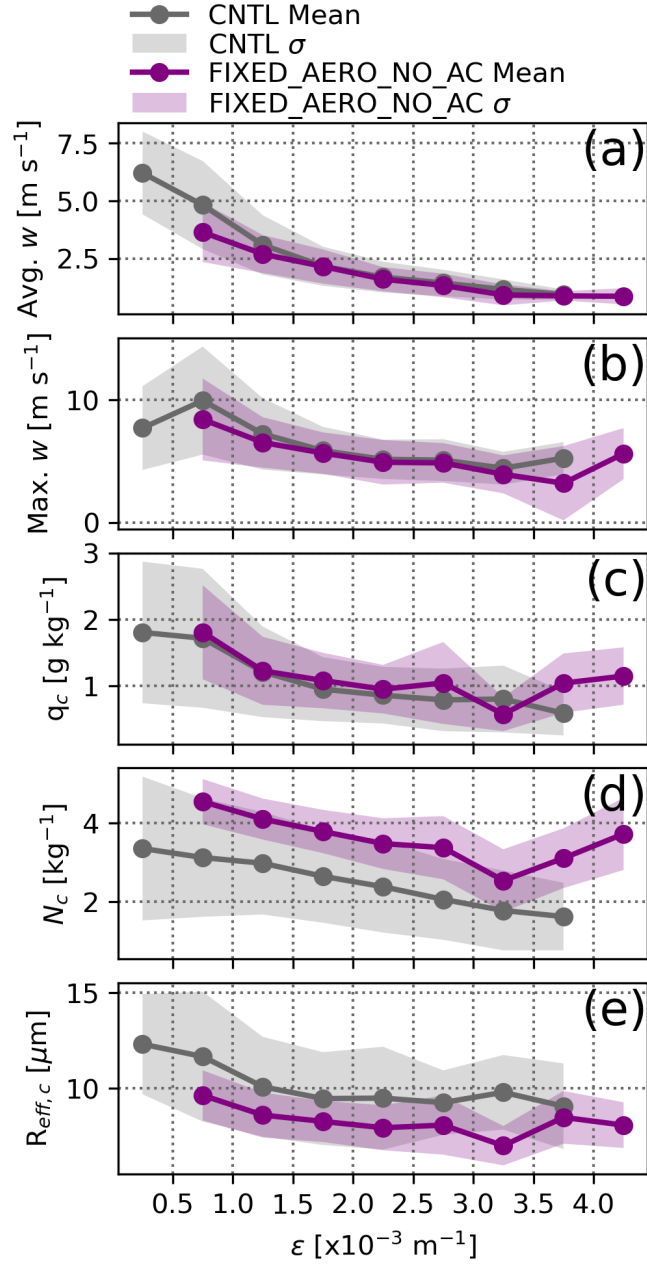
Figure 14. Thermal average properties as a function of fractional entrainment rate ( \varepsilon ). \varepsilon bin widths are 0.5 \times 10^{-3} \text{ m}^{-1} . Shaded regions show the standard deviation from the mean and at least 5 thermals are required for a given \varepsilon bin.
